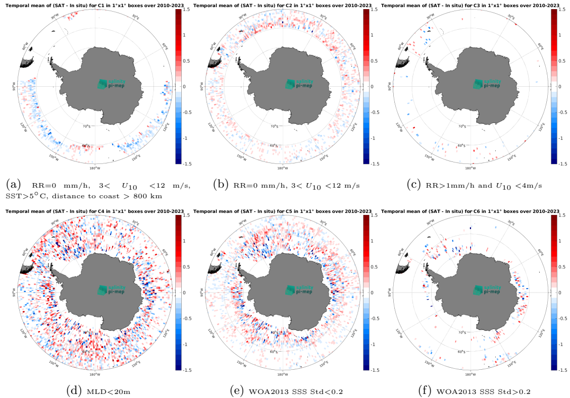
Figure 12: Temporal mean gridded over spatial boxes of size 1^{\circ}\times 1^{\circ} of \Delta\text{SSS} (SMOS SSS L3 v9 - 9 Days (CATDS-CEC-LOCEAN) - Argo) for 6 different subdatasets corresponding to:RR=0 mm/h, 3 < U_{10} < 12 m/s, SST > 5^{\circ}\text{C} , distance to coast > 800 km (a), RR=0 mm/h, 3 < U_{10} < 12 m/s (b), RR > 1\text{mm/h} and U_{10} < 4\text{m/s} (c),MLD < 20\text{m} (d),WOA2013 SSS Std < 0.2 (e),WOA2013 SSS Std > 0.2 (f).
