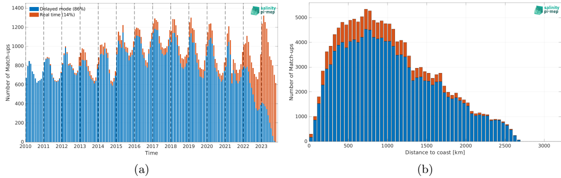
Figure 1: Number of match-ups between Argo and SMOS SSS L3 v9 - 9 Days (CATDS-CEC-LOCEAN) SSS as a function of time (a) and as function of the distance to coast (b) over the Southern Ocean Pi-MEP region and for the full satellite product period.
