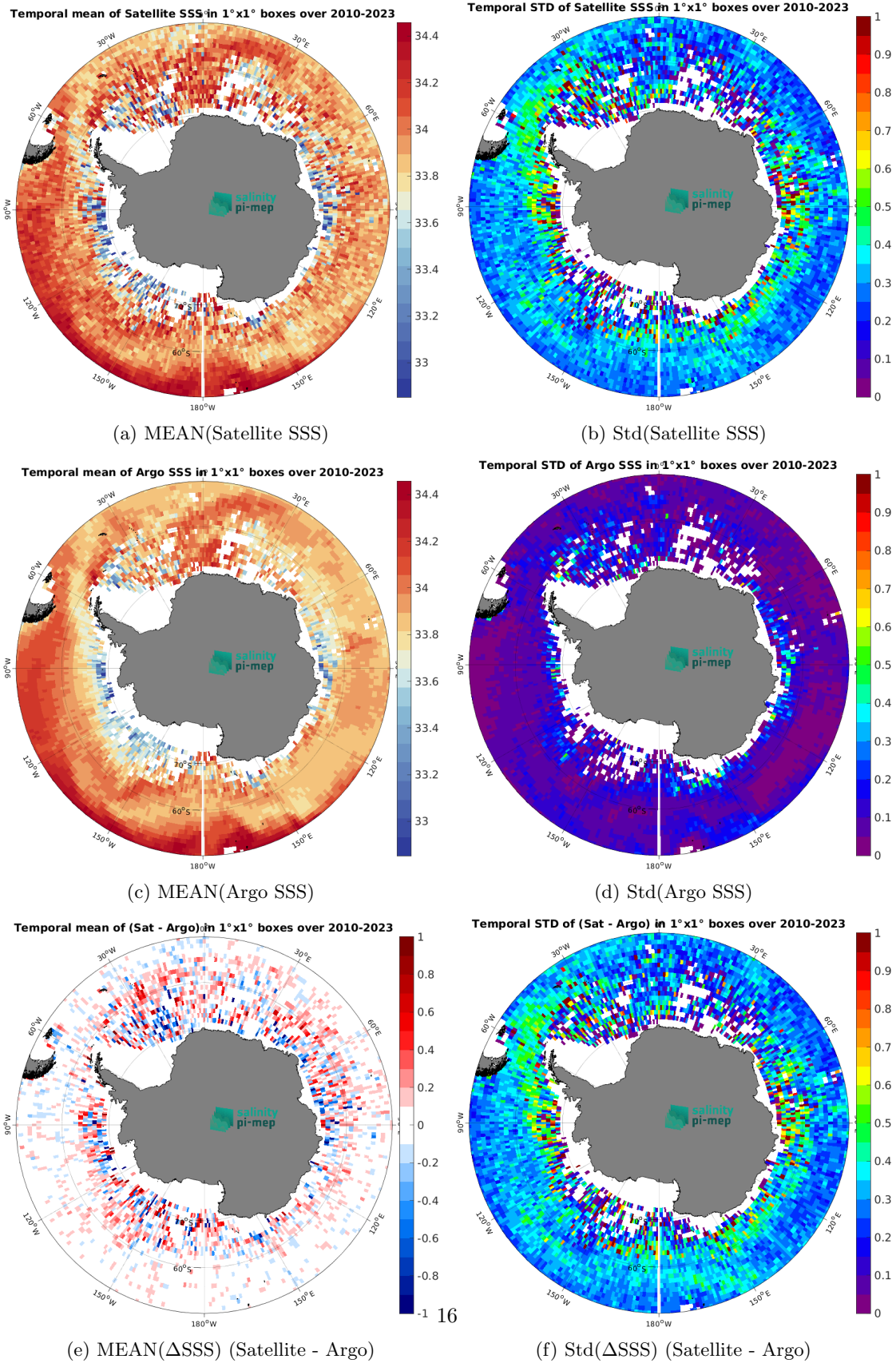
Figure 6: Temporal mean (left) and Std (right) of SSS from SMOS SSS L3 v9 - 9 Days (CATDS-CEC-LOCEAN) (top), Argo (middle), and of \Delta SSS (Satellite - Argo). Only match-up pairs are used to generate these maps.
