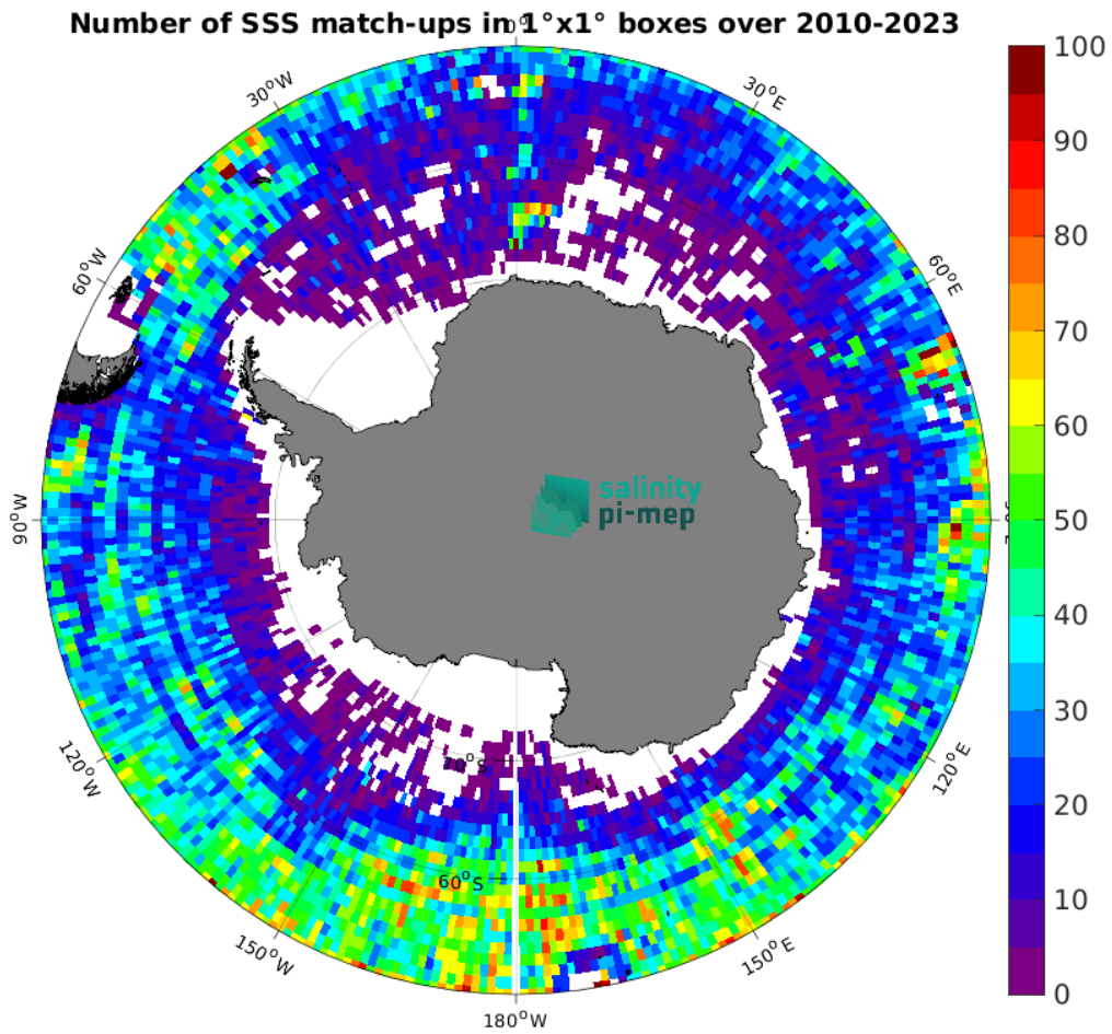
Figure 4: Number of SSS match-ups between Argo SSS and the SMOS SSS L3 v9 - 9 Days (CATDS-CEC-LOCEAN) SSS product for the Southern Ocean Pi-MEP region over 1^\circ \times 1^\circ boxes and for the full satellite product period.
