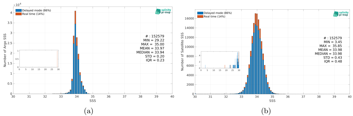
Figure 2: Histograms of SSS from Argo (a) and SMOS SSS L3 v9 - 9 Days (CATDS-CEC-LOCEAN) (b) considering all match-up pairs per bins of 0.1 over the Southern Ocean Pi-MEP region and for the full satellite product period.
