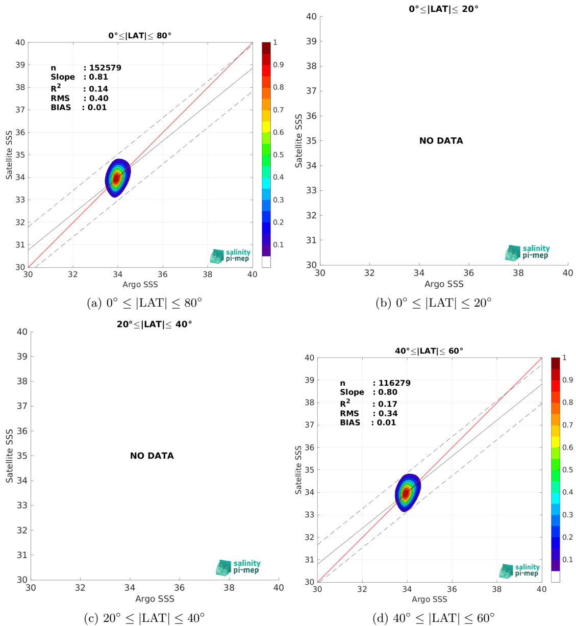
Figure 9: Contour maps of the concentration of SMOS SSS L3 v9 - 9 Days (CATDS-CEC-LOCEAN) SSS (y-axis) versus Argo SSS (x-axis) at match-up pairs for different latitude bands. For each plot, the red line shows x=y . The black thin and dashed lines indicate a linear fit through the data cloud and the \pm 95\% confidence levels, respectively. The number match-up pairs n , the slope and R^2 coefficient of the linear fit, the root mean square (RMS) and the mean bias between satellite and in situ data are indicated for each latitude band in each plots.
