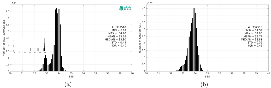
Figure 2: Histograms of SSS from TSG (SAMOS) (a) and SMOS SSS L3 v9 - 18 Days (CATDS-CEC-LOCEAN) (b) considering all match-up pairs per bins of 0.1 over the Southern Ocean Pi-MEP region and for the full satellite product period.
