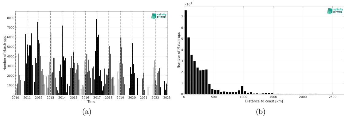
Figure 1: Number of match-ups between TSG (SAMOS) and SMOS SSS L3 v9 - 18 Days (CATDS-CEC-LOCEAN) SSS as a function of time (a) and as function of the distance to coast (b) over the Southern Ocean Pi-MEP region and for the full satellite product period.
