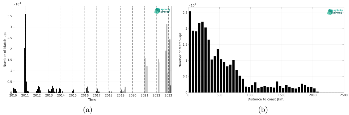
Figure 2: Number of match-ups between TSG (Polarstern) and SMOS SSS L3 v9 - 18 Days (CATDS-CEC-LOCEAN) SSS as a function of time (a) and as function of the distance to coast (b) over the Southern Ocean Pi-MEP region and for the full satellite product period.
