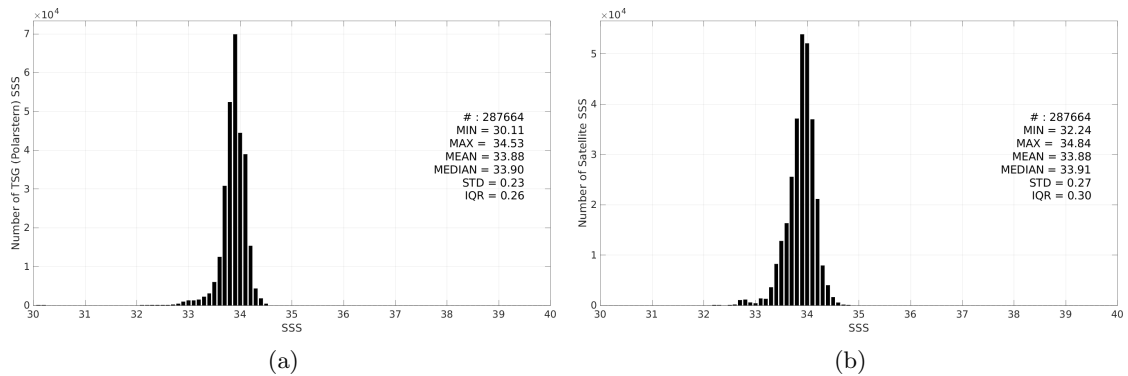
Figure 3: Histograms of SSS from TSG (Polarstern) (a) and SMOS SSS L3 v9 - 18 Days (CATDS-CEC-LOCEAN) (b) considering all match-up pairs per bins of 0.1 over the Southern Ocean Pi-MEP region and for the full satellite product period.
