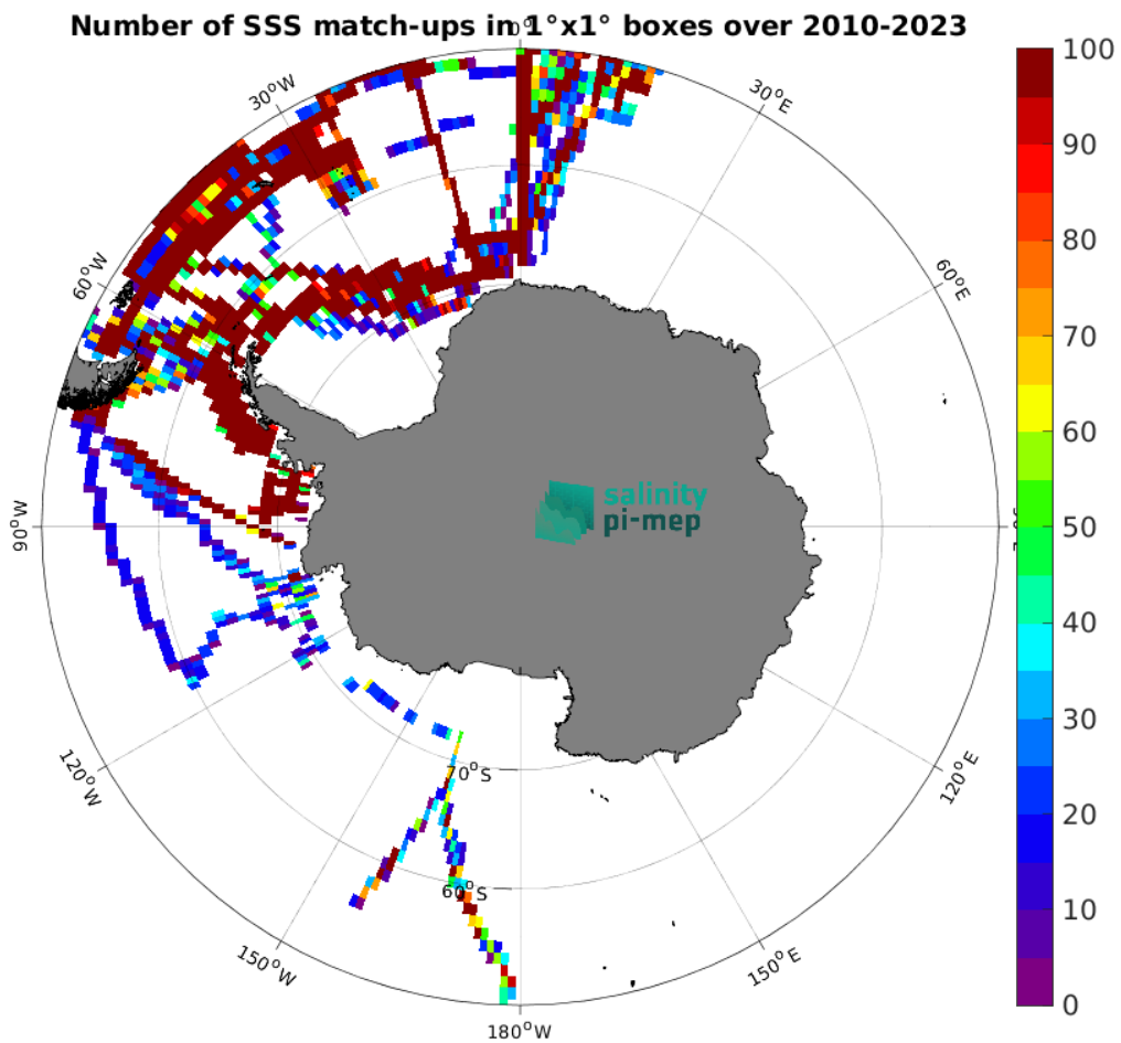
Figure 5: Number of SSS match-ups between TSG (Polarstern) SSS and the SMOS SSS L3 v9 - 18 Days (CATDS-CEC-LOCEAN) SSS product for the Southern Ocean Pi-MEP region over 1^\circ \times 1^\circ boxes and for the full satellite product period.
