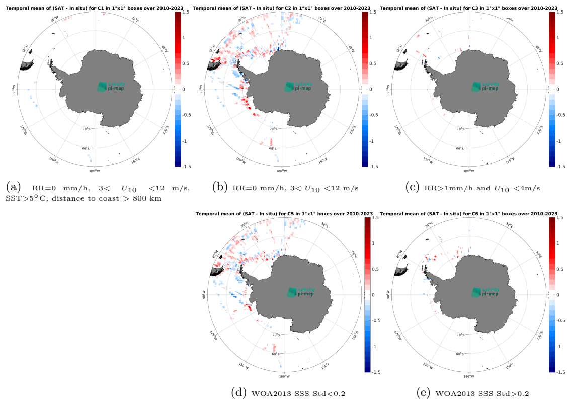
Figure 14: Temporal mean gridded over spatial boxes of size 1^\circ \times 1^\circ of \Delta\text{SSS} (SMOS SSS L3 v9 - 18 Days (CATDS-CEC-LOCEAN) - TSG (Polarstern)) for 5 different subdatasets corresponding to:RR=0 mm/h, 3 < U_{10} < 12 m/s, SST>5°C, distance to coast > 800 km (a), RR=0 mm/h, 3 < U_{10} < 12 m/s (b), RR>1mm/h and U_{10} < 4 m/s (c), WOA2013 SSS Std<0.2 (d), WOA2013 SSS Std>0.2 (e).
