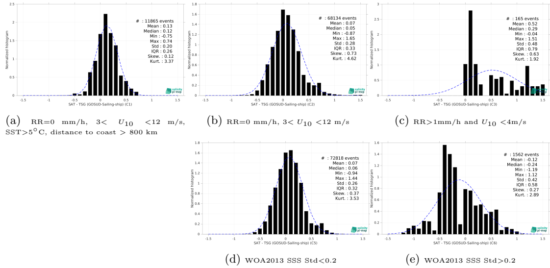
Figure 15: Normalized histogram of \Delta\text{SSS} (SMOS SSS L3 v9 - 18 Days (CATDS-CEC-LOCEAN) - TSG (GOSUD-Sailing-ship)) for 5 different subdatasets corresponding to: RR=0 mm/h, 3 < U_{10} < 12 m/s, SST>5°C, distance to coast > 800 km (a), RR=0 mm/h, 3 < U_{10} < 12 m/s (b), RR>1mm/h and U_{10} < 4 m/s (c), WOA2013 SSS Std<0.2 (d), WOA2013 SSS Std>0.2 (e).
