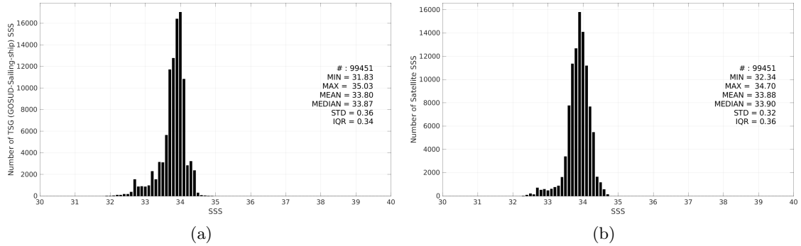
Figure 3: Histograms of SSS from TSG (GOSUD-Sailing-ship) (a) and SMOS SSS L3 v9 - 18 Days (CATDS-CEC-LOCEAN) (b) considering all match-up pairs per bins of 0.1 over the Southern Ocean Pi-MEP region and for the full satellite product period.
