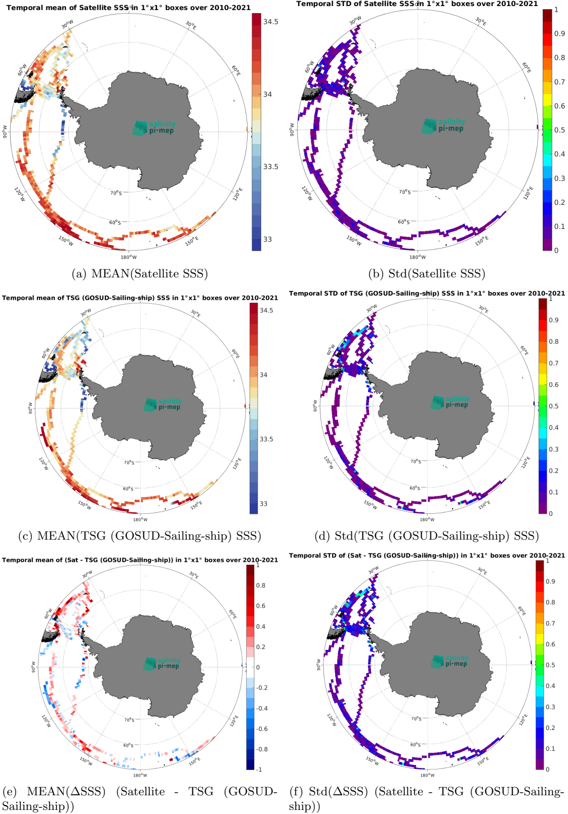
Figure 7: Temporal mean (left) and Std (right) of SSS from SMOS SSS L3 v9 - 18 Days (CATDS-CEC-LOCEAN) (top), TSG (GOSUD-Sailing-ship) (middle), and of \Delta SSS (Satellite - TSG (GOSUD-Sailing-ship)). Only match-up pairs are used to generate these maps.
