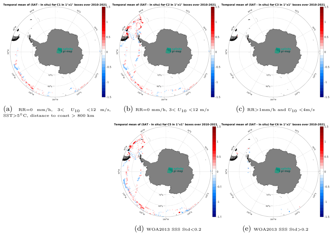
Figure 14: Temporal mean gridded over spatial boxes of size 1^\circ \times 1^\circ of \Delta\text{SSS} (SMOS SSS L3 v9 - 18 Days (CATDS-CEC-LOCEAN) - TSG (GOSUD-Sailing-ship)) for 5 different subdatasets corresponding to:RR=0 mm/h, 3 < U_{10} < 12 m/s, SST>5°C, distance to coast > 800 km (a), RR=0 mm/h, 3 < U_{10} < 12 m/s (b), RR>1mm/h and U_{10} < 4 m/s (c), WOA2013 SSS Std<0.2 (d), WOA2013 SSS Std>0.2 (e).
