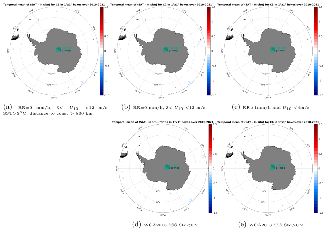
Figure 14: Temporal mean gridded over spatial boxes of size 1^\circ \times 1^\circ of \Delta\text{SSS} (SMOS SSS L3 v9 - 18 Days (CATDS-CEC-LOCEAN) - TSG (GOSUD-Research-vessel)) for 5 different subdatasets corresponding to:RR=0 mm/h, 3 < U_{10} < 12 m/s, SST>5°C, distance to coast > 800 km (a), RR=0 mm/h, 3 < U_{10} < 12 m/s (b), RR>1mm/h and U_{10} < 4 m/s (c), WOA2013 SSS Std<0.2 (d), WOA2013 SSS Std>0.2 (e).
