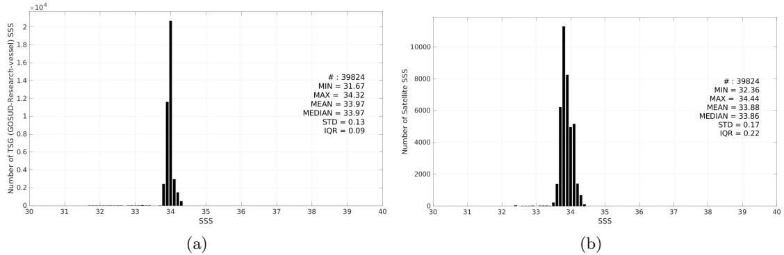
Figure 3: Histograms of SSS from TSG (GOSUD-Research-vessel) (a) and SMOS SSS L3 v9 - 18 Days (CATDS-CEC-LOCEAN) (b) considering all match-up pairs per bins of 0.1 over the Southern Ocean Pi-MEP region and for the full satellite product period.
