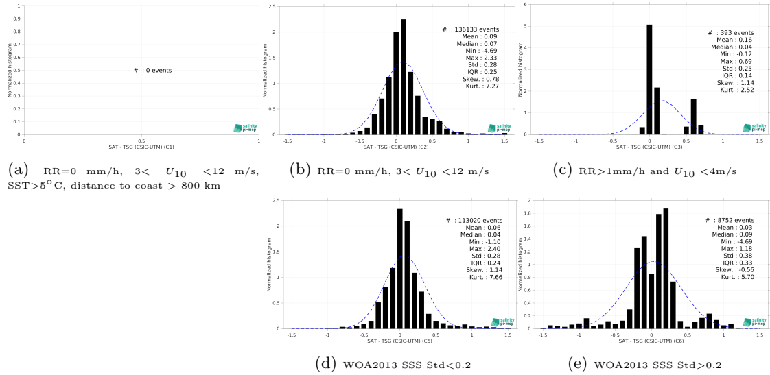
Figure 15: Normalized histogram of \Delta\text{SSS} (SMOS SSS L3 v9 - 18 Days (CATDS-CEC-LOCEAN) - TSG (CSIC-UTM)) for 5 different subdatasets corresponding to: RR=0 mm/h, 3 < U_{10} < 12 m/s, SST > 5^{\circ}\text{C} , distance to coast > 800 km (a), RR=0 mm/h, 3 < U_{10} < 12 m/s (b), RR > 1\text{mm/h} and U_{10} < 4\text{m/s} (c), WOA2013 SSS Std < 0.2 (d), WOA2013 SSS Std > 0.2 (e).
