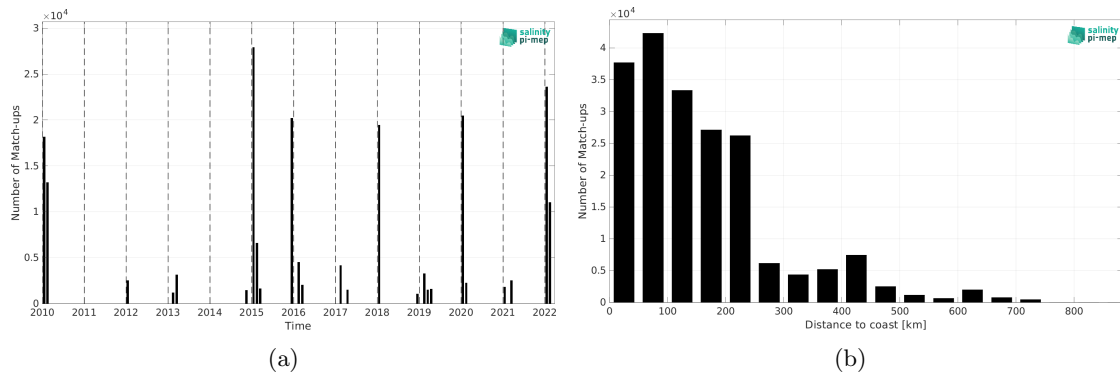
Figure 1: Number of match-ups between TSG (CSIC-UTM) and SMOS SSS L3 v9 - 18 Days (CATDS-CEC-LOCEAN) SSS as a function of time (a) and as function of the distance to coast (b) over the Southern Ocean Pi-MEP region and for the full satellite product period.
