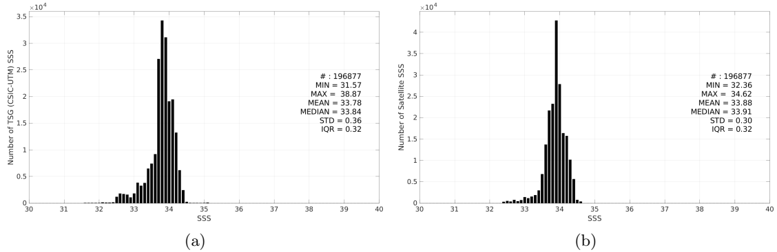
Figure 2: Histograms of SSS from TSG (CSIC-UTM) (a) and SMOS SSS L3 v9 - 18 Days (CATDS-CEC-LOCEAN) (b) considering all match-up pairs per bins of 0.1 over the Southern Ocean Pi-MEP region and for the full satellite product period.
