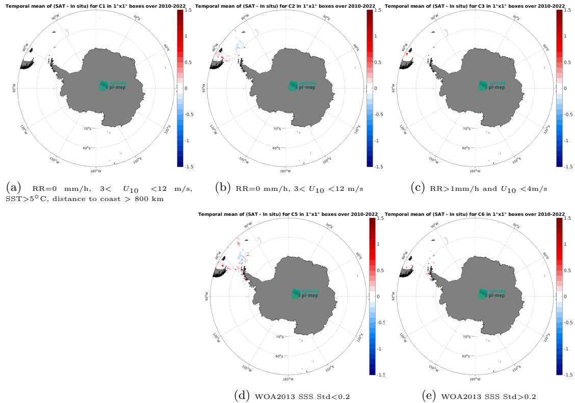
Figure 12: Temporal mean gridded over spatial boxes of size 1^{\circ}\times 1^{\circ} of \Delta\text{SSS} (SMOS SSS L3 v9 - 18 Days (CATDS-CEC-LOCEAN) - TSG (CSIC-UTM)) for 5 different subdatasets corresponding to:RR=0 mm/h, 3 < U_{10} < 12 m/s, SST >5^{\circ}\text{C} , distance to coast > 800 km (a), RR=0 mm/h, 3 < U_{10} < 12 m/s (b), RR >1 mm/h and U_{10} < 4 m/s (c), WOA2013 SSS Std <0.2 (d), WOA2013 SSS Std >0.2 (e).
