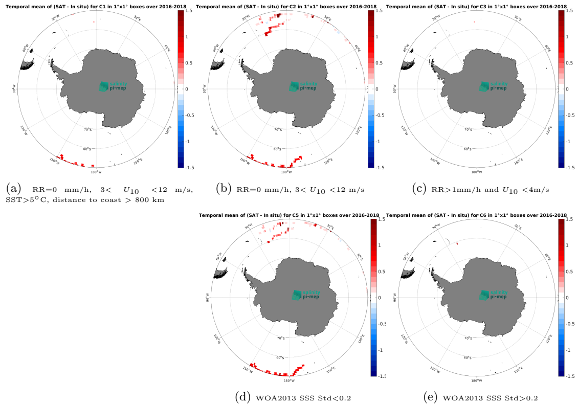
Figure 13: Temporal mean gridded over spatial boxes of size 1^\circ \times 1^\circ of \Delta\text{SSS} (SMOS SSS L3 v9 - 18 Days (CATDS-CEC-LOCEAN) - Surface drifters) for 5 different subdatasets corresponding to:RR=0 mm/h, 3 < U_{10} < 12 m/s, SST >5^\circ\text{C} , distance to coast > 800 km (a), RR=0 mm/h, 3 < U_{10} < 12 m/s (b), RR >1 mm/h and U_{10} < 4 m/s (c), WOA2013 SSS Std <0.2 (d), WOA2013 SSS Std >0.2 (e).
