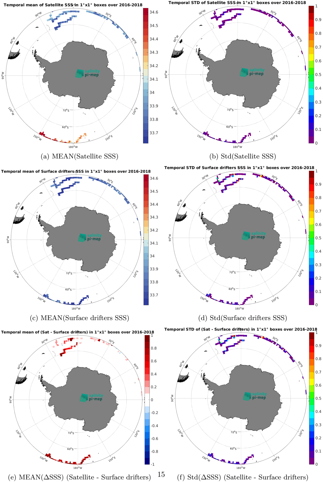
Figure 5: Temporal mean (left) and Std (right) of SSS from SMOS SSS L3 v9 - 18 Days (CATDS-CEC-LOCEAN) (top), Surface drifters (middle), and of \Delta SSS (Satellite - Surface drifters). Only match-up pairs are used to generate these maps.
