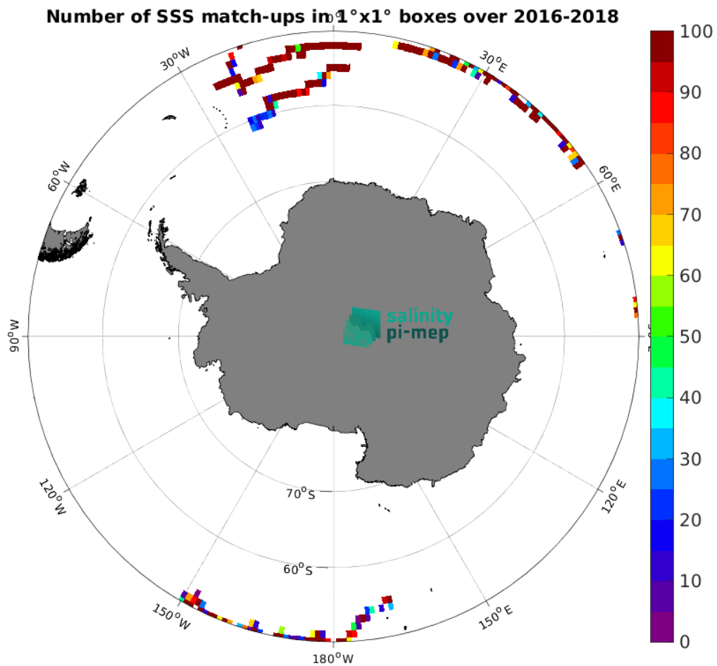
Figure 3: Number of SSS match-ups between Surface drifters SSS and the SMOS SSS L3 v9 - 18 Days (CATDS-CEC-LOCEAN) SSS product for the Southern Ocean Pi-MEP region over 1^\circ \times 1^\circ boxes and for the full satellite product period.
