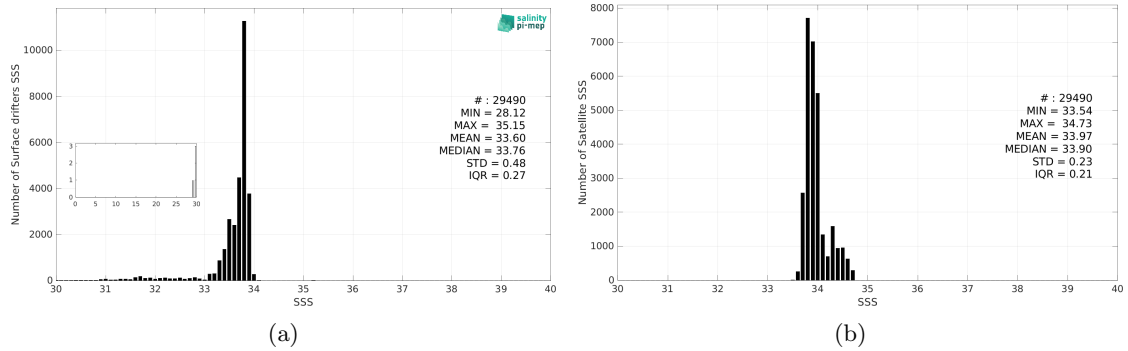
Figure 2: Histograms of SSS from Surface drifters (a) and SMOS SSS L3 v9 - 18 Days (CATDS-CEC-LOCEAN) (b) considering all match-up pairs per bins of 0.1 over the Southern Ocean Pi-MEP region and for the full satellite product period.
