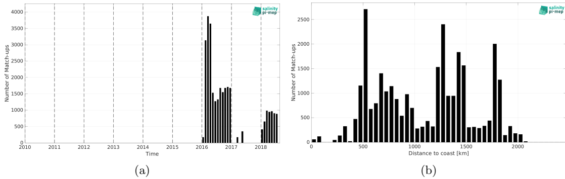
Figure 1: Number of match-ups between Surface drifters and SMOS SSS L3 v9 - 18 Days (CATDS-CEC-LOCEAN) SSS as a function of time (a) and as function of the distance to coast (b) over the Southern Ocean Pi-MEP region and for the full satellite product period.
