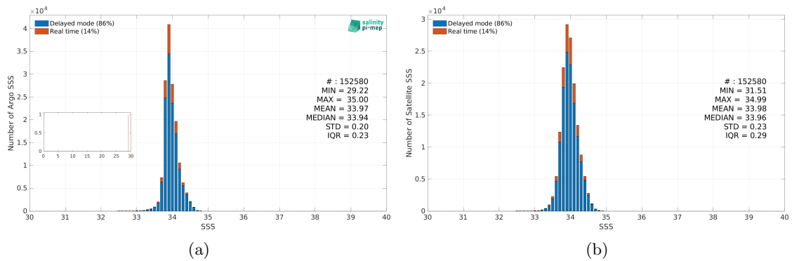
Figure 2: Histograms of SSS from Argo (a) and SMOS SSS L3 v9 - 18 Days (CATDS-CEC-LOCEAN) (b) considering all match-up pairs per bins of 0.1 over the Southern Ocean Pi-MEP region and for the full satellite product period.
