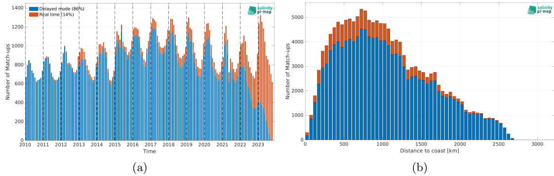
Figure 1: Number of match-ups between Argo and SMOS SSS L3 v9 - 18 Days (CATDS-CEC-LOCEAN) SSS as a function of time (a) and as function of the distance to coast (b) over the Southern Ocean Pi-MEP region and for the full satellite product period.
