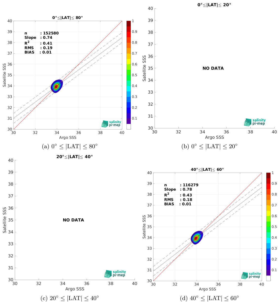
Figure 9: Contour maps of the concentration of SMOS SSS L3 v9 - 18 Days (CATDS-CEC-LOCEAN) SSS (y-axis) versus Argo SSS (x-axis) at match-up pairs for different latitude bands. For each plot, the red line shows x=y . The black thin and dashed lines indicate a linear fit through the data cloud and the \pm 95\% confidence levels, respectively. The number match-up pairs n , the slope and R^2 coefficient of the linear fit, the root mean square (RMS) and the mean bias between satellite and in situ data are indicated for each latitude band in each plots.
