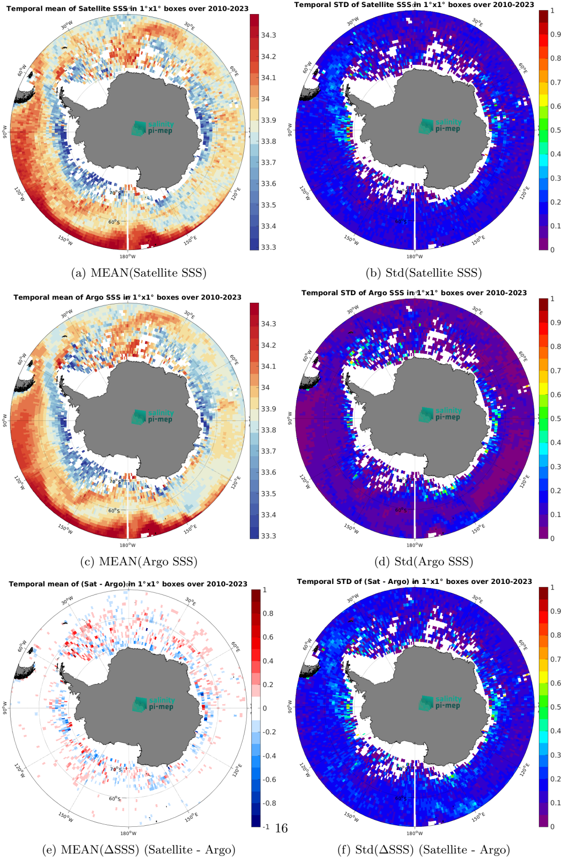
Figure 6: Temporal mean (left) and Std (right) of SSS from SMOS SSS L3 v9 - 18 Days (CATDS-CEC-LOCEAN) (top), Argo (middle), and of \Delta SSS (Satellite - Argo). Only match-up pairs are used to generate these maps.
