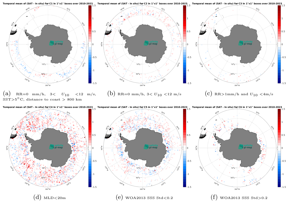
Figure 12: Temporal mean gridded over spatial boxes of size 1^{\circ}\times 1^{\circ} of \Delta\text{SSS} (SMOS SSS L3 v9 - 18 Days (CATDS-CEC-LOCEAN) - Argo) for 6 different subdatasets corresponding to:RR=0 mm/h, 3 < U_{10} < 12 m/s, SST >5^{\circ}\text{C} , distance to coast > 800 km (a), RR=0 mm/h, 3 < U_{10} < 12 m/s (b), RR >1 mm/h and U_{10} < 4 m/s (c),MLD <20 m (d),WOA2013 SSS Std <0.2 (e),WOA2013 SSS Std >0.2 (f).
