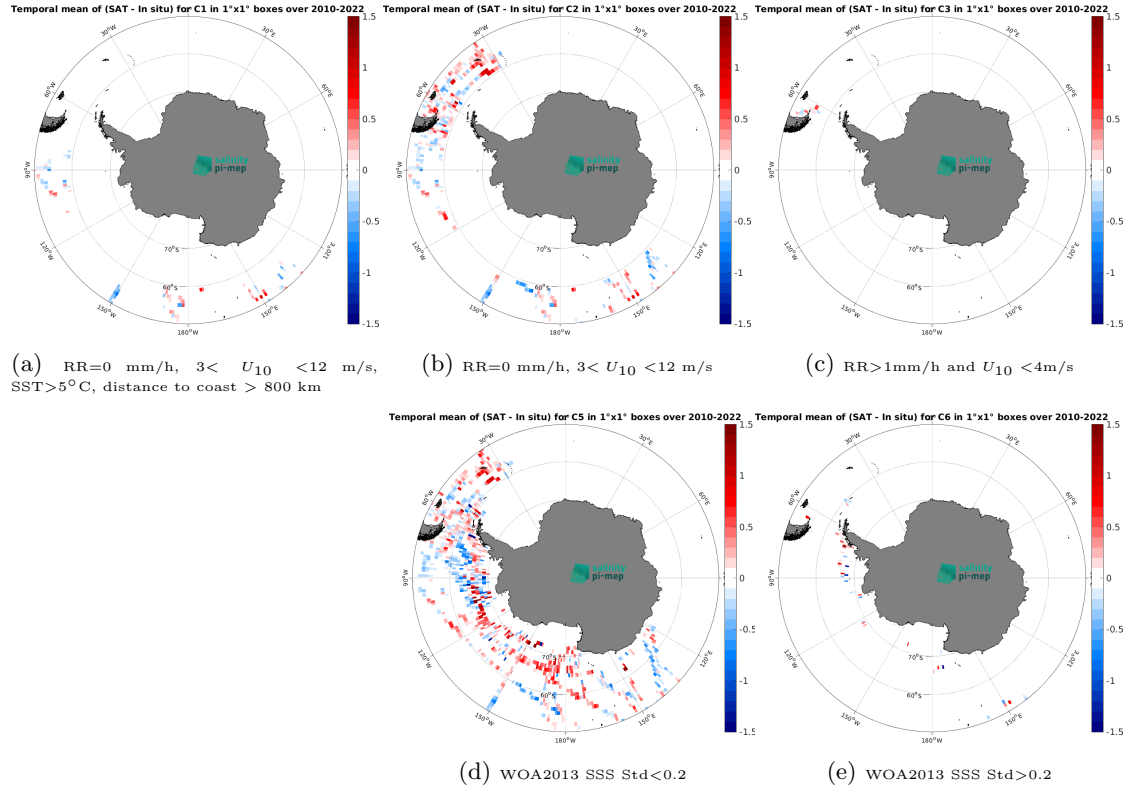
Figure 12: Temporal mean gridded over spatial boxes of size 1^{\circ}\times 1^{\circ} of \Delta\text{SSS} (SMOS SSS L3 v8 - 9 Days (CATDS-CEC-LOCEAN) - TSG (SAMOS)) for 5 different subdatasets corresponding to:RR=0 mm/h, 3 < U_{10} < 12 m/s, SST >5^{\circ}\text{C} , distance to coast > 800 km (a), RR=0 mm/h, 3 < U_{10} < 12 m/s (b), RR >1 mm/h and U_{10} < 4 m/s (c), WOA2013 SSS Std <0.2 (d), WOA2013 SSS Std >0.2 (e).
