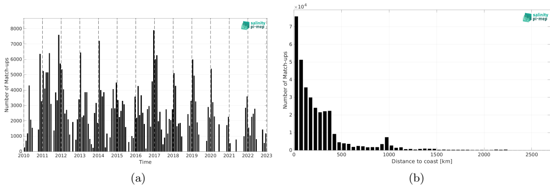
Figure 1: Number of match-ups between TSG (SAMOS) and SMOS SSS L3 v8 - 9 Days (CATDS-CEC-LOCEAN) SSS as a function of time (a) and as function of the distance to coast (b) over the Southern Ocean Pi-MEP region and for the full satellite product period.
