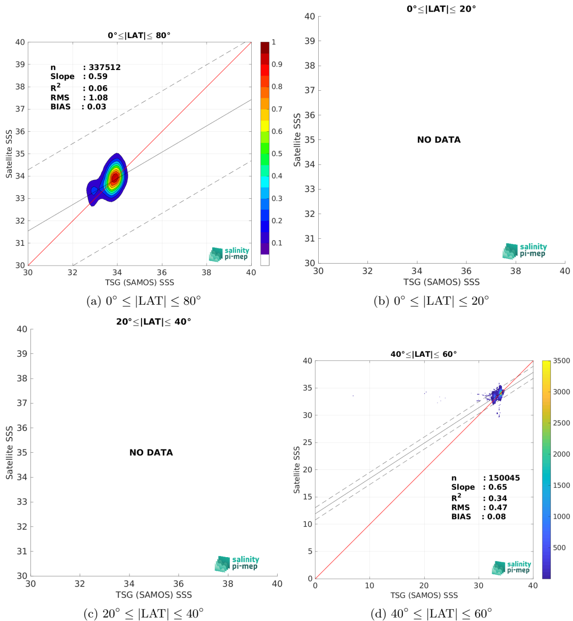
Figure 9: Contour maps of the concentration of SMOS SSS L3 v8 - 9 Days (CATDS-CEC-LOCEAN) SSS (y-axis) versus TSG (SAMOS) SSS (x-axis) at match-up pairs for different latitude bands. For each plot, the red line shows x=y . The black thin and dashed lines indicate a linear fit through the data cloud and the \pm 95\% confidence levels, respectively. The number match-up pairs n , the slope and R^2 coefficient of the linear fit, the root mean square (RMS) and the mean bias between satellite and in situ data are indicated for each latitude band in each plots.
