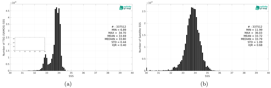
Figure 2: Histograms of SSS from TSG (SAMOS) (a) and SMOS SSS L3 v8 - 9 Days (CATDS-CEC-LOCEAN) (b) considering all match-up pairs per bins of 0.1 over the Southern Ocean Pi-MEP region and for the full satellite product period.
