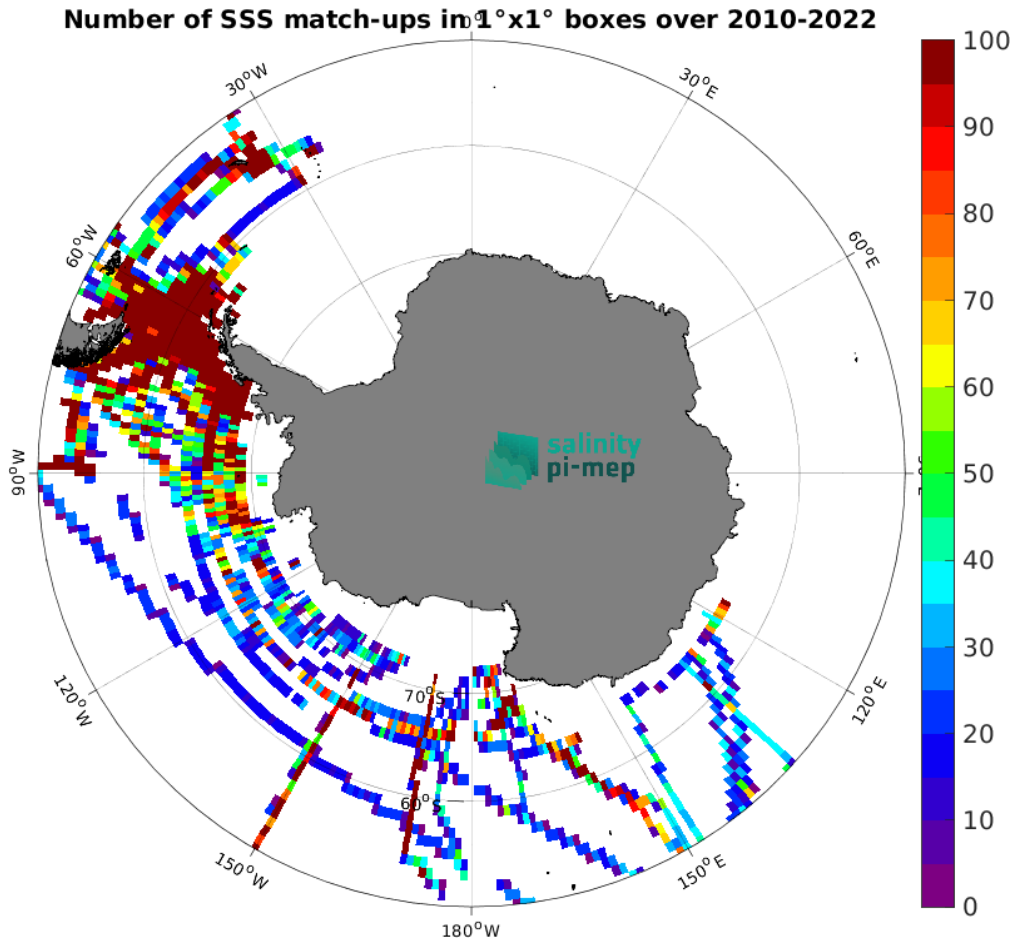
Figure 4: Number of SSS match-ups between TSG (SAMOS) SSS and the SMOS SSS L3 v8 - 9 Days (CATDS-CEC-LOCEAN) SSS product for the Southern Ocean Pi-MEP region over 1^\circ \times 1^\circ boxes and for the full satellite product period.
