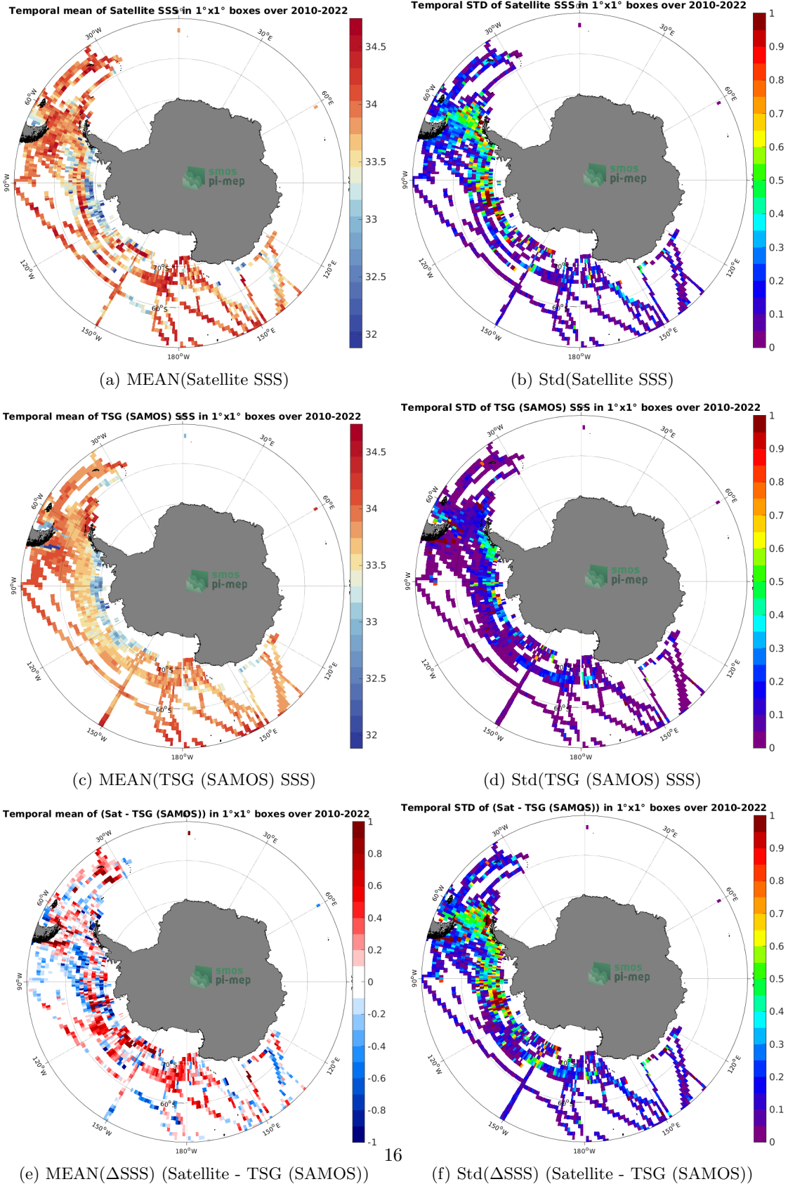
Figure 6: Temporal mean (left) and Std (right) of SSS from SMOS SSS L3 v8 - 9 Days (CATDS-CECOS-LOCEAN) (top), TSG (SAMOS) (middle), and of \Delta SSS (Satellite - TSG (SAMOS)). Only match-up pairs are used to generate these maps.
