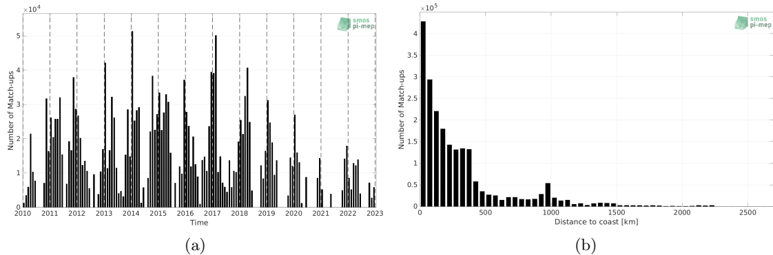
Figure 1: Number of match-ups between TSG (SAMOS) and SMOS SSS L3 v8 - 9 Days (CATDS-CECOS-LOCEAN) SSS as a function of time (a) and as function of the distance to coast (b) over the Southern Ocean Pi-MEP region and for the full satellite product period.
