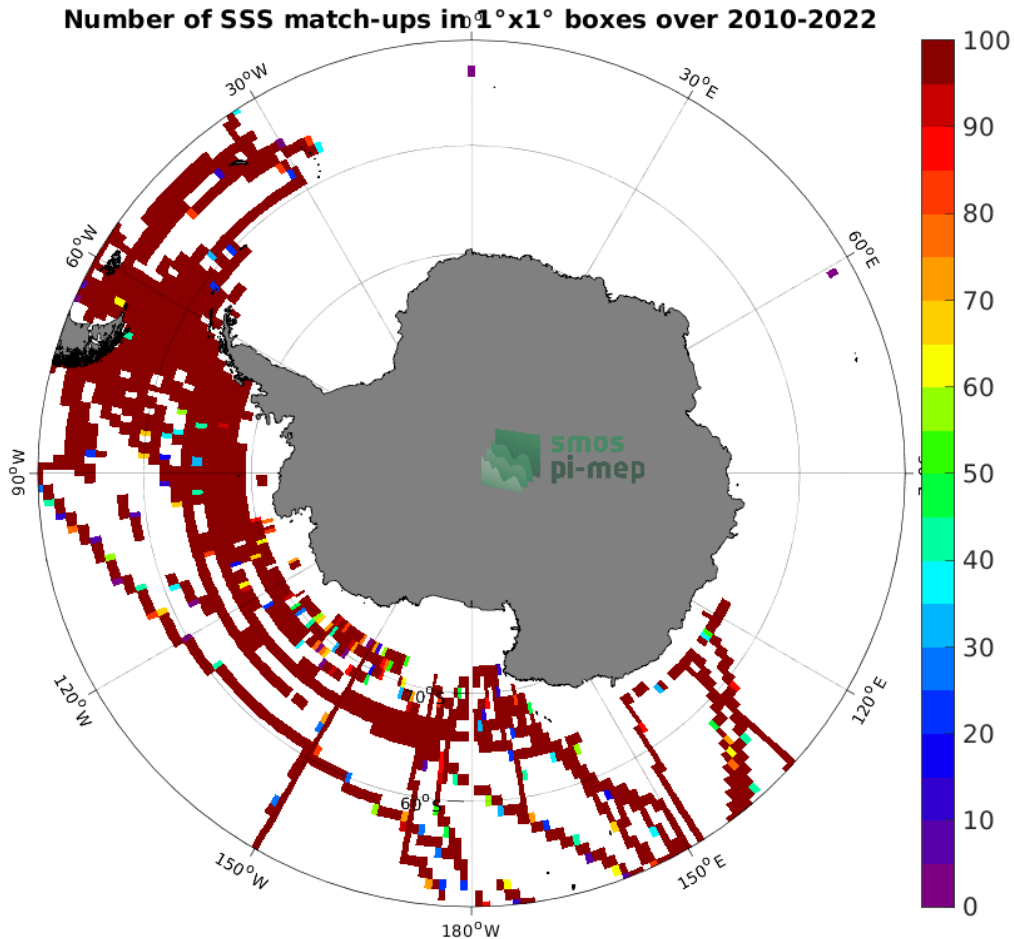
Figure 4: Number of SSS match-ups between TSG (SAMOS) SSS and the SMOS SSS L3 v8 - 9 Days (CATDS-CECOS-LOCEAN) SSS product for the Southern Ocean Pi-MEP region over 1^\circ \times 1^\circ boxes and for the full satellite product period.
