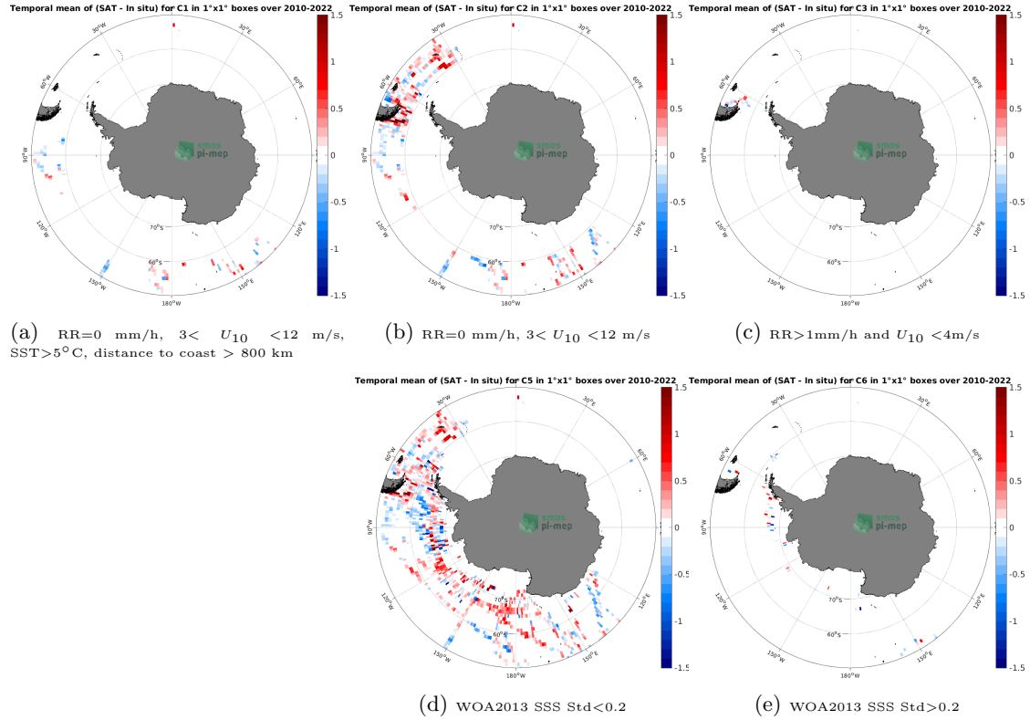
Figure 12: Temporal mean gridded over spatial boxes of size 1^{\circ}\times 1^{\circ} of \Delta\text{SSS} (SMOS SSS L3 v8 - 9 Days (CATDS-CECOS-LOCEAN) - TSG (SAMOS)) for 5 different subdatasets corresponding to:RR=0 mm/h, 3 < U_{10} < 12 m/s, SST >5^{\circ}\text{C} , distance to coast > 800 km (a), RR=0 mm/h, 3 < U_{10} < 12 m/s (b), RR >1 mm/h and U_{10} < 4 m/s (c), WOA2013 SSS Std <0.2 (d), WOA2013 SSS Std >0.2 (e).
