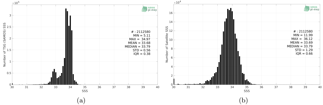
Figure 2: Histograms of SSS from TSG (SAMOS) (a) and SMOS SSS L3 v8 - 9 Days (CATDS-CECOS-LOCEAN) (b) considering all match-up pairs per bins of 0.1 over the Southern Ocean Pi-MEP region and for the full satellite product period.
