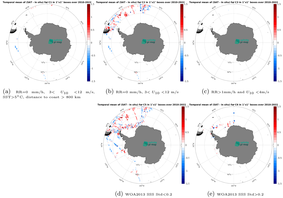
Figure 12: Temporal mean gridded over spatial boxes of size 1^{\circ}\times 1^{\circ} of \Delta\text{SSS} (SMOS SSS L3 v8 - 9 Days (CATDS-CEC-LOCEAN) - TSG (Polarstern)) for 5 different subdatasets corresponding to: RR=0 mm/h, 3 < U_{10} < 12 m/s, SST > 5^{\circ}\text{C} , distance to coast > 800 km (a), RR=0 mm/h, 3 < U_{10} < 12 m/s (b), RR > 1 mm/h and U_{10} < 4 m/s (c), WOA2013 SSS Std < 0.2 (d), WOA2013 SSS Std > 0.2 (e).
