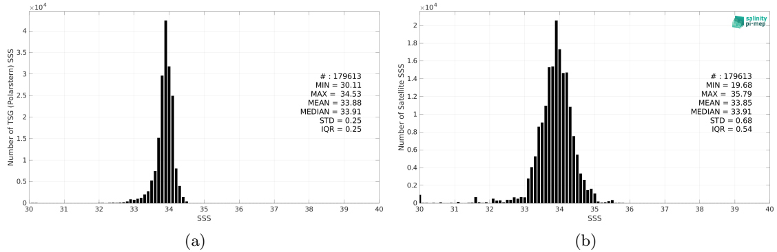
Figure 2: Histograms of SSS from TSG (Polarstern) (a) and SMOS SSS L3 v8 - 9 Days (CATDS-CEC-LOCEAN) (b) considering all match-up pairs per bins of 0.1 over the Southern Ocean Pi-MEP region and for the full satellite product period.
