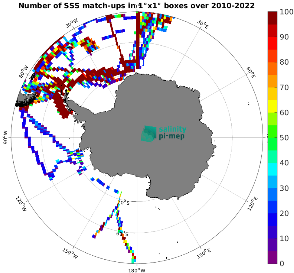
Figure 4: Number of SSS match-ups between TSG (Polarstern) SSS and the SMOS SSS L3 v8 - 9 Days (CATDS-CEC-LOCEAN) SSS product for the Southern Ocean Pi-MEP region over 1^\circ \times 1^\circ boxes and for the full satellite product period.
