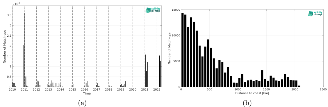
Figure 1: Number of match-ups between TSG (Polarstern) and SMOS SSS L3 v8 - 9 Days (CATDS-CEC-LOCEAN) SSS as a function of time (a) and as function of the distance to coast (b) over the Southern Ocean Pi-MEP region and for the full satellite product period.
