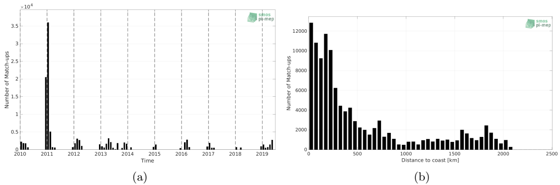
Figure 1: Number of match-ups between TSG (Polarstern) and SMOS SSS L3 v8 - 9 Days (CATDS-CECOS-LOCEAN) SSS as a function of time (a) and as function of the distance to coast (b) over the Southern Ocean Pi-MEP region and for the full satellite product period.
