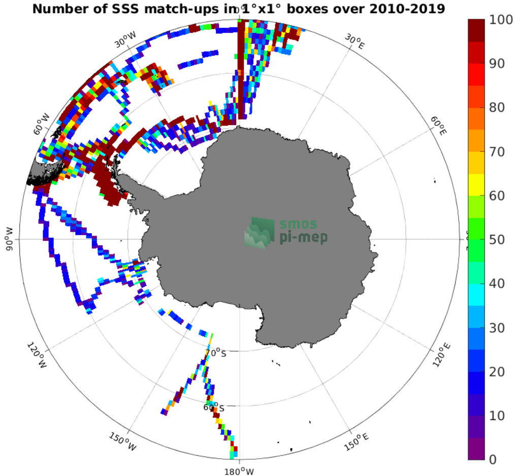
Figure 4: Number of SSS match-ups between TSG (Polarstern) SSS and the SMOS SSS L3 v8 - 9 Days (CATDS-CECOS-LOCEAN) SSS product for the Southern Ocean Pi-MEP region over 1^\circ \times 1^\circ boxes and for the full satellite product period.
