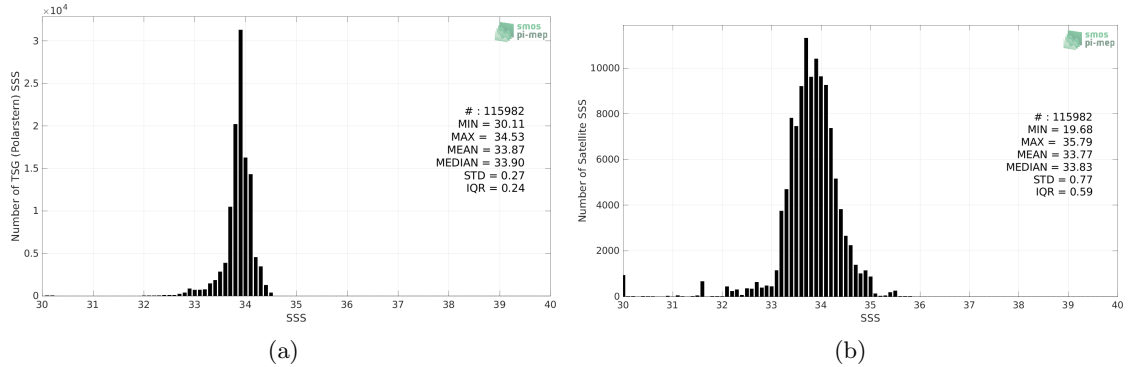
Figure 2: Histograms of SSS from TSG (Polarstern) (a) and SMOS SSS L3 v8 - 9 Days (CATDS-CECOS-LOCEAN) (b) considering all match-up pairs per bins of 0.1 over the Southern Ocean Pi-MEP region and for the full satellite product period.
