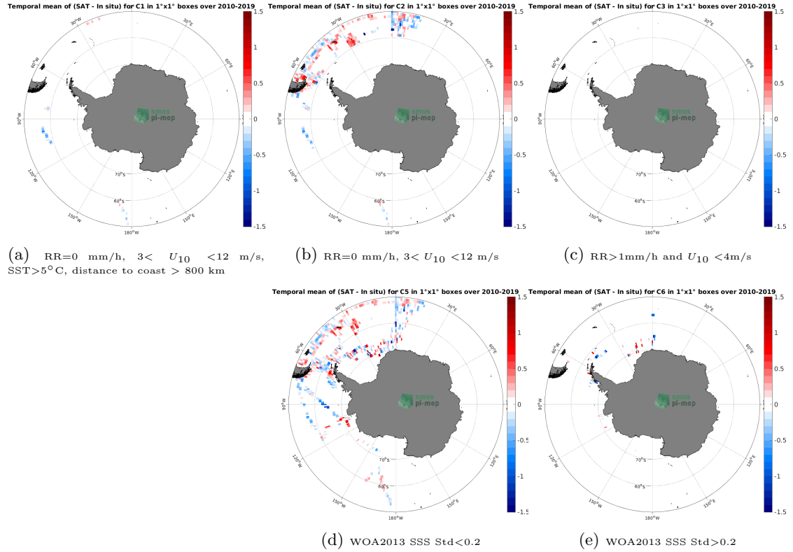
Figure 12: Temporal mean gridded over spatial boxes of size 1^{\circ}\times 1^{\circ} of \Delta\text{SSS} (SMOS SSS L3 v8 - 9 Days (CATDS-CECOS-LOCEAN) - TSG (Polarstern)) for 5 different subdatasets corresponding to:RR=0 mm/h, 3 < U_{10} < 12 m/s, SST >5^{\circ}\text{C} , distance to coast > 800 km (a), RR=0 mm/h, 3 < U_{10} < 12 m/s (b), RR >1 mm/h and U_{10} < 4 m/s (c), WOA2013 SSS Std <0.2 (d), WOA2013 SSS Std >0.2 (e).
