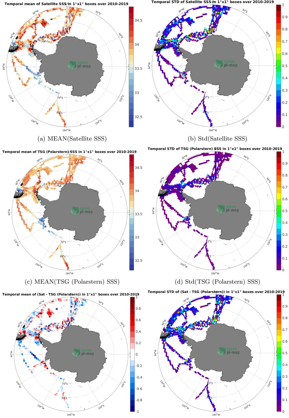
Figure 6: Temporal mean (left) and Std (right) of SSS from SMOS SSS L3 v8 - 9 Days (CATDS-CECOS-LOCEAN) (top), TSG (Polarstern) (middle), and of \Delta SSS (Satellite - TSG (Polarstern)). Only match-up pairs are used to generate these maps.
