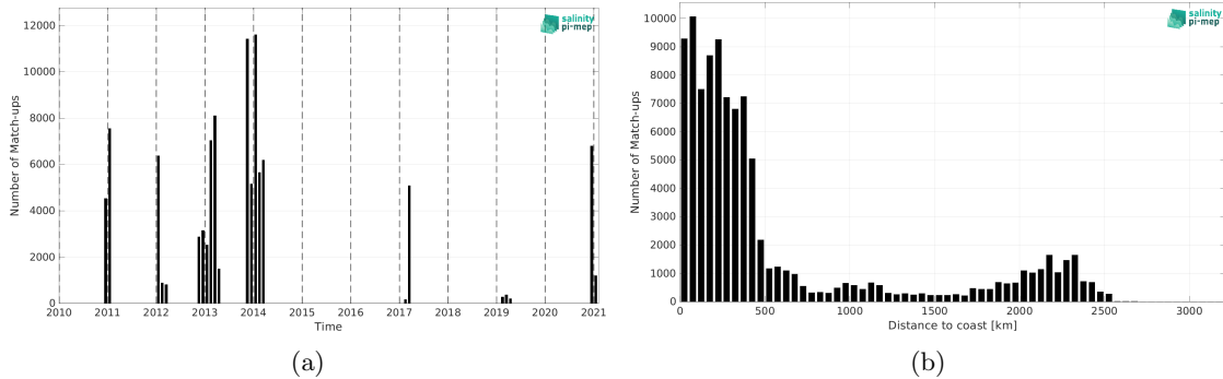
Figure 1: Number of match-ups between TSG (GOSUD-Sailing-ship) and SMOS SSS L3 v8 - 9 Days (CATDS-CEC-LOCEAN) SSS as a function of time (a) and as function of the distance to coast (b) over the Southern Ocean Pi-MEP region and for the full satellite product period.
