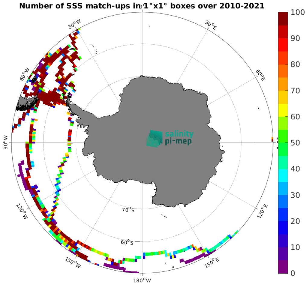
Figure 4: Number of SSS match-ups between TSG (GOSUD-Sailing-ship) SSS and the SMOS SSS L3 v8 - 9 Days (CATDS-CEC-LOCEAN) SSS product for the Southern Ocean Pi-MEP region over 1^\circ \times 1^\circ boxes and for the full satellite product period.
