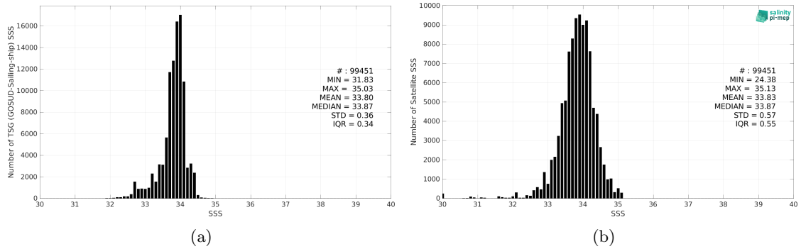
Figure 2: Histograms of SSS from TSG (GOSUD-Sailing-ship) (a) and SMOS SSS L3 v8 - 9 Days (CATDS-CEC-LOCEAN) (b) considering all match-up pairs per bins of 0.1 over the Southern Ocean Pi-MEP region and for the full satellite product period.
