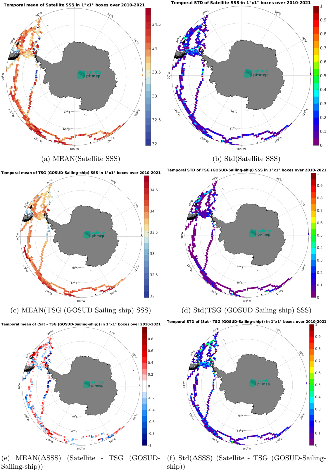
Figure 6: Temporal mean (left) and Std (right) of SSS from SMOS SSS L3 v8 - 9 Days (CATDS-CEC-LOCEAN) (top), TSG (GOSUD-Sailing-ship) (middle), and of \Delta SSS (Satellite - TSG (GOSUD-Sailing-ship)). Only match-up pairs are used to generate these maps.
