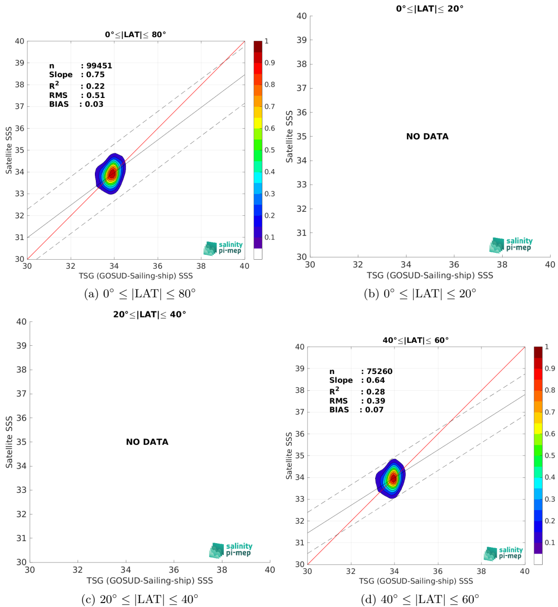
Figure 9: Contour maps of the concentration of SMOS SSS L3 v8 - 9 Days (CATDS-CEC-LOCEAN) SSS (y-axis) versus TSG (GOSUD-Sailing-ship) SSS (x-axis) at match-up pairs for different latitude bands. For each plot, the red line shows x=y . The black thin and dashed lines indicate a linear fit through the data cloud and the \pm 95\% confidence levels, respectively. The number match-up pairs n , the slope and R^2 coefficient of the linear fit, the root mean square (RMS) and the mean bias between satellite and in situ data are indicated for each latitude band in each plots.
