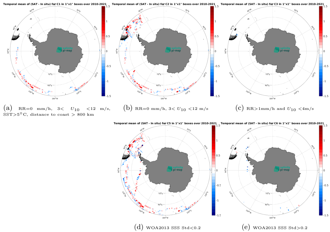
Figure 12: Temporal mean gridded over spatial boxes of size 1^\circ \times 1^\circ of \Delta\text{SSS} (SMOS SSS L3 v8 - 9 Days (CATDS-CEC-LOCEAN) - TSG (GOSUD-Sailing-ship)) for 5 different subdatasets corresponding to: RR=0 mm/h, 3 < U_{10} < 12 m/s, SST > 5^\circ\text{C} , distance to coast > 800 km (a), RR=0 mm/h, 3 < U_{10} < 12 m/s (b), RR > 1 mm/h and U_{10} < 4 m/s (c), WOA2013 SSS Std < 0.2 (d), WOA2013 SSS Std > 0.2 (e).
