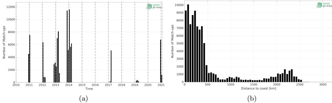
Figure 1: Number of match-ups between TSG (GOSUD-Sailing-ship) and SMOS SSS L3 v8 - 9 Days (CATDS-CECOS-LOCEAN) SSS as a function of time (a) and as function of the distance to coast (b) over the Southern Ocean Pi-MEP region and for the full satellite product period.
