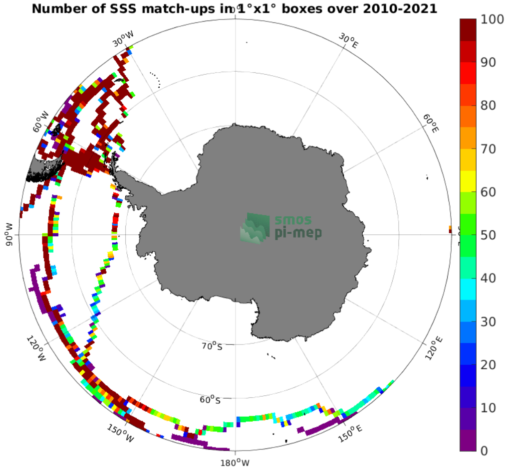
Figure 4: Number of SSS match-ups between TSG (GOSUD-Sailing-ship) SSS and the SMOS SSS L3 v8 - 9 Days (CATDS-CECOS-LOCEAN) SSS product for the Southern Ocean Pi-MEP region over 1^\circ \times 1^\circ boxes and for the full satellite product period.
