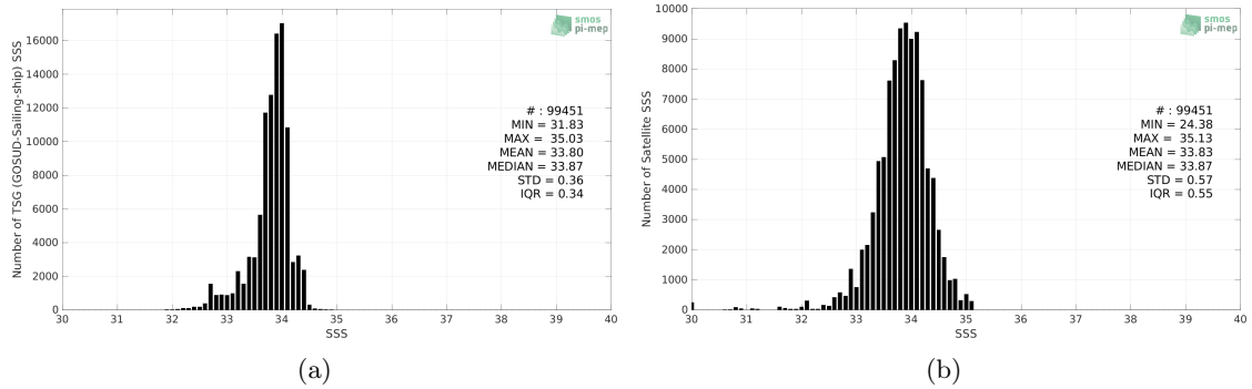
Figure 2: Histograms of SSS from TSG (GOSUD-Sailing-ship) (a) and SMOS SSS L3 v8 - 9 Days (CATDS-CECOS-LOCEAN) (b) considering all match-up pairs per bins of 0.1 over the Southern Ocean Pi-MEP region and for the full satellite product period.
