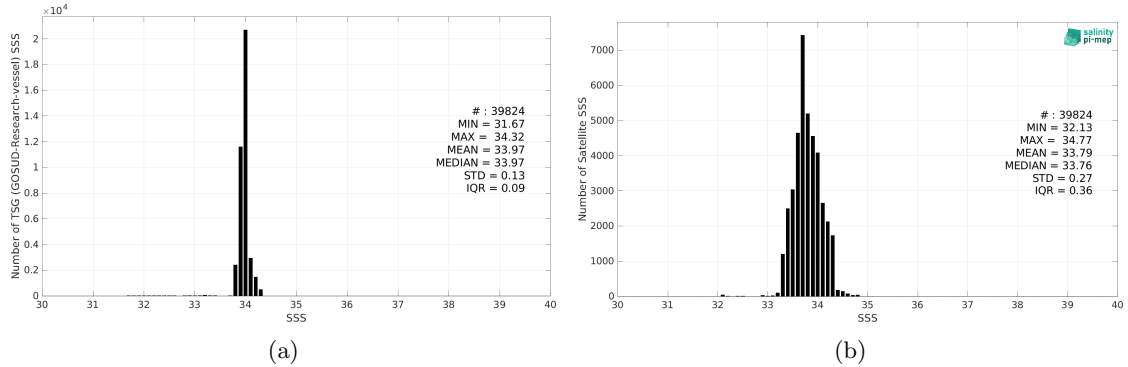
Figure 2: Histograms of SSS from TSG (GOSUD-Research-vessel) (a) and SMOS SSS L3 v8 - 9 Days (CATDS-CEC-LOCEAN) (b) considering all match-up pairs per bins of 0.1 over the Southern Ocean Pi-MEP region and for the full satellite product period.
