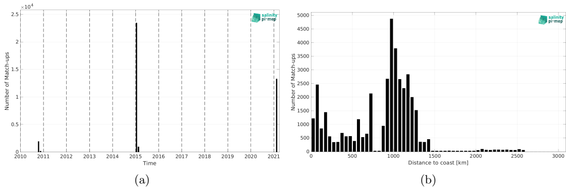
Figure 1: Number of match-ups between TSG (GOSUD-Research-vessel) and SMOS SSS L3 v8 - 9 Days (CATDS-CEC-LOCEAN) SSS as a function of time (a) and as function of the distance to coast (b) over the Southern Ocean Pi-MEP region and for the full satellite product period.
