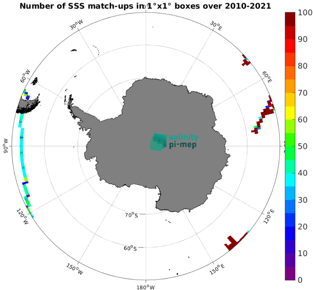
Figure 4: Number of SSS match-ups between TSG (GOSUD-Research-vessel) SSS and the SMOS SSS L3 v8 - 9 Days (CATDS-CEC-LOCEAN) SSS product for the Southern Ocean Pi-MEP region over 1^\circ \times 1^\circ boxes and for the full satellite product period.
