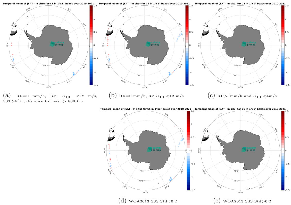
Figure 12: Temporal mean gridded over spatial boxes of size 1^\circ \times 1^\circ of \Delta\text{SSS} (SMOS SSS L3 v8 - 9 Days (CATDS-CEC-LOCEAN) - TSG (GOSUD-Research-vessel)) for 5 different subdatasets corresponding to: RR=0 mm/h, 3 < U_{10} < 12 m/s, SST > 5^\circ\text{C} , distance to coast > 800 km (a), RR=0 mm/h, 3 < U_{10} < 12 m/s (b), RR > 1 mm/h and U_{10} < 4 m/s (c), WOA2013 SSS Std < 0.2 (d), WOA2013 SSS Std > 0.2 (e).
