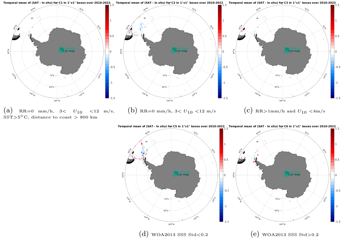
Figure 12: Temporal mean gridded over spatial boxes of size 1^{\circ}\times 1^{\circ} of \Delta\text{SSS} (SMOS SSS L3 v8 - 9 Days (CATDS-CEC-LOCEAN) - TSG (CSIC-UTM)) for 5 different subdatasets corresponding to:RR=0 mm/h, 3 < U_{10} < 12 m/s, SST >5^{\circ}\text{C} , distance to coast > 800 km (a), RR=0 mm/h, 3 < U_{10} < 12 m/s (b), RR >1 mm/h and U_{10} < 4 m/s (c), WOA2013 SSS Std <0.2 (d), WOA2013 SSS Std >0.2 (e).
