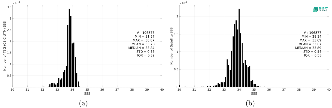
Figure 2: Histograms of SSS from TSG (CSIC-UTM) (a) and SMOS SSS L3 v8 - 9 Days (CATDS-CEC-LOCEAN) (b) considering all match-up pairs per bins of 0.1 over the Southern Ocean Pi-MEP region and for the full satellite product period.
