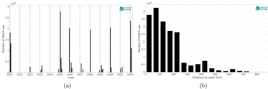
Figure 1: Number of match-ups between TSG (CSIC-UTM) and SMOS SSS L3 v8 - 9 Days (CATDS-CEC-LOCEAN) SSS as a function of time (a) and as function of the distance to coast (b) over the Southern Ocean Pi-MEP region and for the full satellite product period.
