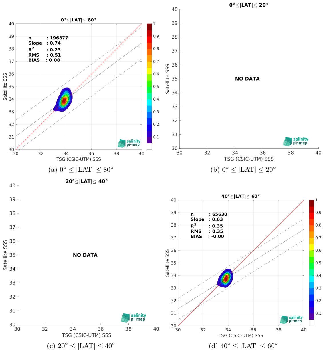
Figure 9: Contour maps of the concentration of SMOS SSS L3 v8 - 9 Days (CATDS-CEC-LOCEAN) SSS (y-axis) versus TSG (CSIC-UTM) SSS (x-axis) at match-up pairs for different latitude bands. For each plot, the red line shows x=y . The black thin and dashed lines indicate a linear fit through the data cloud and the \pm 95\% confidence levels, respectively. The number match-up pairs n , the slope and R^2 coefficient of the linear fit, the root mean square (RMS) and the mean bias between satellite and in situ data are indicated for each latitude band in each plots.
