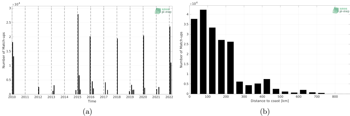
Figure 1: Number of match-ups between TSG (CSIC-UTM) and SMOS SSS L3 v8 - 9 Days (CATDS-CECOS-LOCEAN) SSS as a function of time (a) and as function of the distance to coast (b) over the Southern Ocean Pi-MEP region and for the full satellite product period.
