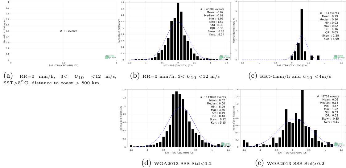
Figure 13: Normalized histogram of \Delta SSS (SMOS SSS L3 v8 - 9 Days (CATDS-CECOS-LOCEAN) - TSG (CSIC-UTM)) for 5 different subdatasets corresponding to: RR=0 mm/h, 3 < U_{10} < 12 m/s, SST>5°C, distance to coast > 800 km (a), RR=0 mm/h, 3 < U_{10} < 12 m/s (b), RR>1mm/h and U_{10} < 4 m/s (c), WOA2013 SSS Std<0.2 (d), WOA2013 SSS Std>0.2 (e).
