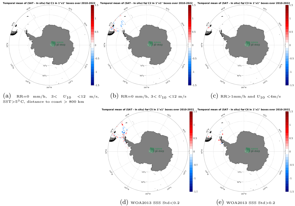
Figure 12: Temporal mean gridded over spatial boxes of size 1^{\circ}\times 1^{\circ} of \Delta\text{SSS} (SMOS SSS L3 v8 - 9 Days (CATDS-CECOS-LOCEAN) - TSG (CSIC-UTM)) for 5 different subdatasets corresponding to: \text{RR}=0 mm/h, 3 < U_{10} < 12 m/s, \text{SST}>5^{\circ}\text{C} , distance to coast > 800 km (a), \text{RR}=0 mm/h, 3 < U_{10} < 12 m/s (b), \text{RR}>1 mm/h and U_{10} < 4 m/s (c), WOA2013 SSS Std < 0.2 (d), WOA2013 SSS Std > 0.2 (e).
