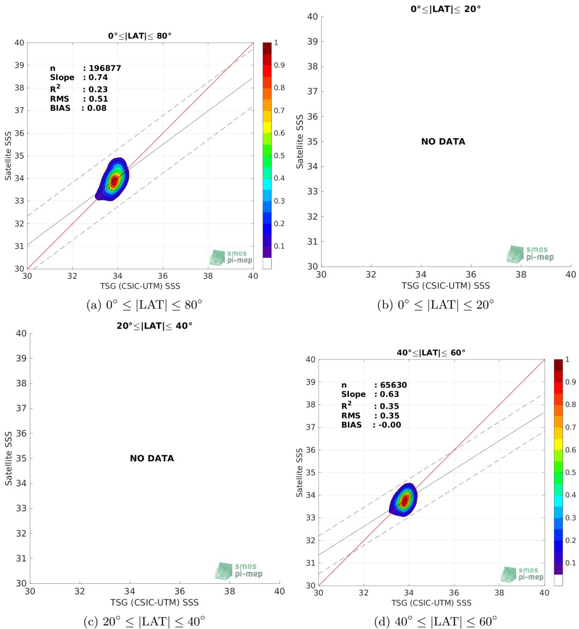
Figure 9: Contour maps of the concentration of SMOS SSS L3 v8 - 9 Days (CATDS-CECOS-LOCEAN) SSS (y-axis) versus TSG (CSIC-UTM) SSS (x-axis) at match-up pairs for different latitude bands. For each plot, the red line shows x=y . The black thin and dashed lines indicate a linear fit through the data cloud and the \pm 95\% confidence levels, respectively. The number match-up pairs n , the slope and R^2 coefficient of the linear fit, the root mean square (RMS) and the mean bias between satellite and in situ data are indicated for each latitude band in each plots.
