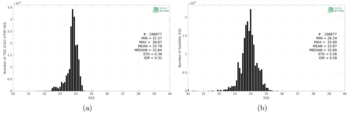
Figure 2: Histograms of SSS from TSG (CSIC-UTM) (a) and SMOS SSS L3 v8 - 9 Days (CATDS-CECOS-LOCEAN) (b) considering all match-up pairs per bins of 0.1 over the Southern Ocean Pi-MEP region and for the full satellite product period.
