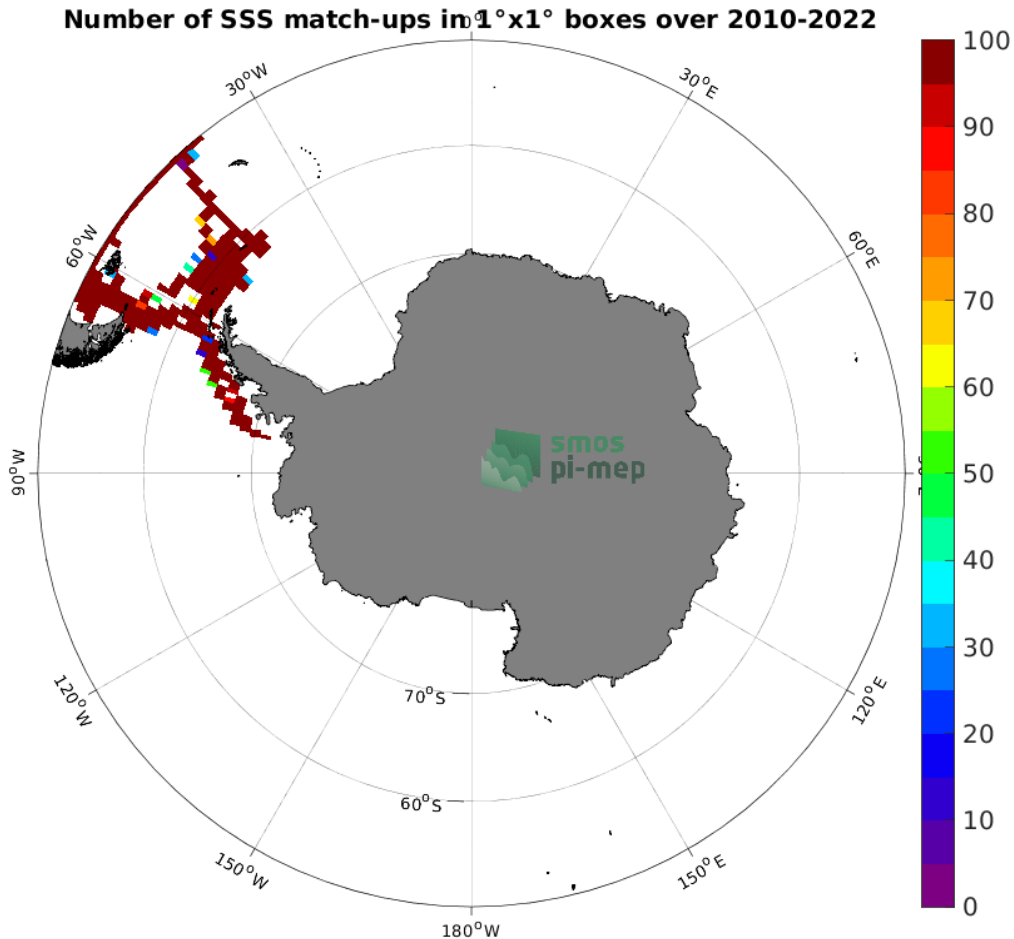
Figure 4: Number of SSS match-ups between TSG (CSIC-UTM) SSS and the SMOS SSS L3 v8 - 9 Days (CATDS-CECOS-LOCEAN) SSS product for the Southern Ocean Pi-MEP region over 1^\circ \times 1^\circ boxes and for the full satellite product period.
