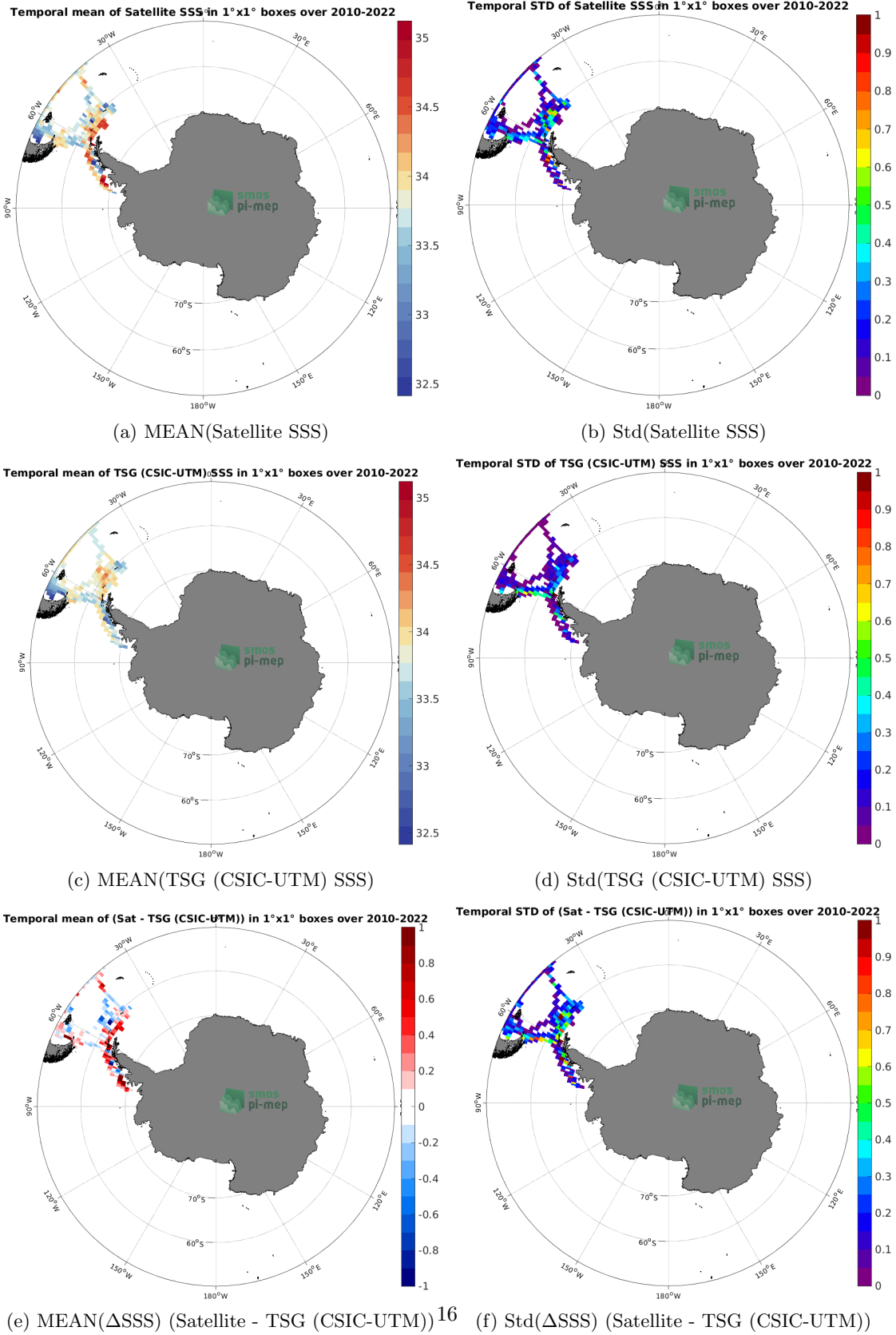
Figure 6: Temporal mean (left) and Std (right) of SSS from SMOS SSS L3 v8 - 9 Days (CATDS-CECOS-LOCEAN) (top), TSG (CSIC-UTM) (middle), and of \Delta SSS (Satellite - TSG (CSIC-UTM)). Only match-up pairs are used to generate these maps.
