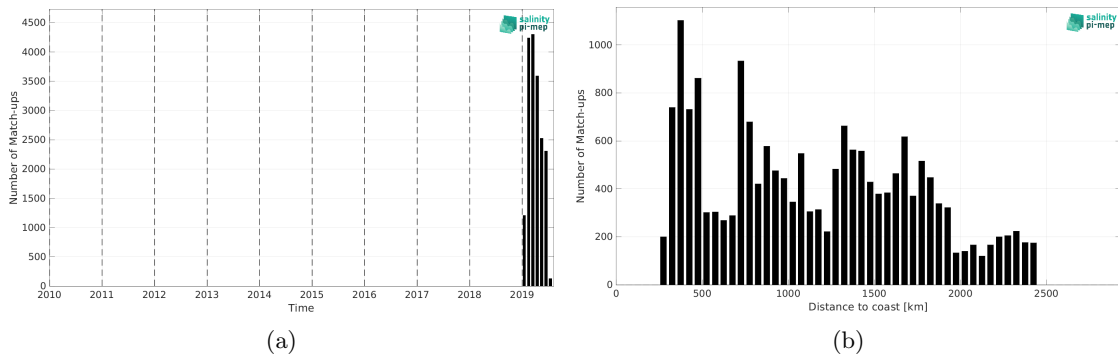
Figure 1: Number of match-ups between Saildrone and SMOS SSS L3 v8 - 9 Days (CATDS-CEC-LOCEAN) SSS as a function of time (a) and as function of the distance to coast (b) over the Southern Ocean Pi-MEP region and for the full satellite product period.
