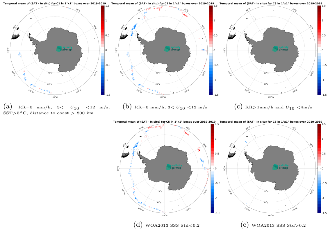
Figure 12: Temporal mean gridded over spatial boxes of size 1^{\circ}\times 1^{\circ} of \Delta\text{SSS} (SMOS SSS L3 v8 - 9 Days (CATDS-CEC-LOCEAN) - Saildrone) for 5 different subdatasets corresponding to:RR=0 mm/h, 3 < U_{10} < 12 m/s, SST >5^{\circ}\text{C} , distance to coast > 800 km (a), RR=0 mm/h, 3 < U_{10} < 12 m/s (b), RR >1 mm/h and U_{10} < 4 m/s (c), WOA2013 SSS Std <0.2 (d), WOA2013 SSS Std >0.2 (e).
