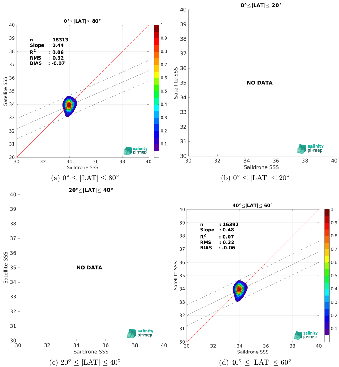
Figure 9: Contour maps of the concentration of SMOS SSS L3 v8 - 9 Days (CATDS-CEC-LOCEAN) SSS (y-axis) versus Saildrone SSS (x-axis) at match-up pairs for different latitude bands. For each plot, the red line shows x=y . The black thin and dashed lines indicate a linear fit through the data cloud and the \pm 95\% confidence levels, respectively. The number match-up pairs n , the slope and R^2 coefficient of the linear fit, the root mean square (RMS) and the mean bias between satellite and in situ data are indicated for each latitude band in each plots.
