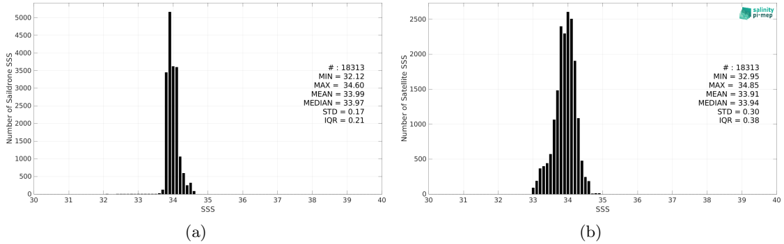
Figure 2: Histograms of SSS from Sairdrone (a) and SMOS SSS L3 v8 - 9 Days (CATDS-CEC-LOCEAN) (b) considering all match-up pairs per bins of 0.1 over the Southern Ocean Pi-MEP region and for the full satellite product period.
