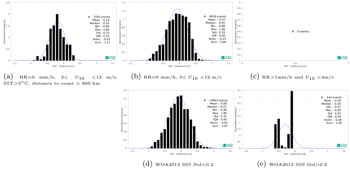
Figure 13: Normalized histogram of \Delta SSS (SMOS SSS L3 v8 - 9 Days (CATDS-CEC-LOCEAN) - Saildrone) for 5 different subdatasets corresponding to: RR=0 mm/h, 3 < U_{10} < 12 m/s, SST > 5°C, distance to coast > 800 km (a), RR=0 mm/h, 3 < U_{10} < 12 m/s (b), RR > 1mm/h and U_{10} < 4 m/s (c), WOA2013 SSS Std < 0.2 (d), WOA2013 SSS Std > 0.2 (e).
