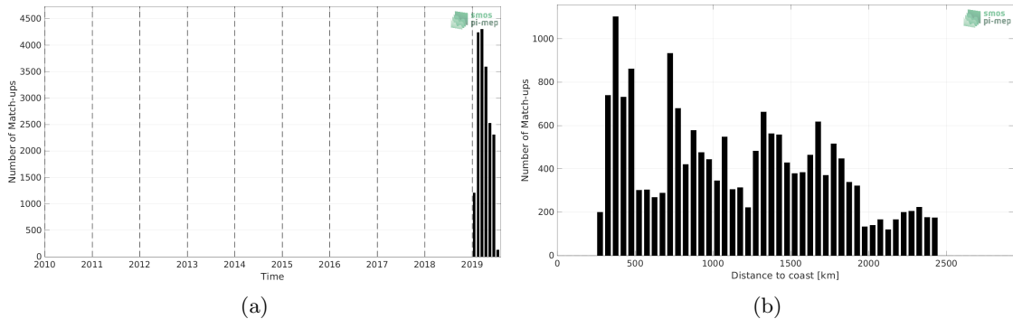
Figure 1: Number of match-ups between Saildrone and SMOS SSS L3 v8 - 9 Days (CATDS-CECOS-LOCEAN) SSS as a function of time (a) and as function of the distance to coast (b) over the Southern Ocean Pi-MEP region and for the full satellite product period.
