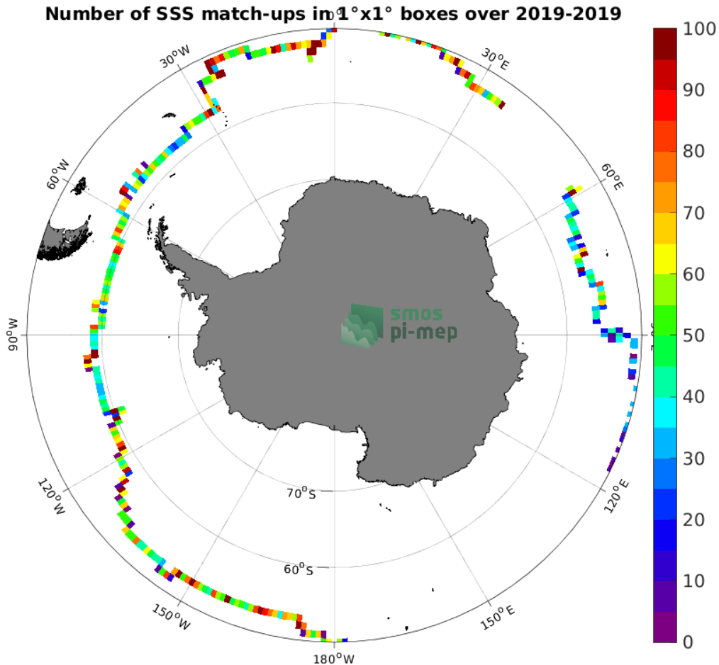
Figure 4: Number of SSS match-ups between Saildrone SSS and the SMOS SSS L3 v8 - 9 Days (CATDS-CECOS-LOCEAN) SSS product for the Southern Ocean Pi-MEP region over 1^\circ \times 1^\circ boxes and for the full satellite product period.
