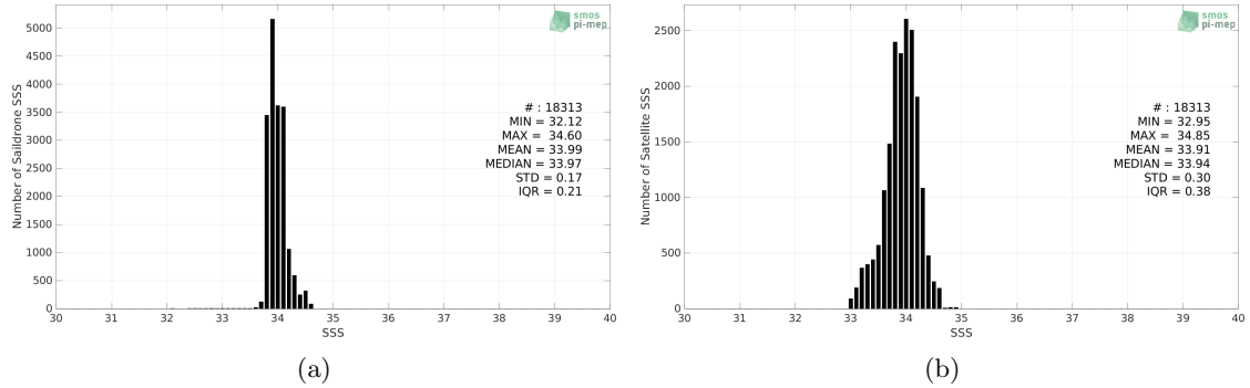
Figure 2: Histograms of SSS from Saildrone (a) and SMOS SSS L3 v8 - 9 Days (CATDS-CECOS-LOCEAN) (b) considering all match-up pairs per bins of 0.1 over the Southern Ocean Pi-MEP region and for the full satellite product period.
