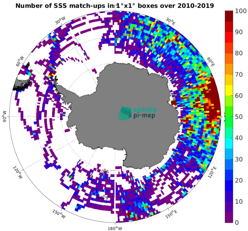
Figure 4: Number of SSS match-ups between Marine mammals SSS and the SMOS SSS L3 v8 - 9 Days (CATDS-CEC-LOCEAN) SSS product for the Southern Ocean Pi-MEP region over 1^\circ \times 1^\circ boxes and for the full satellite product period.
