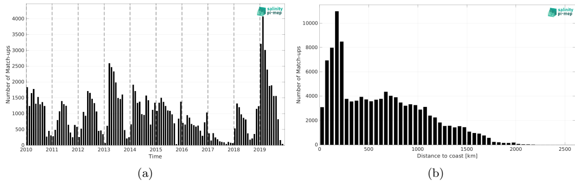
Figure 1: Number of match-ups between Marine mammals and SMOS SSS L3 v8 - 9 Days (CATDS-CEC-LOCEAN) SSS as a function of time (a) and as function of the distance to coast (b) over the Southern Ocean Pi-MEP region and for the full satellite product period.
