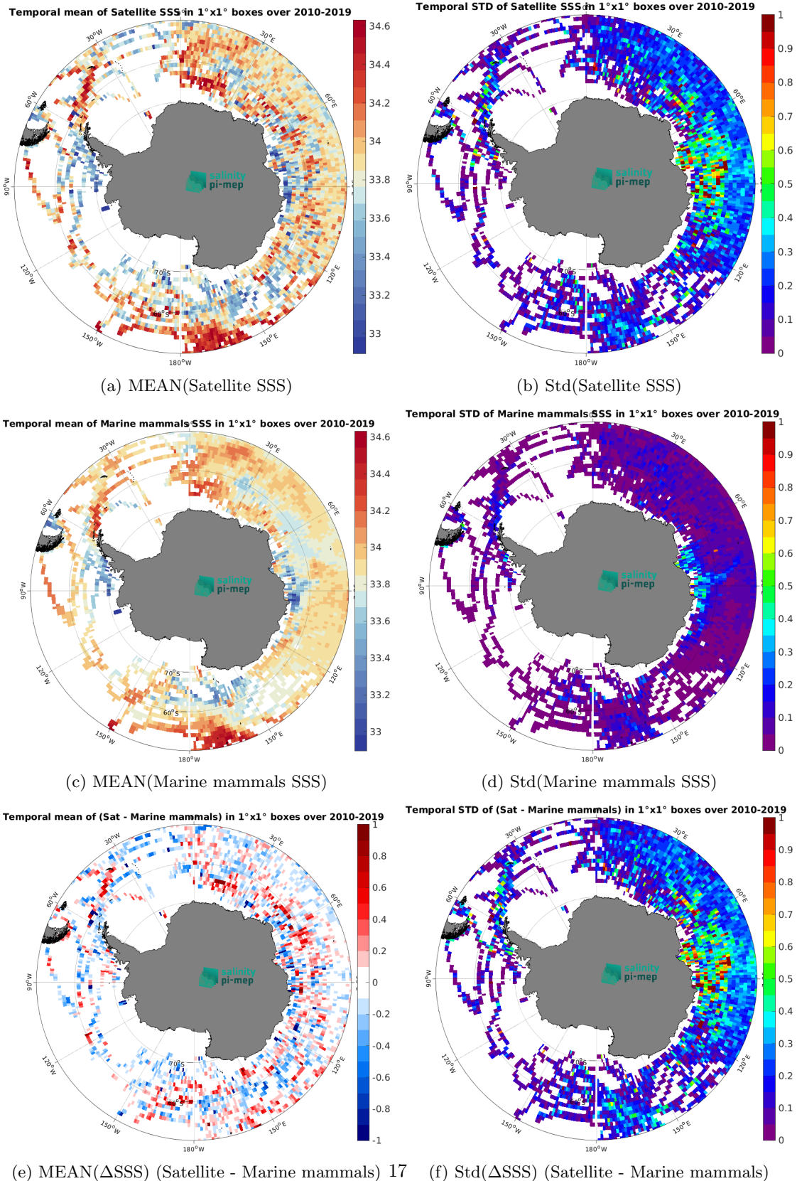
Figure 6: Temporal mean (left) and Std (right) of SSS from SMOS SSS L3 v8 - 9 Days (CATDS-CEC-LOCEAN) (top), Marine mammals (middle), and of \Delta SSS (Satellite - Marine mammals). Only match-up pairs are used to generate these maps.
