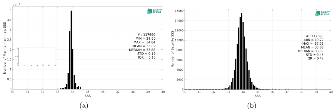
Figure 2: Histograms of SSS from Marine mammals (a) and SMOS SSS L3 v8 - 9 Days (CATDS-CEC-LOCEAN) (b) considering all match-up pairs per bins of 0.1 over the Southern Ocean Pi-MEP region and for the full satellite product period.
