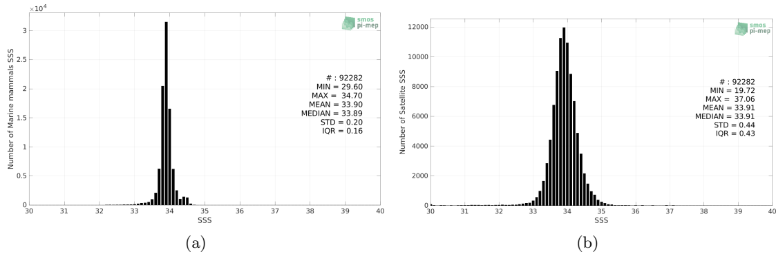
Figure 2: Histograms of SSS from Marine mammals (a) and SMOS SSS L3 v8 - 9 Days (CATDS-CECOS-LOCEAN) (b) considering all match-up pairs per bins of 0.1 over the Southern Ocean Pi-MEP region and for the full satellite product period.
