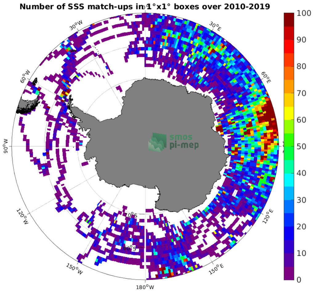
Figure 4: Number of SSS match-ups between Marine mammals SSS and the SMOS SSS L3 v8 - 9 Days (CATDS-CECOS-LOCEAN) SSS product for the Southern Ocean Pi-MEP region over 1^\circ \times 1^\circ boxes and for the full satellite product period.
