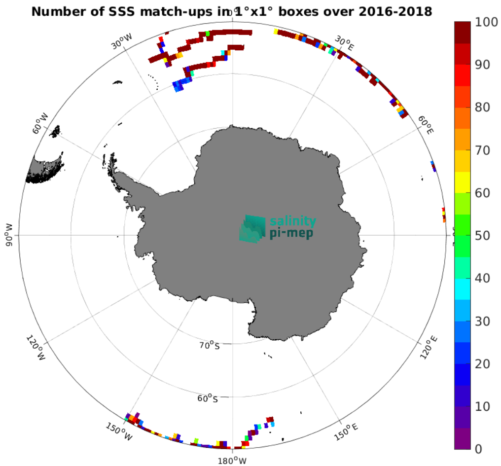
Figure 3: Number of SSS match-ups between Surface drifters SSS and the SMOS SSS L3 v8 - 9 Days (CATDS-CEC-LOCEAN) SSS product for the Southern Ocean Pi-MEP region over 1^\circ \times 1^\circ boxes and for the full satellite product period.
