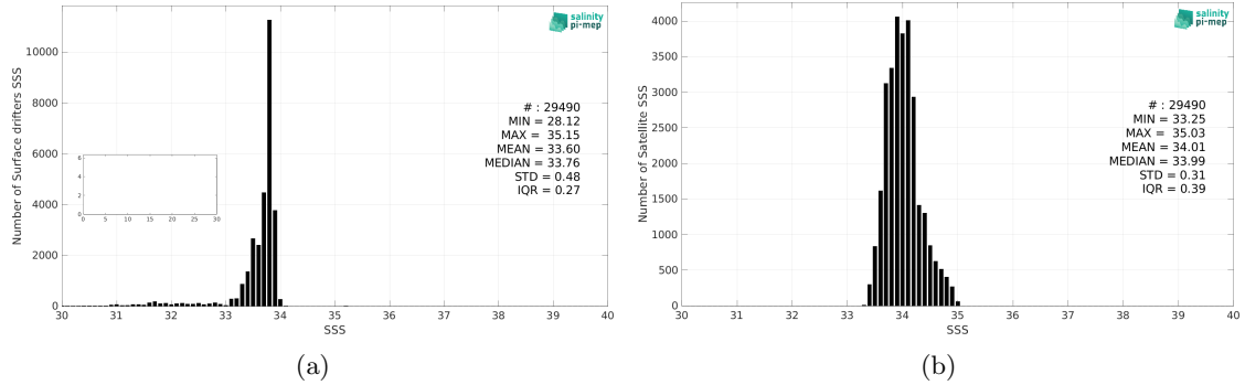
Figure 2: Histograms of SSS from Surface drifters (a) and SMOS SSS L3 v8 - 9 Days (CATDS-CEC-LOCEAN) (b) considering all match-up pairs per bins of 0.1 over the Southern Ocean Pi-MEP region and for the full satellite product period.
