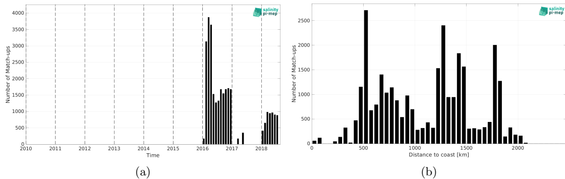
Figure 1: Number of match-ups between Surface drifters and SMOS SSS L3 v8 - 9 Days (CATDS-CEC-LOCEAN) SSS as a function of time (a) and as function of the distance to coast (b) over the Southern Ocean Pi-MEP region and for the full satellite product period.
