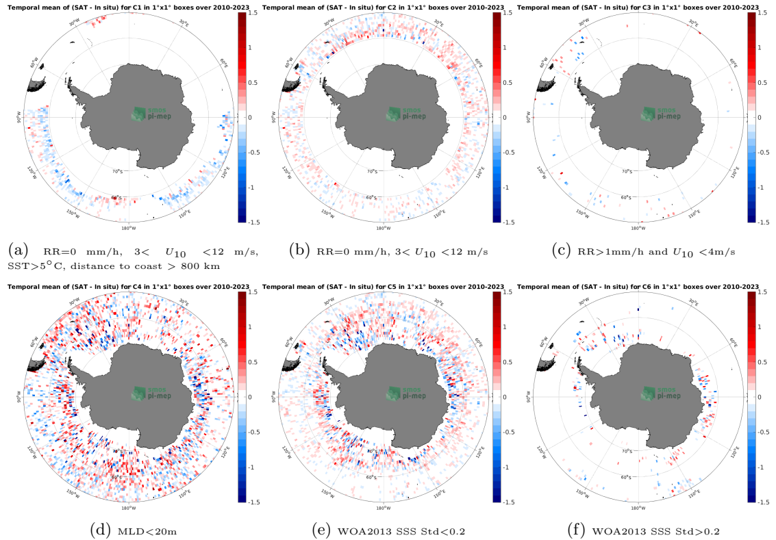
Figure 12: Temporal mean gridded over spatial boxes of size 1^{\circ}\times 1^{\circ} of \Delta\text{SSS} (SMOS SSS L3 v8 - 9 Days (CATDS-CECOS-LOCEAN) - Argo) for 6 different subdatasets corresponding to:RR=0 mm/h, 3 < U_{10} < 12 m/s, \text{SST} > 5^{\circ}\text{C} , distance to coast > 800 km (a), RR=0 mm/h, 3 < U_{10} < 12 m/s (b), RR >1\text{mm/h} and U_{10} < 4\text{m/s} (c),MLD <20\text{m} (d),WOA2013 SSS Std <0.2 (e),WOA2013 SSS Std >0.2 (f).
