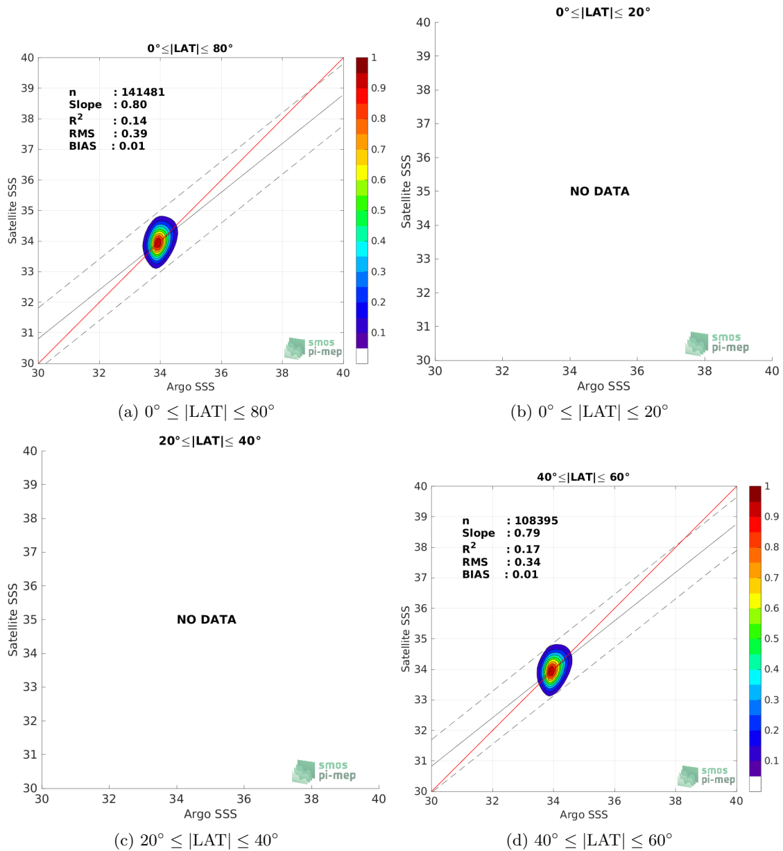
Figure 9: Contour maps of the concentration of SMOS SSS L3 v8 - 9 Days (CATDS-CECOS-LOCEAN) SSS (y-axis) versus Argo SSS (x-axis) at match-up pairs for different latitude bands. For each plot, the red line shows x=y . The black thin and dashed lines indicate a linear fit through the data cloud and the \pm 95\% confidence levels, respectively. The number match-up pairs n , the slope and R^2 coefficient of the linear fit, the root mean square (RMS) and the mean bias between satellite and in situ data are indicated for each latitude band in each plots.
