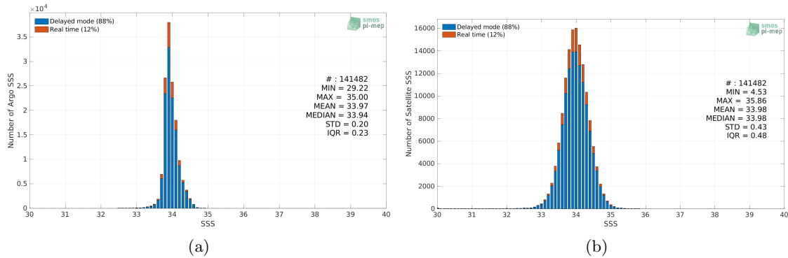
Figure 2: Histograms of SSS from Argo (a) and SMOS SSS L3 v8 - 9 Days (CATDS-CECOS-LOCEAN) (b) considering all match-up pairs per bins of 0.1 over the Southern Ocean Pi-MEP region and for the full satellite product period.
