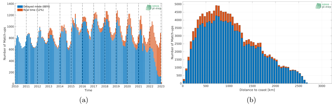
Figure 1: Number of match-ups between Argo and SMOS SSS L3 v8 - 9 Days (CATDS-CECOS-LOCEAN) SSS as a function of time (a) and as function of the distance to coast (b) over the Southern Ocean Pi-MEP region and for the full satellite product period.
