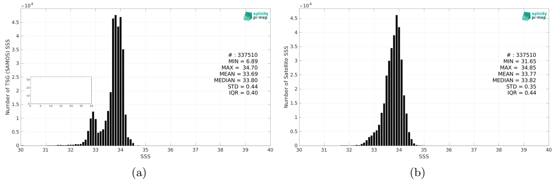
Figure 2: Histograms of SSS from TSG (SAMOS) (a) and SMOS SSS L3 v8 - 18 Days (CATDS-CEC-LOCEAN) (b) considering all match-up pairs per bins of 0.1 over the Southern Ocean Pi-MEP region and for the full satellite product period.
