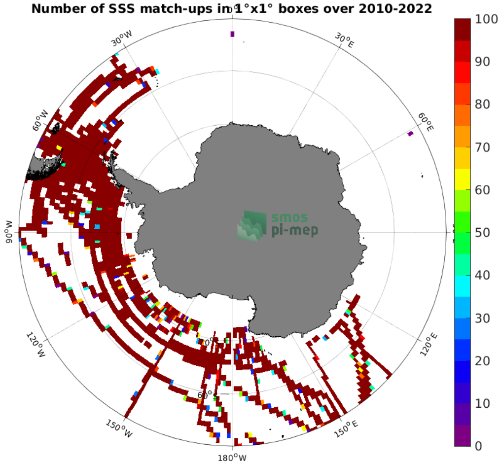
Figure 4: Number of SSS match-ups between TSG (SAMOS) SSS and the SMOS SSS L3 v8 - 18 Days (CATDS-CECOS-LOCEAN) SSS product for the Southern Ocean Pi-MEP region over 1^\circ \times 1^\circ boxes and for the full satellite product period.
