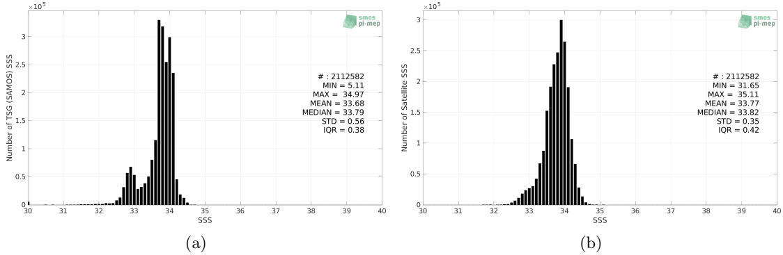
Figure 2: Histograms of SSS from TSG (SAMOS) (a) and SMOS SSS L3 v8 - 18 Days (CATDS-CECOS-LOCEAN) (b) considering all match-up pairs per bins of 0.1 over the Southern Ocean Pi-MEP region and for the full satellite product period.
