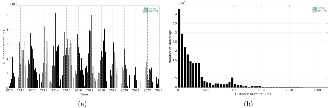
Figure 1: Number of match-ups between TSG (SAMOS) and SMOS SSS L3 v8 - 18 Days (CATDS-CECOS-LOCEAN) SSS as a function of time (a) and as function of the distance to coast (b) over the Southern Ocean Pi-MEP region and for the full satellite product period.
