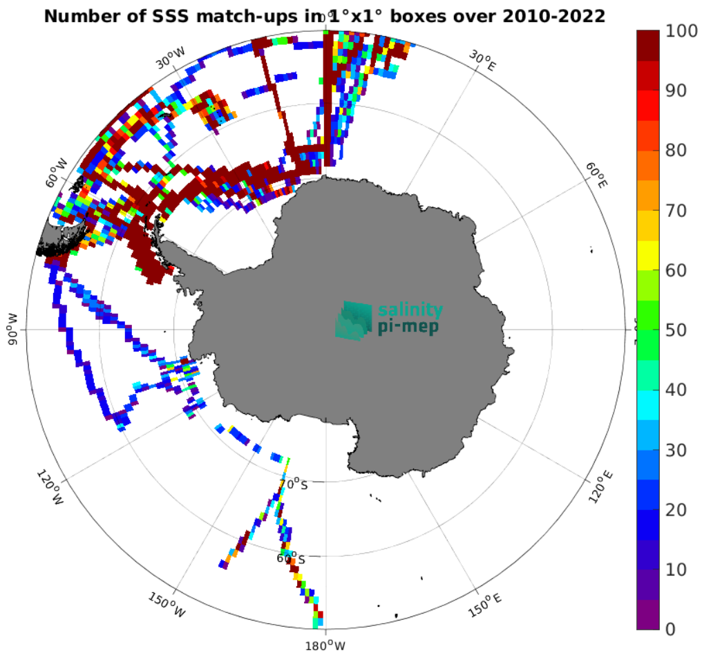
Figure 4: Number of SSS match-ups between TSG (Polarstern) SSS and the SMOS SSS L3 v8 - 18 Days (CATDS-CEC-LOCEAN) SSS product for the Southern Ocean Pi-MEP region over 1^\circ \times 1^\circ boxes and for the full satellite product period.
