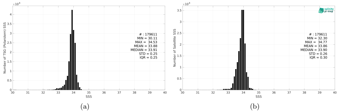
Figure 2: Histograms of SSS from TSG (Polarstern) (a) and SMOS SSS L3 v8 - 18 Days (CATDS-CEC-LOCEAN) (b) considering all match-up pairs per bins of 0.1 over the Southern Ocean Pi-MEP region and for the full satellite product period.
