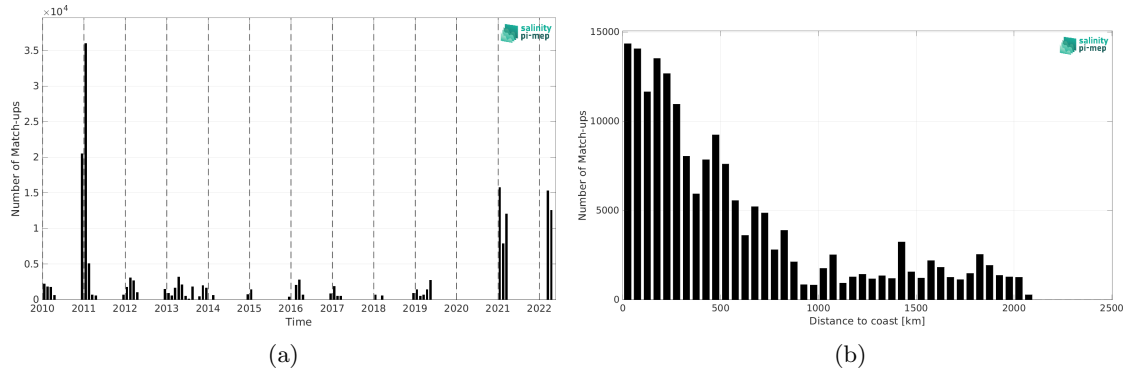
Figure 1: Number of match-ups between TSG (Polarstern) and SMOS SSS L3 v8 - 18 Days (CATDS-CEC-LOCEAN) SSS as a function of time (a) and as function of the distance to coast (b) over the Southern Ocean Pi-MEP region and for the full satellite product period.
