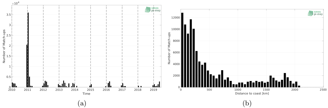
Figure 1: Number of match-ups between TSG (Polarstern) and SMOS SSS L3 v8 - 18 Days (CATDS-CECOS-LOCEAN) SSS as a function of time (a) and as function of the distance to coast (b) over the Southern Ocean Pi-MEP region and for the full satellite product period.
