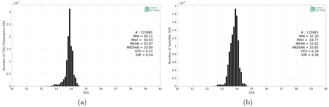
Figure 2: Histograms of SSS from TSG (Polarstern) (a) and SMOS SSS L3 v8 - 18 Days (CATDS-CECOS-LOCEAN) (b) considering all match-up pairs per bins of 0.1 over the Southern Ocean Pi-MEP region and for the full satellite product period.
