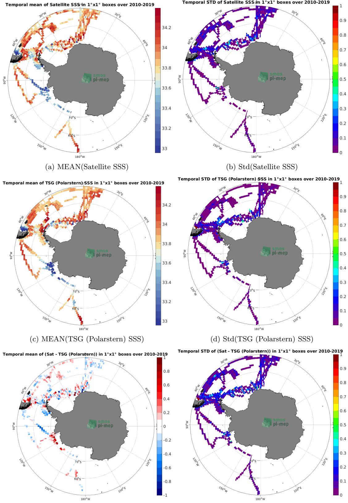
Figure 6: Temporal mean (left) and Std (right) of SSS from SMOS SSS L3 v8 - 18 Days (CATDS-CECOS-LOCEAN) (top), TSG (Polarstern) (middle), and of \Delta SSS (Satellite - TSG (Polarstern)). Only match-up pairs are used to generate these maps.
