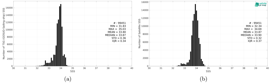
Figure 2: Histograms of SSS from TSG (GOSUD-Sailing-ship) (a) and SMOS SSS L3 v8 - 18 Days (CATDS-CEC-LOCEAN) (b) considering all match-up pairs per bins of 0.1 over the Southern Ocean Pi-MEP region and for the full satellite product period.
