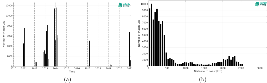
Figure 1: Number of match-ups between TSG (GOSUD-Sailing-ship) and SMOS SSS L3 v8 - 18 Days (CATDS-CEC-LOCEAN) SSS as a function of time (a) and as function of the distance to coast (b) over the Southern Ocean Pi-MEP region and for the full satellite product period.
