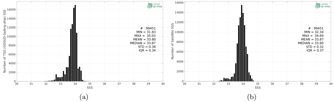
Figure 2: Histograms of SSS from TSG (GOSUD-Sailing-ship) (a) and SMOS SSS L3 v8 - 18 Days (CATDS-CECOS-LOCEAN) (b) considering all match-up pairs per bins of 0.1 over the Southern Ocean Pi-MEP region and for the full satellite product period.
