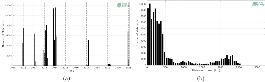
Figure 1: Number of match-ups between TSG (GOSUD-Sailing-ship) and SMOS SSS L3 v8 - 18 Days (CATDS-CECOS-LOCEAN) SSS as a function of time (a) and as function of the distance to coast (b) over the Southern Ocean Pi-MEP region and for the full satellite product period.
