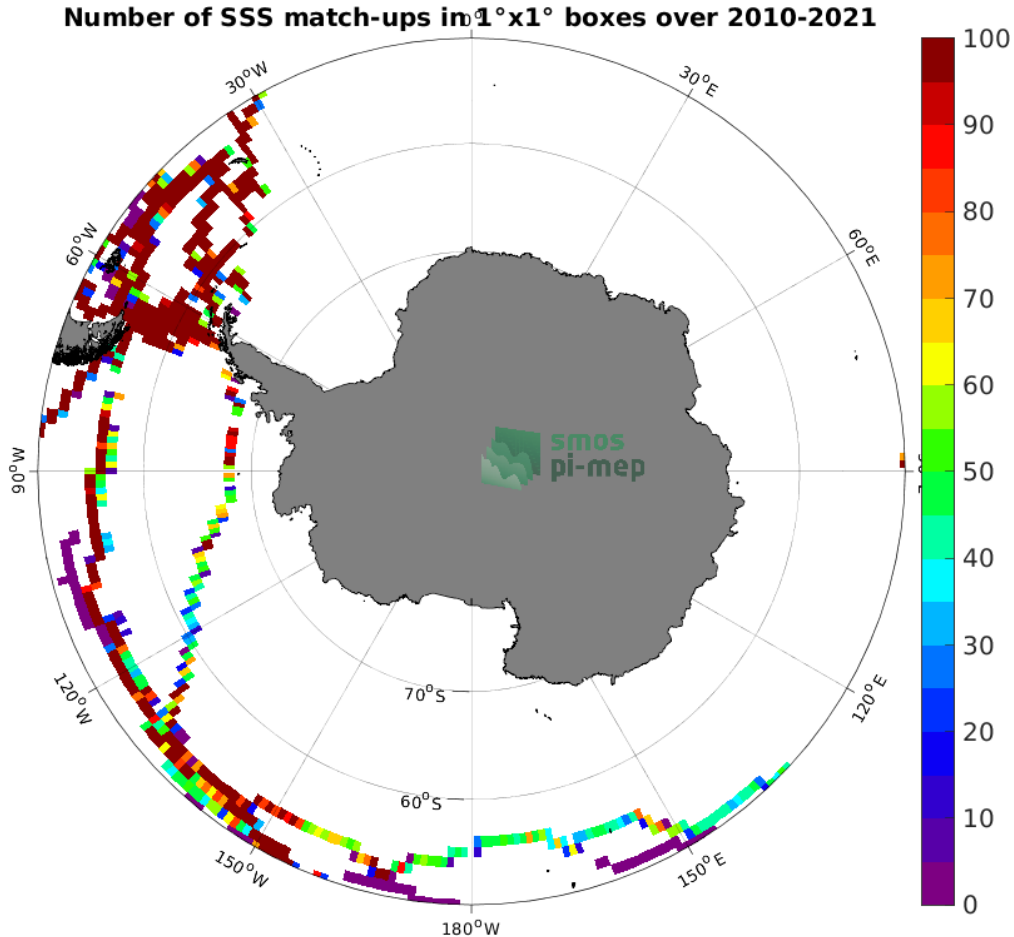
Figure 4: Number of SSS match-ups between TSG (GOSUD-Sailing-ship) SSS and the SMOS SSS L3 v8 - 18 Days (CATDS-CECOS-LOCEAN) SSS product for the Southern Ocean Pi-MEP region over 1^\circ \times 1^\circ boxes and for the full satellite product period.
