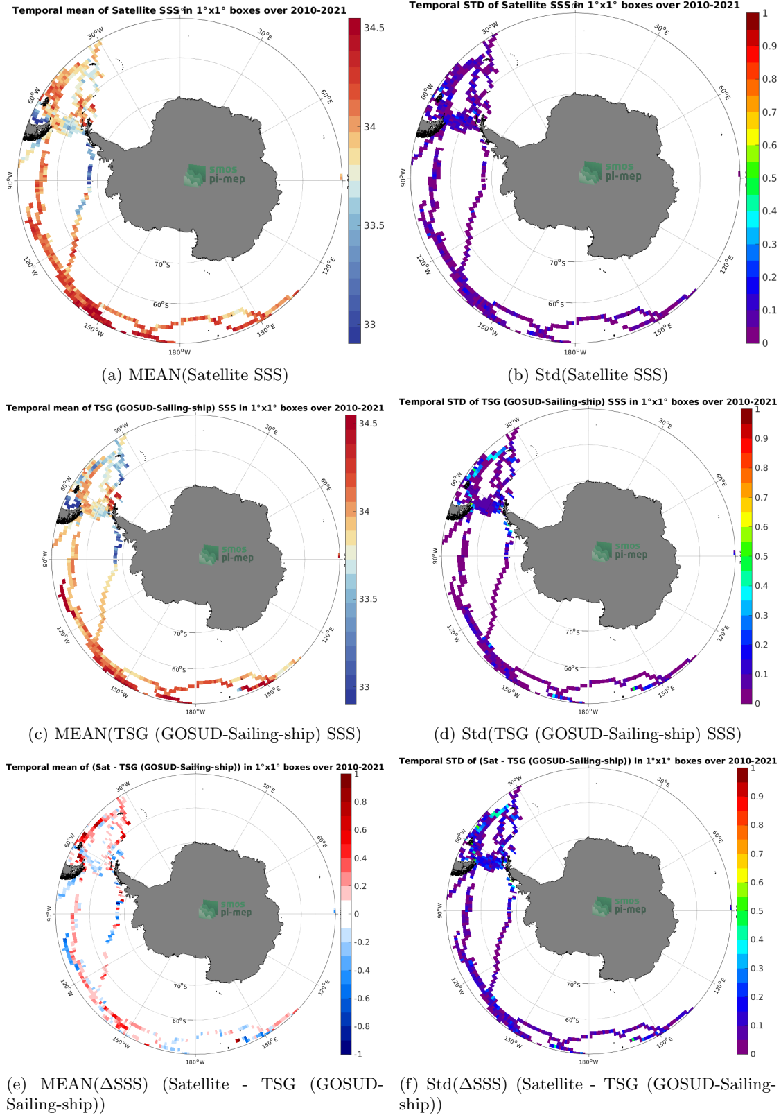
Figure 6: Temporal mean (left) and Std (right) of SSS from SMOS SSS L3 v8 - 18 Days (CATDS-CECOS-LOCEAN) (top), TSG (GOSUD-Sailing-ship) (middle), and of \Delta SSS (Satellite - TSG (GOSUD-Sailing-ship)). Only match-up pairs are used to generate these maps.
