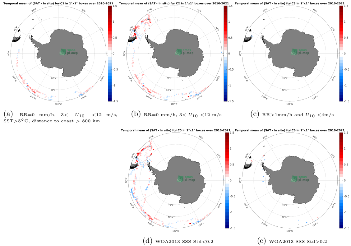
Figure 12: Temporal mean gridded over spatial boxes of size 1^\circ \times 1^\circ of \Delta SSS (SMOS SSS L3 v8 - 18 Days (CATDS-CECOS-LOCEAN) - TSG (GOSUD-Sailing-ship)) for 5 different subdatasets corresponding to:RR=0 mm/h, 3 < U_{10} < 12 m/s, SST>5°C, distance to coast > 800 km (a), RR=0 mm/h, 3 < U_{10} < 12 m/s (b), RR>1mm/h and U_{10} < 4 m/s (c), WOA2013 SSS Std<0.2 (d), WOA2013 SSS Std>0.2 (e).
