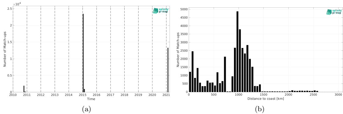
Figure 1: Number of match-ups between TSG (GOSUD-Research-vessel) and SMOS SSS L3 v8 - 18 Days (CATDS-CEC-LOCEAN) SSS as a function of time (a) and as function of the distance to coast (b) over the Southern Ocean Pi-MEP region and for the full satellite product period.
