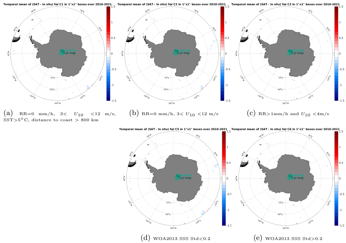
Figure 12: Temporal mean gridded over spatial boxes of size 1^\circ \times 1^\circ of \Delta\text{SSS} (SMOS SSS L3 v8 - 18 Days (CATDS-CEC-LOCEAN) - TSG (GOSUD-Research-vessel)) for 5 different subdatasets corresponding to: RR=0 mm/h, 3 < U_{10} < 12 m/s, SST > 5^\circ\text{C} , distance to coast > 800 km (a), RR=0 mm/h, 3 < U_{10} < 12 m/s (b), RR > 1 mm/h and U_{10} < 4 m/s (c), WOA2013 SSS Std < 0.2 (d), WOA2013 SSS Std > 0.2 (e).
