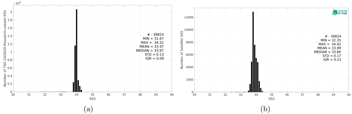
Figure 2: Histograms of SSS from TSG (GOSUD-Research-vessel) (a) and SMOS SSS L3 v8 - 18 Days (CATDS-CEC-LOCEAN) (b) considering all match-up pairs per bins of 0.1 over the Southern Ocean Pi-MEP region and for the full satellite product period.
