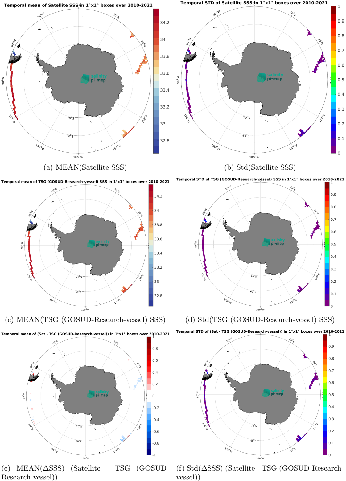
Figure 6: Temporal mean (left) and Std (right) of SSS from SMOS SSS L3 v8 - 18 Days (CATDS-CEC-LOCEAN) (top), TSG (GOSUD-Research-vessel) (middle), and of \Delta SSS (Satellite - TSG (GOSUD-Research-vessel)). Only match-up pairs are used to generate these maps.
