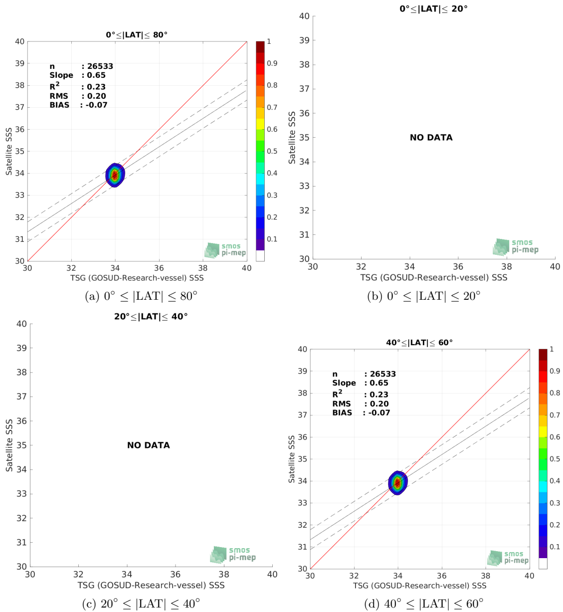
Figure 9: Contour maps of the concentration of SMOS SSS L3 v8 - 18 Days (CATDS-CECOS-LOCEAN) SSS (y-axis) versus TSG (GOSUD-Research-vessel) SSS (x-axis) at match-up pairs for different latitude bands. For each plot, the red line shows x=y . The black thin and dashed lines indicate a linear fit through the data cloud and the \pm 95\% confidence levels, respectively. The number match-up pairs n , the slope and R^2 coefficient of the linear fit, the root mean square (RMS) and the mean bias between satellite and in situ data are indicated for each latitude band in each plots.
