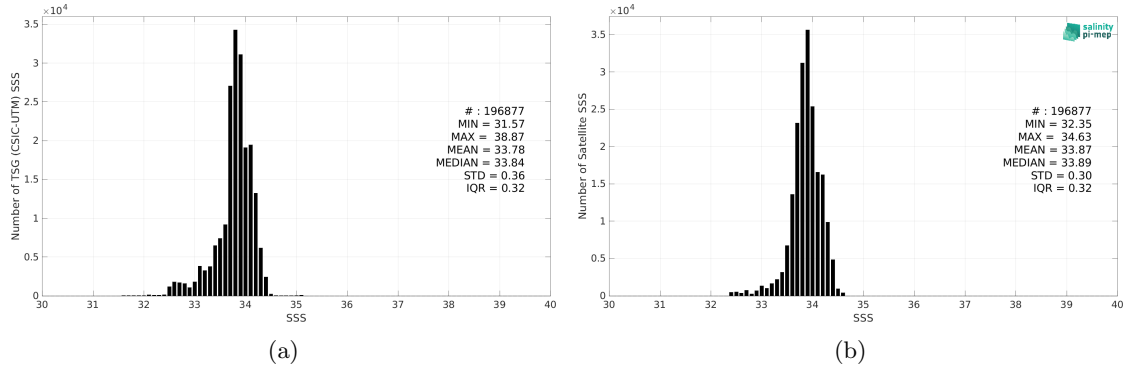
Figure 2: Histograms of SSS from TSG (CSIC-UTM) (a) and SMOS SSS L3 v8 - 18 Days (CATDS-CEC-LOCEAN) (b) considering all match-up pairs per bins of 0.1 over the Southern Ocean Pi-MEP region and for the full satellite product period.
