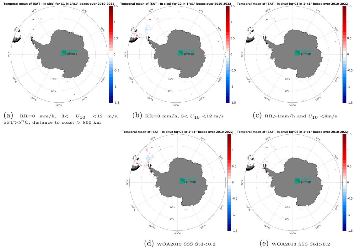
Figure 12: Temporal mean gridded over spatial boxes of size 1^{\circ}\times 1^{\circ} of \Delta\text{SSS} (SMOS SSS L3 v8 - 18 Days (CATDS-CEC-LOCEAN) - TSG (CSIC-UTM)) for 5 different subdatasets corresponding to:RR=0 mm/h, 3 < U_{10} < 12 m/s, SST >5^{\circ}\text{C} , distance to coast > 800 km (a), RR=0 mm/h, 3 < U_{10} < 12 m/s (b), RR >1 mm/h and U_{10} < 4 m/s (c), WOA2013 SSS Std <0.2 (d), WOA2013 SSS Std >0.2 (e).
