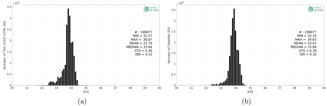
Figure 2: Histograms of SSS from TSG (CSIC-UTM) (a) and SMOS SSS L3 v8 - 18 Days (CATDS-CECOS-LOCEAN) (b) considering all match-up pairs per bins of 0.1 over the Southern Ocean Pi-MEP region and for the full satellite product period.
