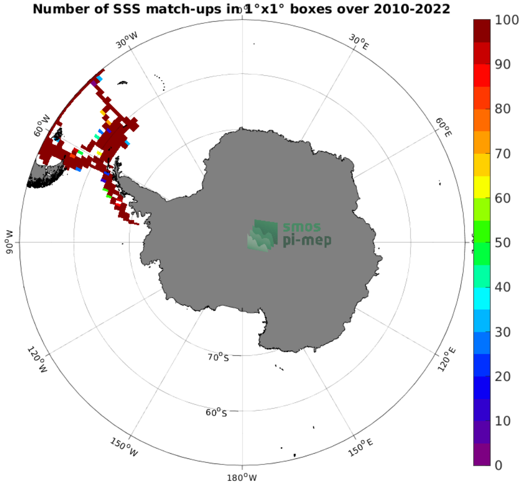
Figure 4: Number of SSS match-ups between TSG (CSIC-UTM) SSS and the SMOS SSS L3 v8 - 18 Days (CATDS-CECOS-LOCEAN) SSS product for the Southern Ocean Pi-MEP region over 1^\circ \times 1^\circ boxes and for the full satellite product period.
