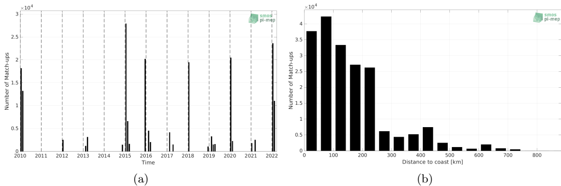
Figure 1: Number of match-ups between TSG (CSIC-UTM) and SMOS SSS L3 v8 - 18 Days (CATDS-CECOS-LOCEAN) SSS as a function of time (a) and as function of the distance to coast (b) over the Southern Ocean Pi-MEP region and for the full satellite product period.
