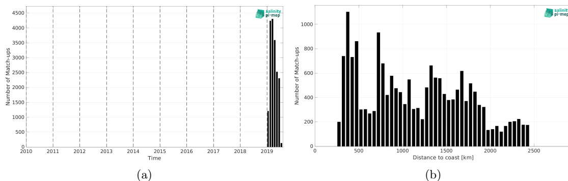
Figure 1: Number of match-ups between Saildrone and SMOS SSS L3 v8 - 18 Days (CATDS-CEC-LOCEAN) SSS as a function of time (a) and as function of the distance to coast (b) over the Southern Ocean Pi-MEP region and for the full satellite product period.
