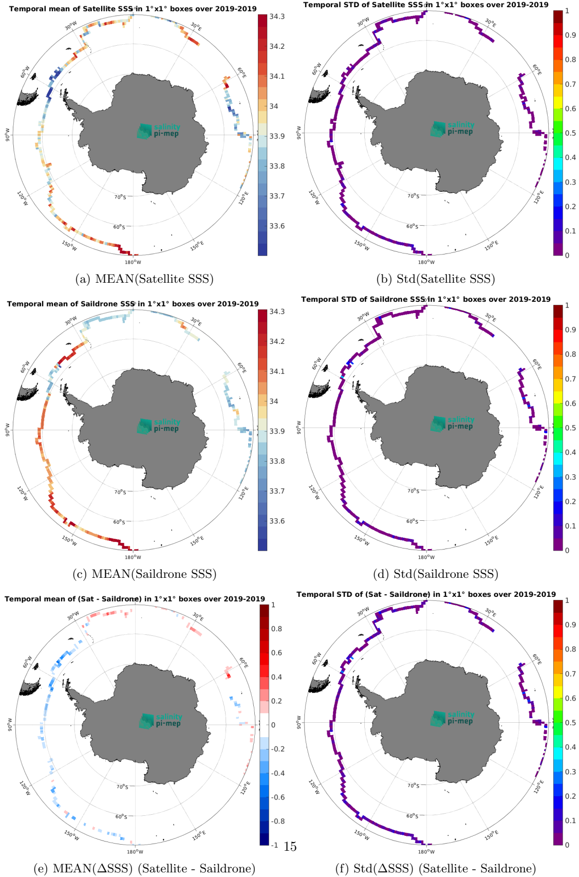
Figure 6: Temporal mean (left) and Std (right) of SSS from SMOS SSS L3 v8 - 18 Days (CATDS-CEC-LOCEAN) (top), Saildrone (middle), and of \Delta SSS (Satellite - Saildrone). Only match-up pairs are used to generate these maps.
