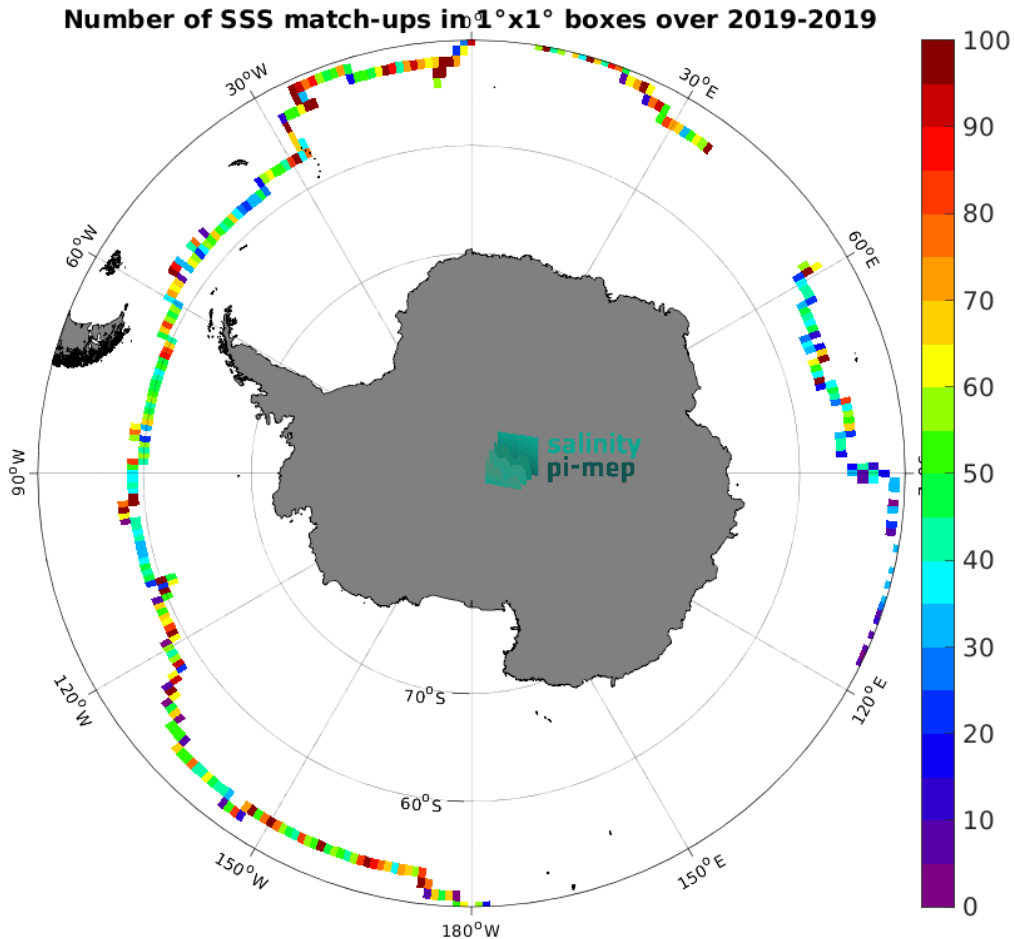
Figure 4: Number of SSS match-ups between Sairdrone SSS and the SMOS SSS L3 v8 - 18 Days (CATDS-CEC-LOCEAN) SSS product for the Southern Ocean Pi-MEP region over 1^\circ \times 1^\circ boxes and for the full satellite product period.
