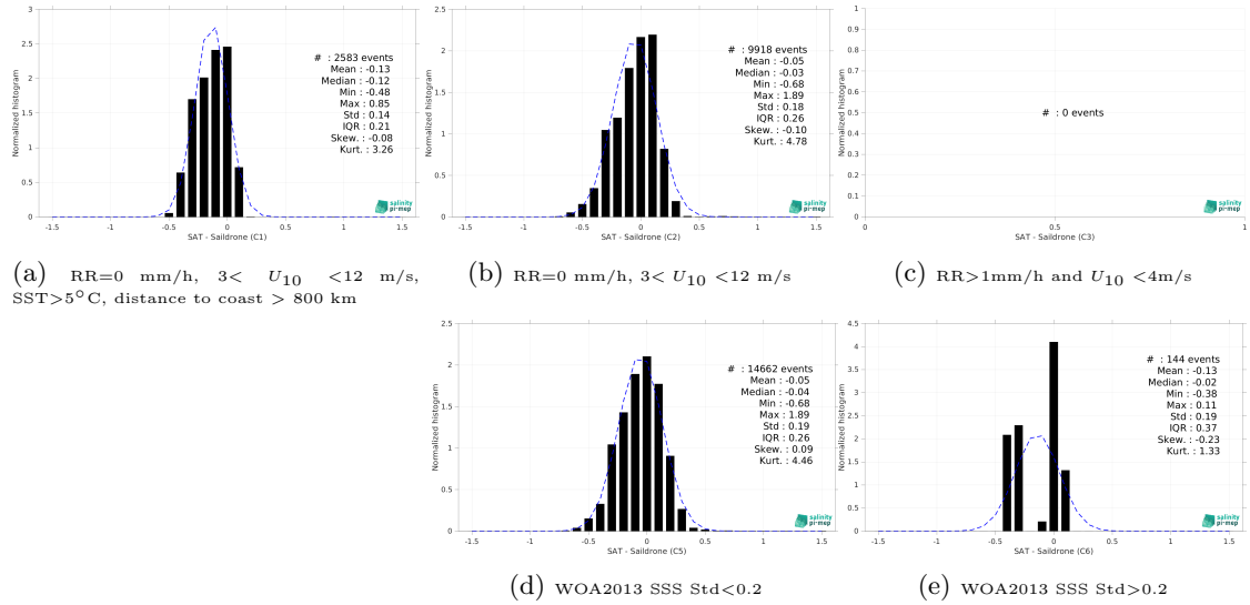
Figure 13: Normalized histogram of \Delta SSS (SMOS SSS L3 v8 - 18 Days (CATDS-CEC-LOCEAN) - Saildrone) for 5 different subdatasets corresponding to: RR=0 mm/h, 3 < U_{10} < 12 m/s, SST > 5°C, distance to coast > 800 km (a), RR=0 mm/h, 3 < U_{10} < 12 m/s (b), RR > 1mm/h and U_{10} < 4 m/s (c), WOA2013 SSS Std < 0.2 (d), WOA2013 SSS Std > 0.2 (e).
