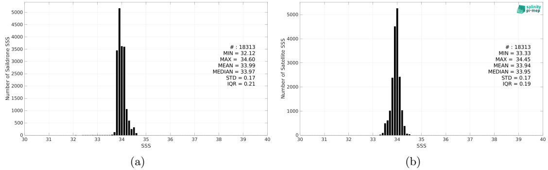
Figure 2: Histograms of SSS from Sairdrone (a) and SMOS SSS L3 v8 - 18 Days (CATDS-CEC-LOCEAN) (b) considering all match-up pairs per bins of 0.1 over the Southern Ocean Pi-MEP region and for the full satellite product period.
