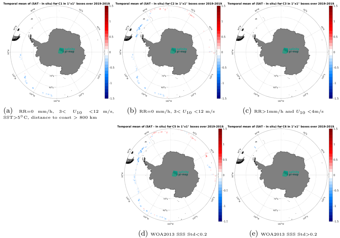
Figure 12: Temporal mean gridded over spatial boxes of size 1^{\circ}\times 1^{\circ} of \Delta\text{SSS} (SMOS SSS L3 v8 - 18 Days (CATDS-CEC-LOCEAN) - Saildrone) for 5 different subdatasets corresponding to:RR=0 mm/h, 3 < U_{10} < 12 m/s, SST >5^{\circ}\text{C} , distance to coast > 800 km (a), RR=0 mm/h, 3 < U_{10} < 12 m/s (b), RR >1 mm/h and U_{10} < 4 m/s (c), WOA2013 SSS Std <0.2 (d), WOA2013 SSS Std >0.2 (e).
