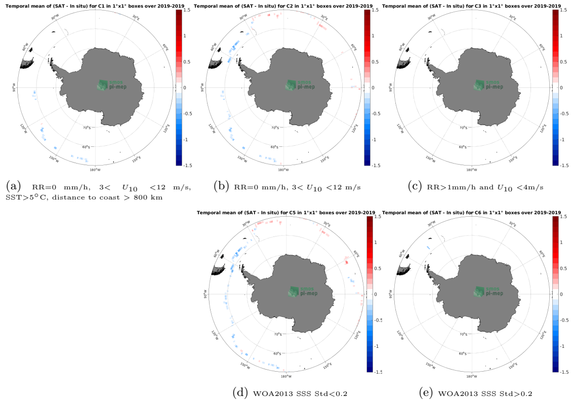
Figure 12: Temporal mean gridded over spatial boxes of size 1^{\circ}\times 1^{\circ} of \Delta\text{SSS} (SMOS SSS L3 v8 - 18 Days (CATDS-CECOS-LOCEAN) - Saildrone) for 5 different subdatasets corresponding to:RR=0 mm/h, 3 < U_{10} < 12 m/s, SST >5^{\circ}\text{C} , distance to coast > 800 km (a), RR=0 mm/h, 3 < U_{10} < 12 m/s (b), RR >1 mm/h and U_{10} < 4 m/s (c), WOA2013 SSS Std <0.2 (d), WOA2013 SSS Std >0.2 (e).
