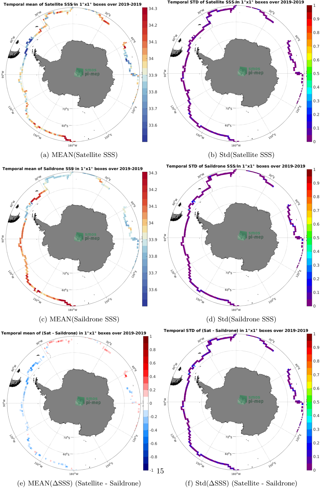
Figure 6: Temporal mean (left) and Std (right) of SSS from SMOS SSS L3 v8 - 18 Days (CATDS-CECOS-LOCEAN) (top), Saildrone (middle), and of \Delta SSS (Satellite - Saildrone). Only match-up pairs are used to generate these maps.
