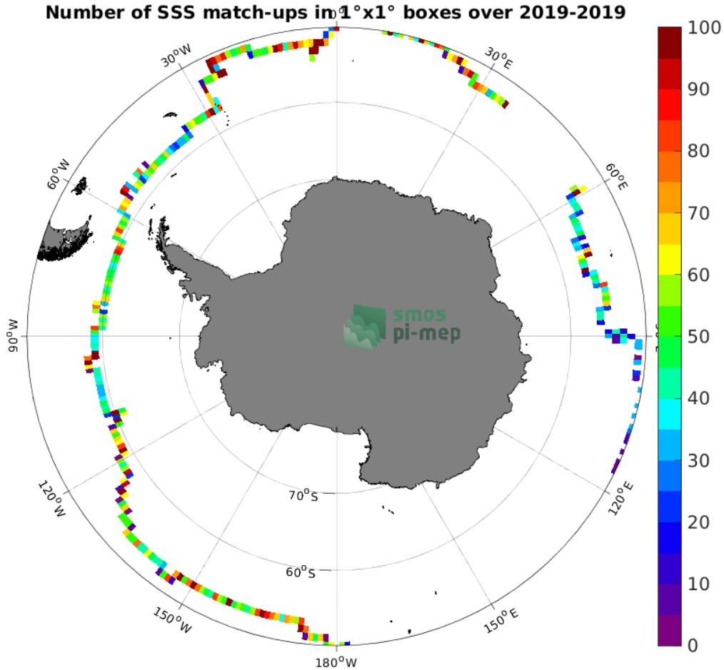
Figure 4: Number of SSS match-ups between Saildrone SSS and the SMOS SSS L3 v8 - 18 Days (CATDS-CECOS-LOCEAN) SSS product for the Southern Ocean Pi-MEP region over 1^\circ \times 1^\circ boxes and for the full satellite product period.
