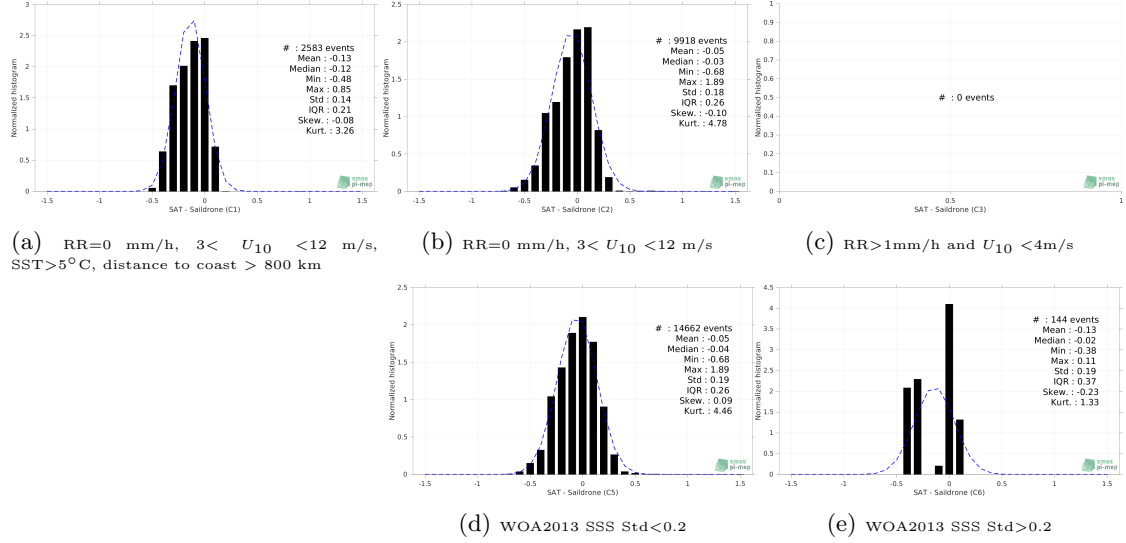
Figure 13: Normalized histogram of \Delta SSS (SMOS SSS L3 v8 - 18 Days (CATDS-CECOS-LOCEAN) - Saildrone) for 5 different subdatasets corresponding to: RR=0 mm/h, 3 < U_{10} < 12 m/s, SST > 5°C, distance to coast > 800 km (a), RR=0 mm/h, 3 < U_{10} < 12 m/s (b), RR > 1mm/h and U_{10} < 4 m/s (c), WOA2013 SSS Std < 0.2 (d), WOA2013 SSS Std > 0.2 (e).
