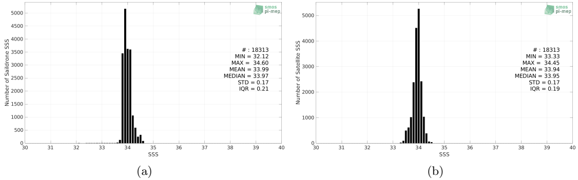
Figure 2: Histograms of SSS from Saildrone (a) and SMOS SSS L3 v8 - 18 Days (CATDS-CECOS-LOCEAN) (b) considering all match-up pairs per bins of 0.1 over the Southern Ocean Pi-MEP region and for the full satellite product period.
