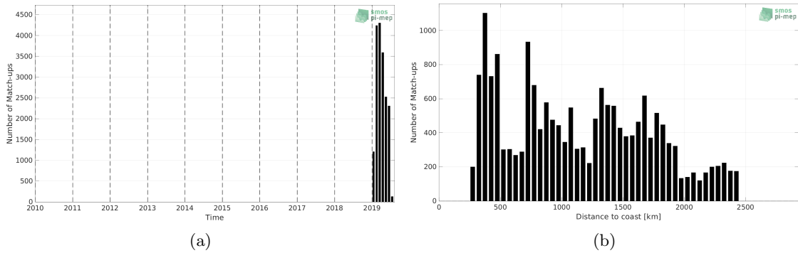
Figure 1: Number of match-ups between Saildrone and SMOS SSS L3 v8 - 18 Days (CATDS-CECOS-LOCEAN) SSS as a function of time (a) and as function of the distance to coast (b) over the Southern Ocean Pi-MEP region and for the full satellite product period.
