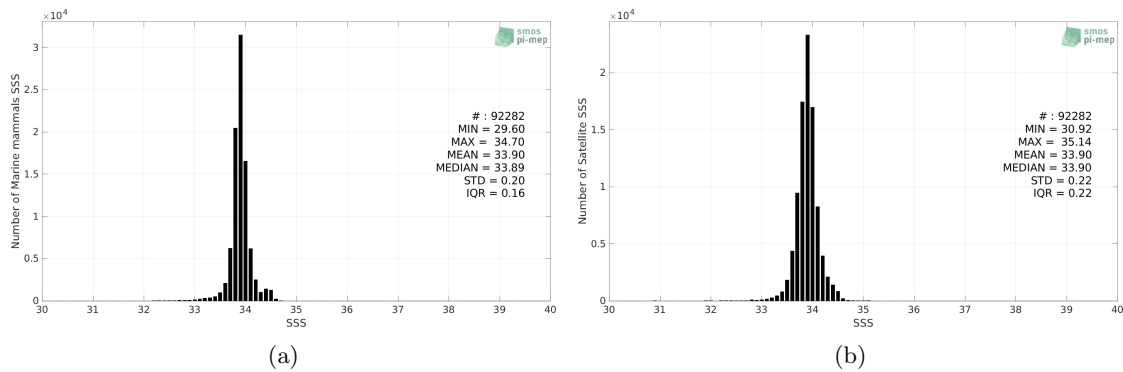
Figure 2: Histograms of SSS from Marine mammals (a) and SMOS SSS L3 v8 - 18 Days (CATDS-CECOS-LOCEAN) (b) considering all match-up pairs per bins of 0.1 over the Southern Ocean Pi-MEP region and for the full satellite product period.
