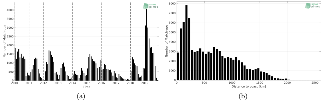
Figure 1: Number of match-ups between Marine mammals and SMOS SSS L3 v8 - 18 Days (CATDS-CECOS-LOCEAN) SSS as a function of time (a) and as function of the distance to coast (b) over the Southern Ocean Pi-MEP region and for the full satellite product period.
