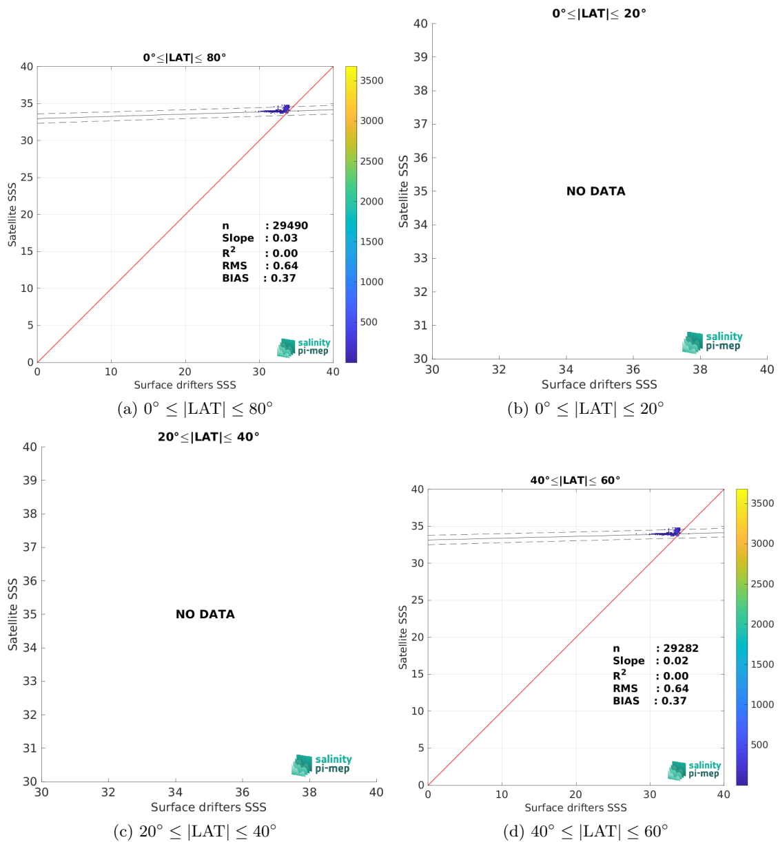
Figure 8: Contour maps of the concentration of SMOS SSS L3 v8 - 18 Days (CATDS-CEC-LOCEAN) SSS (y-axis) versus Surface drifters SSS (x-axis) at match-up pairs for different latitude bands. For each plot, the red line shows x=y . The black thin and dashed lines indicate a linear fit through the data cloud and the \pm 95\% confidence levels, respectively. The number match-up pairs n , the slope and R^2 coefficient of the linear fit, the root mean square (RMS) and the mean bias between satellite and in situ data are indicated for each latitude band in each plots.
