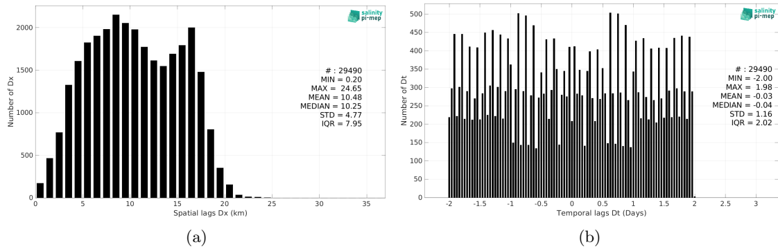
Figure 4: Histograms of the spatial (a) and temporal (b) lags between the location/time of the Surface drifters measurement and the date of the corresponding SMOS SSS L3 v8 - 18 Days (CATDS-CEC-LOCEAN) SSS pixel.
