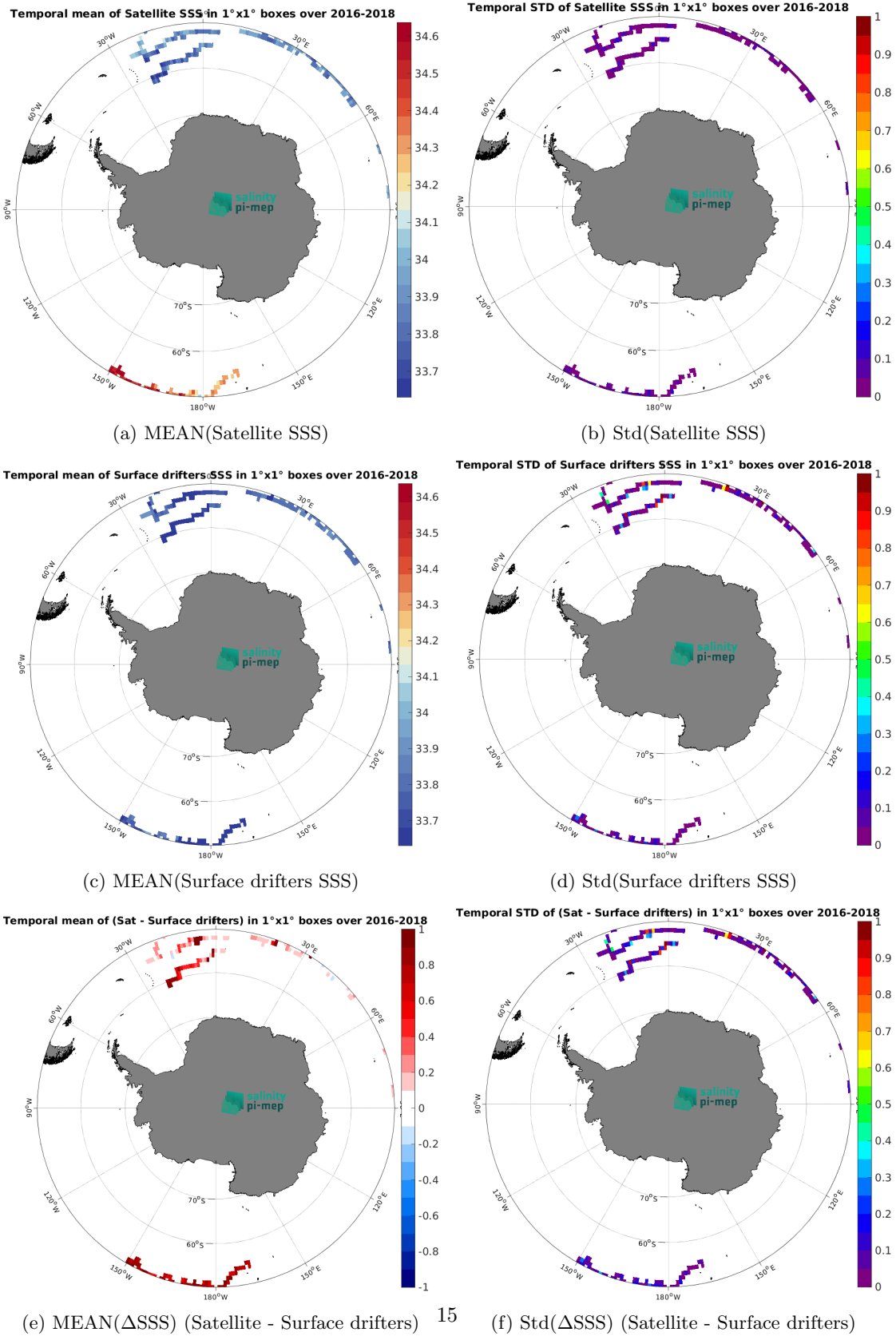
Figure 5: Temporal mean (left) and Std (right) of SSS from SMOS SSS L3 v8 - 18 Days (CATDS-CEC-LOCEAN) (top), Surface drifters (middle), and of \Delta SSS (Satellite - Surface drifters). Only match-up pairs are used to generate these maps.
