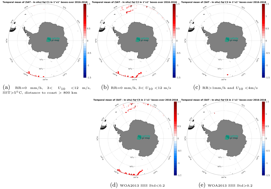
Figure 11: Temporal mean gridded over spatial boxes of size 1^{\circ}\times 1^{\circ} of \Delta\text{SSS} (SMOS SSS L3 v8 - 18 Days (CATDS-CEC-LOCEAN) - Surface drifters) for 5 different subdatasets corresponding to: RR=0 mm/h, 3 < U_{10} < 12 m/s, SST >5^{\circ}\text{C} , distance to coast > 800 km (a), RR=0 mm/h, 3 < U_{10} < 12 m/s (b), RR >1 mm/h and U_{10} < 4 m/s (c), WOA2013 SSS Std <0.2 (d), WOA2013 SSS Std >0.2 (e).
