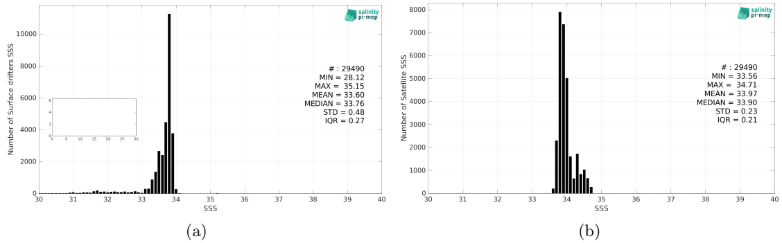
Figure 2: Histograms of SSS from Surface drifters (a) and SMOS SSS L3 v8 - 18 Days (CATDS-CEC-LOCEAN) (b) considering all match-up pairs per bins of 0.1 over the Southern Ocean Pi-MEP region and for the full satellite product period.
