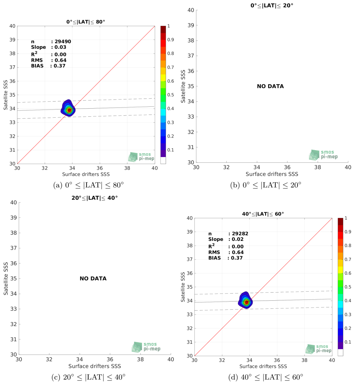
Figure 8: Contour maps of the concentration of SMOS SSS L3 v8 - 18 Days (CATDS-CECOS-LOCEAN) SSS (y-axis) versus Surface drifters SSS (x-axis) at match-up pairs for different latitude bands. For each plot, the red line shows x=y . The black thin and dashed lines indicate a linear fit through the data cloud and the \pm 95\% confidence levels, respectively. The number match-up pairs n , the slope and R^2 coefficient of the linear fit, the root mean square (RMS) and the mean bias between satellite and in situ data are indicated for each latitude band in each plots.
