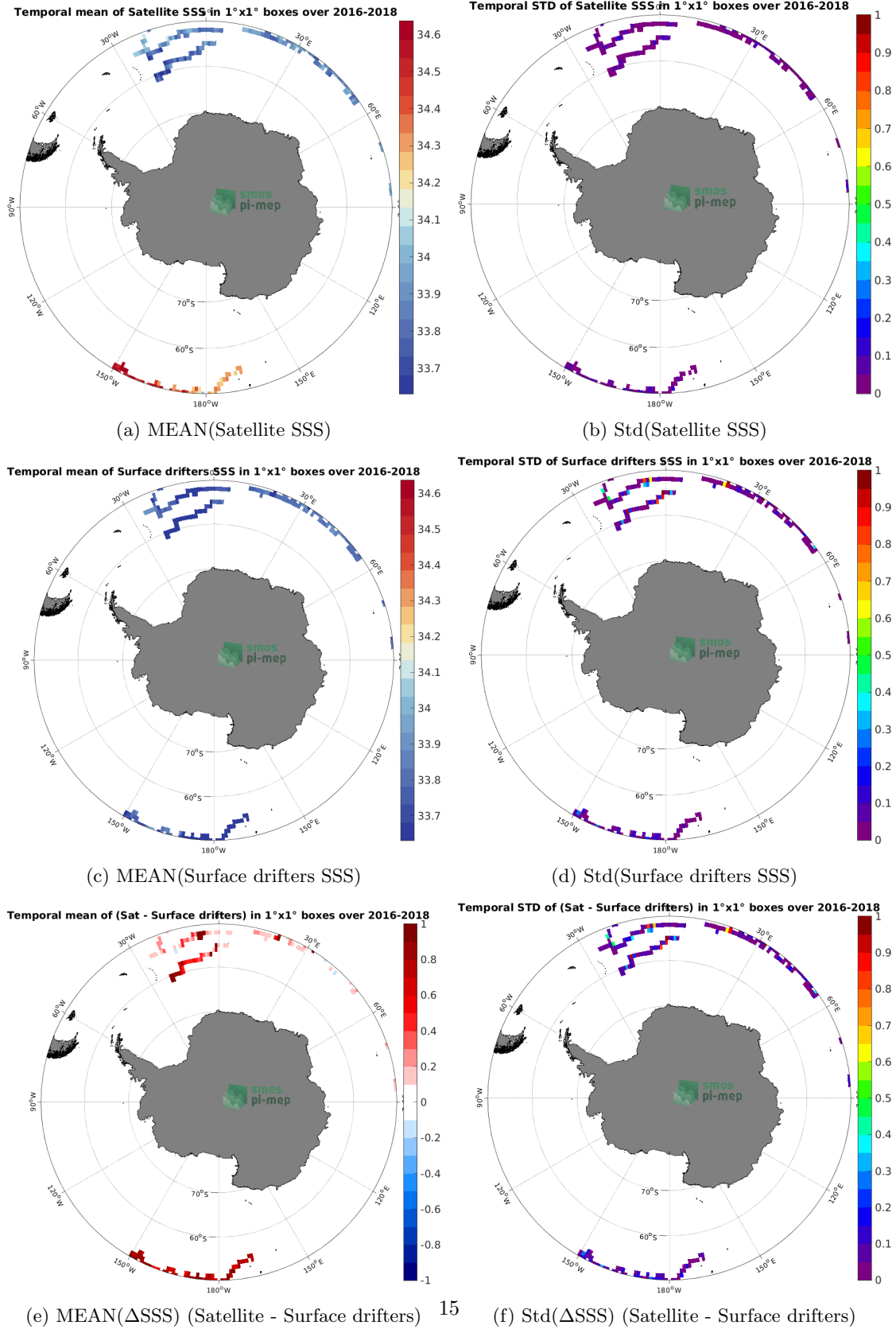
Figure 5: Temporal mean (left) and Std (right) of SSS from SMOS SSS L3 v8 - 18 Days (CATDS-CECOS-LOCEAN) (top), Surface drifters (middle), and of \Delta SSS (Satellite - Surface drifters). Only match-up pairs are used to generate these maps.
