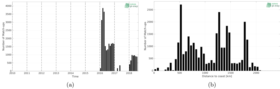
Figure 1: Number of match-ups between Surface drifters and SMOS SSS L3 v8 - 18 Days (CATDS-CECOS-LOCEAN) SSS as a function of time (a) and as function of the distance to coast (b) over the Southern Ocean Pi-MEP region and for the full satellite product period.
