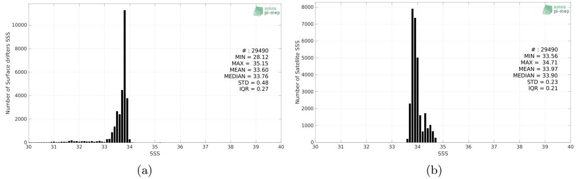
Figure 2: Histograms of SSS from Surface drifters (a) and SMOS SSS L3 v8 - 18 Days (CATDS-CECOS-LOCEAN) (b) considering all match-up pairs per bins of 0.1 over the Southern Ocean Pi-MEP region and for the full satellite product period.
