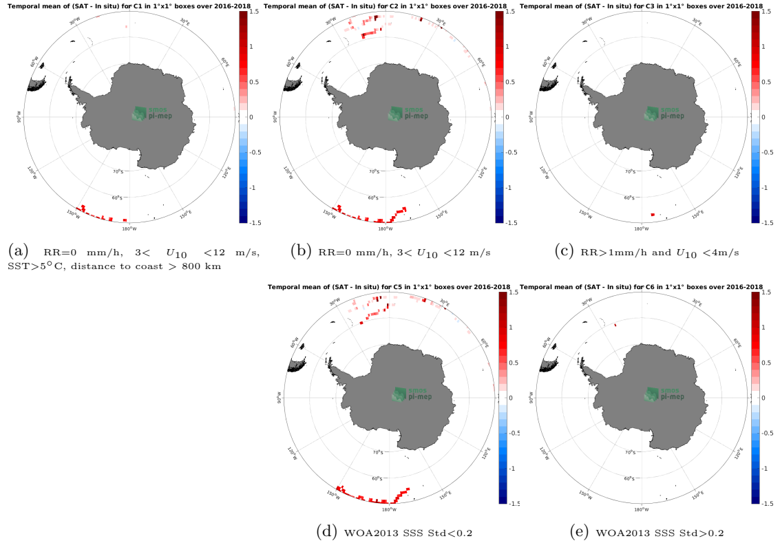
Figure 11: Temporal mean gridded over spatial boxes of size 1^{\circ}\times 1^{\circ} of \Delta\text{SSS} (SMOS SSS L3 v8 - 18 Days (CATDS-CECOS-LOCEAN) - Surface drifters) for 5 different subdatasets corresponding to:RR=0 mm/h, 3 < U_{10} < 12 m/s, SST >5^{\circ}\text{C} , distance to coast > 800 km (a), RR=0 mm/h, 3 < U_{10} < 12 m/s (b), RR >1 mm/h and U_{10} < 4 m/s (c), WOA2013 SSS Std <0.2 (d), WOA2013 SSS Std >0.2 (e).
