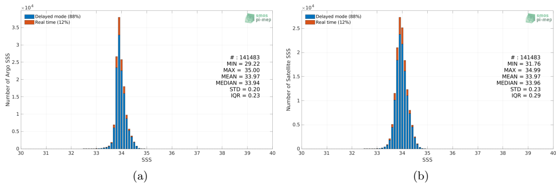
Figure 2: Histograms of SSS from Argo (a) and SMOS SSS L3 v8 - 18 Days (CATDS-CECOS-LOCEAN) (b) considering all match-up pairs per bins of 0.1 over the Southern Ocean Pi-MEP region and for the full satellite product period.
