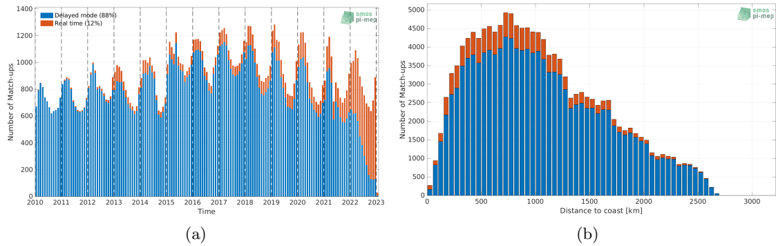
Figure 1: Number of match-ups between Argo and SMOS SSS L3 v8 - 18 Days (CATDS-CECOS-LOCEAN) SSS as a function of time (a) and as function of the distance to coast (b) over the Southern Ocean Pi-MEP region and for the full satellite product period.
