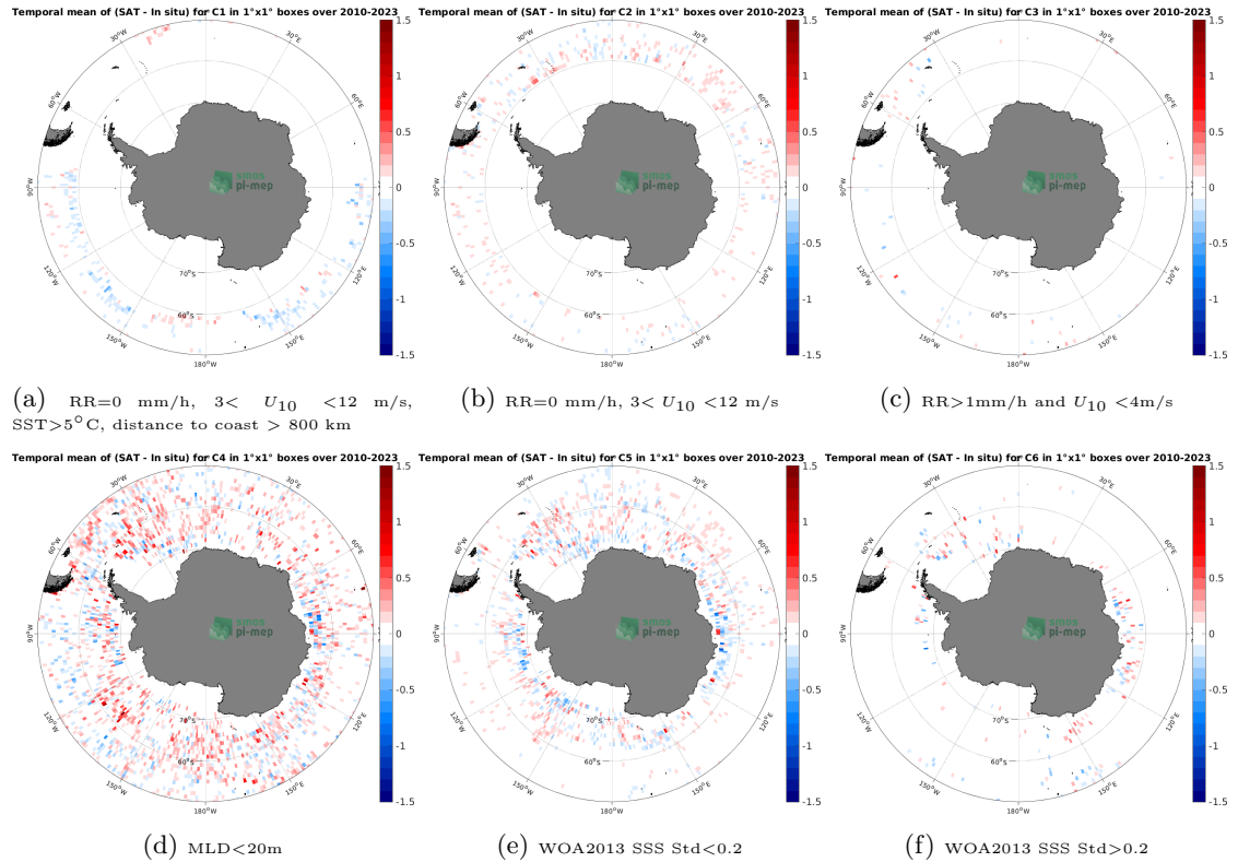
Figure 12: Temporal mean gridded over spatial boxes of size 1^{\circ}\times 1^{\circ} of \Delta\text{SSS} (SMOS SSS L3 v8 - 18 Days (CATDS-CECOS-LOCEAN) - Argo) for 6 different subdatasets corresponding to: \text{RR}=0 mm/h, 3 < U_{10} < 12 m/s, \text{SST} > 5^{\circ}\text{C} , distance to coast > 800 km (a), \text{RR}=0 mm/h, 3 < U_{10} < 12 m/s (b), \text{RR} > 1\text{mm/h} and U_{10} < 4\text{m/s} (c), \text{MLD} < 20\text{m} (d), \text{WOA2013 SSS Std} < 0.2 (e), \text{WOA2013 SSS Std} > 0.2 (f).
