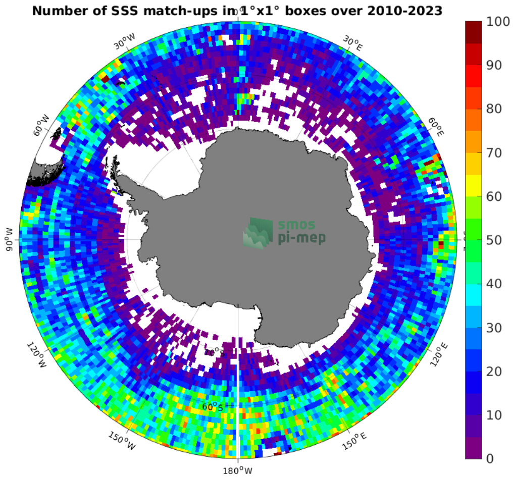
Figure 4: Number of SSS match-ups between Argo SSS and the SMOS SSS L3 v8 - 18 Days (CATDS-CECOS-LOCEAN) SSS product for the Southern Ocean Pi-MEP region over 1^\circ \times 1^\circ boxes and for the full satellite product period.
