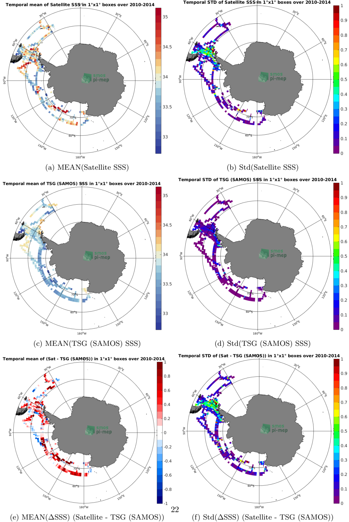
Figure 6: Temporal mean (left) and Std (right) of SSS from SMOS SSS L3 v7 - 9 Days (CATDS-CECOS-LOCEAN) (top), TSG (SAMOS) (middle), and of \Delta SSS (Satellite - TSG (SAMOS)). Only match-up pairs are used to generate these maps.
