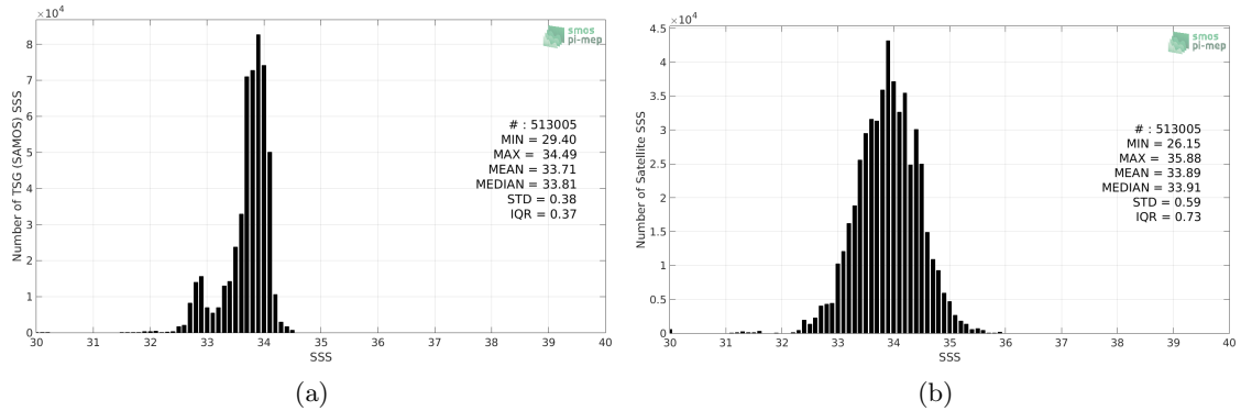
Figure 2: Histograms of SSS from TSG (SAMOS) (a) and SMOS SSS L3 v7 - 9 Days (CATDS-CECOS-LOCEAN) (b) considering all match-up pairs per bins of 0.1 over the Southern Ocean Pi-MEP region and for the full satellite product period.
