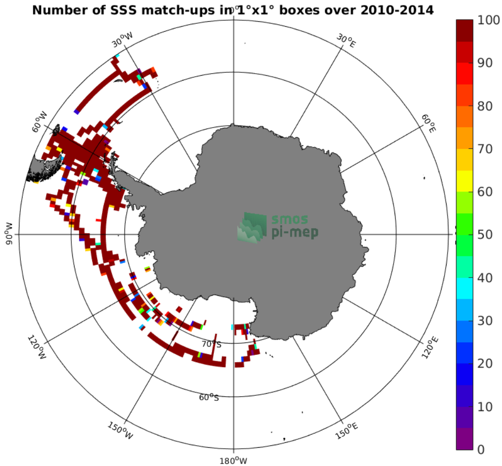
Figure 4: Number of SSS match-ups between TSG (SAMOS) SSS and the SMOS SSS L3 v7 - 9 Days (CATDS-CECOS-LOCEAN) SSS product for the Southern Ocean Pi-MEP region over 1^\circ \times 1^\circ boxes and for the full satellite product period.
