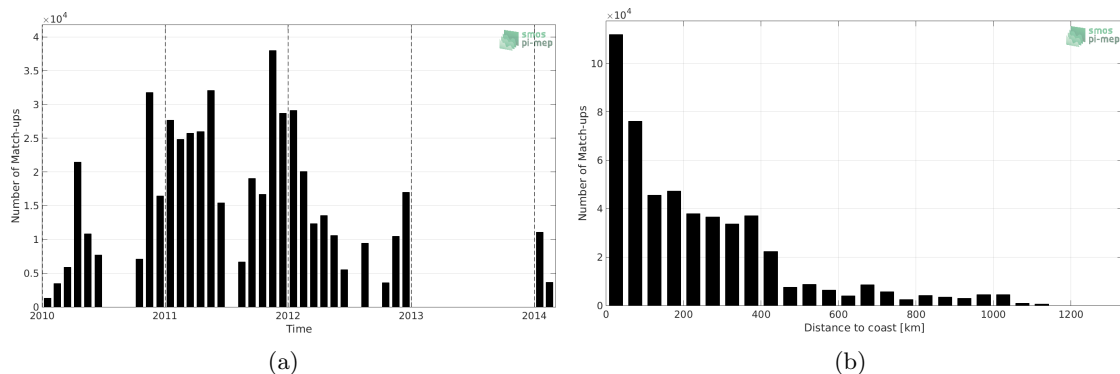
Figure 1: Number of match-ups between TSG (SAMOS) and SMOS SSS L3 v7 - 9 Days (CATDS-CECOS-LOCEAN) SSS as a function of time (a) and as function of the distance to coast (b) over the Southern Ocean Pi-MEP region and for the full satellite product period.
