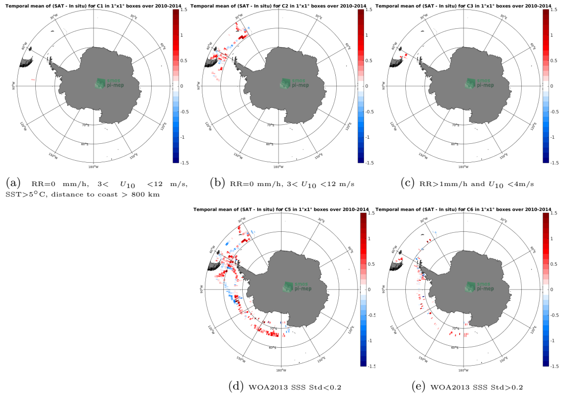
Figure 12: Temporal mean gridded over spatial boxes of size 1^{\circ}\times 1^{\circ} of \Delta\text{SSS} (SMOS SSS L3 v7 - 9 Days (CATDS-CECOS-LOCEAN) - TSG (SAMOS)) for 5 different subdatasets corresponding to:RR=0 mm/h, 3 < U_{10} < 12 m/s, SST >5^{\circ}\text{C} , distance to coast > 800 km (a), RR=0 mm/h, 3 < U_{10} < 12 m/s (b), RR >1 mm/h and U_{10} < 4 m/s (c), WOA2013 SSS Std <0.2 (d), WOA2013 SSS Std >0.2 (e).
