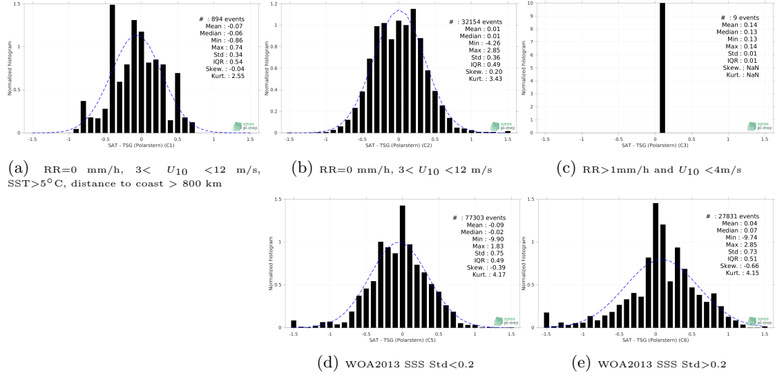
Figure 13: Normalized histogram of \Delta SSS (SMOS SSS L3 v7 - 9 Days (CATDS-CECOS-LOCEAN) - TSG (Polarstern)) for 5 different subdatasets corresponding to: RR=0 mm/h, 3 < U_{10} < 12 m/s, SST > 5°C, distance to coast > 800 km (a), RR=0 mm/h, 3 < U_{10} < 12 m/s (b), RR > 1mm/h and U_{10} < 4 m/s (c), WOA2013 SSS Std < 0.2 (d), WOA2013 SSS Std > 0.2 (e).
