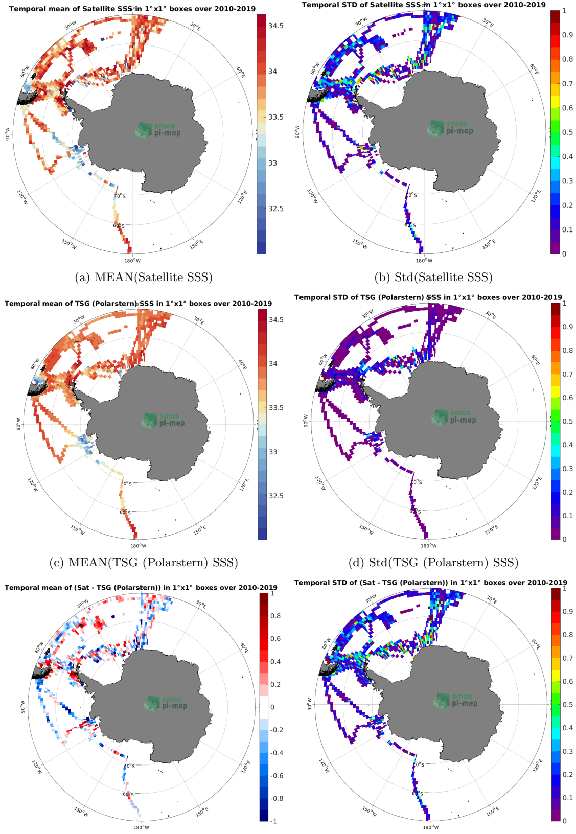
Figure 6: Temporal mean (left) and Std (right) of SSS from SMOS SSS L3 v7 - 9 Days (CATDS-CECOS-LOCEAN) (top), TSG (Polarstern) (middle), and of \Delta SSS (Satellite - TSG (Polarstern)). Only match-up pairs are used to generate these maps.
