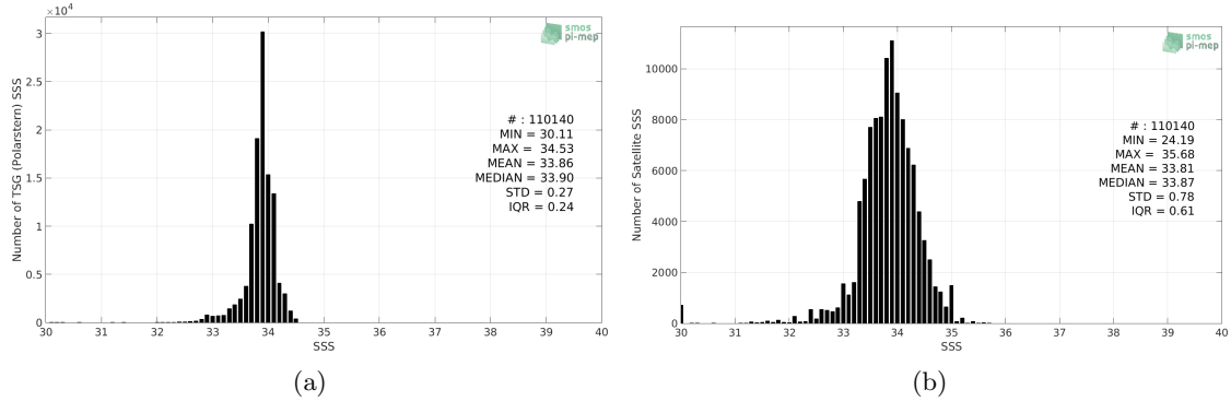
Figure 2: Histograms of SSS from TSG (Polarstern) (a) and SMOS SSS L3 v7 - 9 Days (CATDS-CECOS-LOCEAN) (b) considering all match-up pairs per bins of 0.1 over the Southern Ocean Pi-MEP region and for the full satellite product period.
