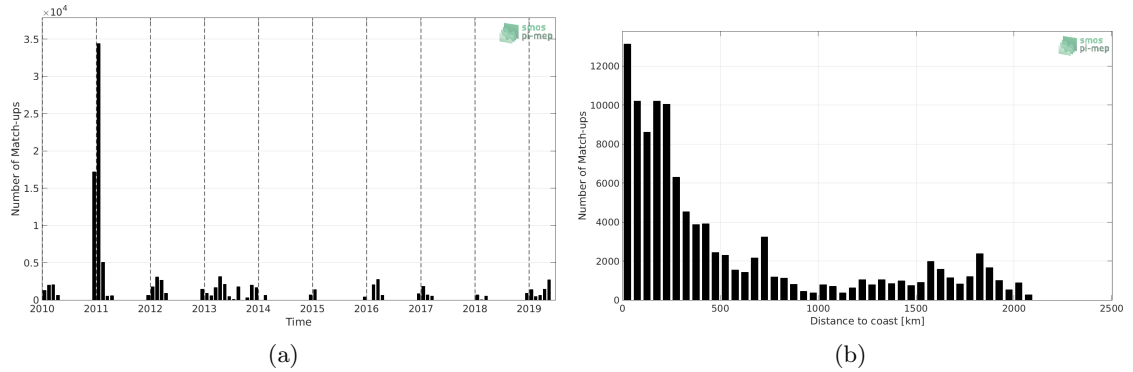
Figure 1: Number of match-ups between TSG (Polarstern) and SMOS SSS L3 v7 - 9 Days (CATDS-CECOS-LOCEAN) SSS as a function of time (a) and as function of the distance to coast (b) over the Southern Ocean Pi-MEP region and for the full satellite product period.
