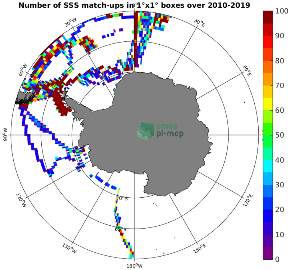
Figure 4: Number of SSS match-ups between TSG (Polarstern) SSS and the SMOS SSS L3 v7 - 9 Days (CATDS-CECOS-LOCEAN) SSS product for the Southern Ocean Pi-MEP region over 1^\circ \times 1^\circ boxes and for the full satellite product period.
