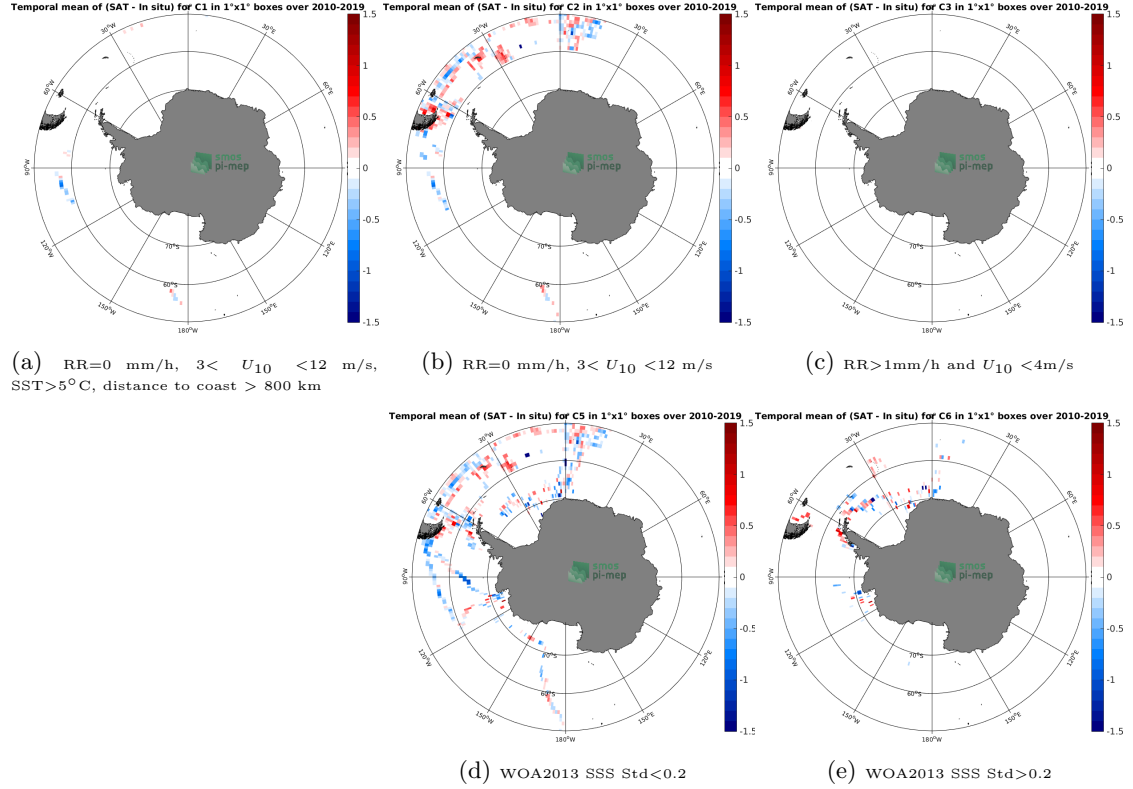
Figure 12: Temporal mean gridded over spatial boxes of size 1^{\circ} \times 1^{\circ} of \Delta\text{SSS} (SMOS SSS L3 v7 - 9 Days (CATDS-CECOS-LOCEAN) - TSG (Polarstern)) for 5 different subdatasets corresponding to: RR=0 mm/h, 3 < U_{10} < 12 m/s, SST > 5^{\circ}\text{C} , distance to coast > 800 km (a), RR=0 mm/h, 3 < U_{10} < 12 m/s (b), RR > 1 mm/h and U_{10} < 4 m/s (c), WOA2013 SSS Std < 0.2 (d), WOA2013 SSS Std > 0.2 (e).
