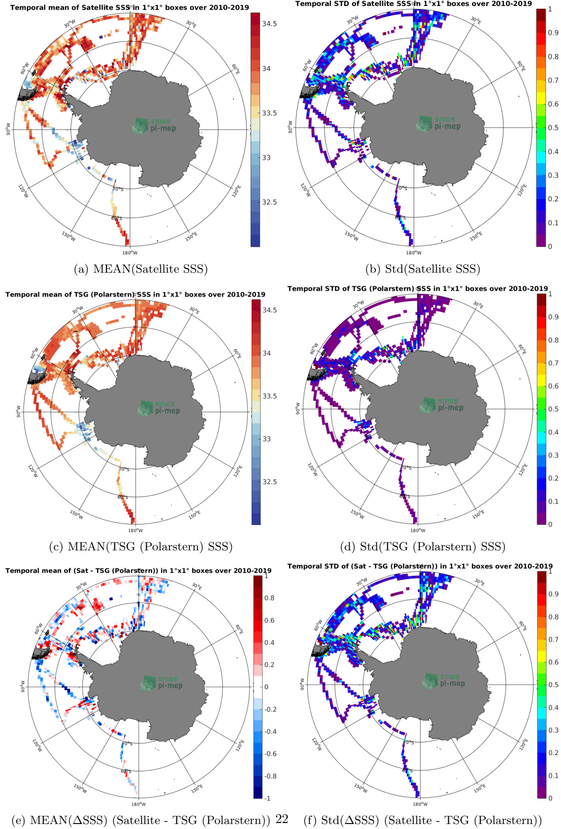
Figure 6: Temporal mean (left) and Std (right) of SSS from SMOS SSS L3 v7 - 9 Days (CATDS-CECOS-LOCEAN) (top), TSG (Polarstern) (middle), and of \Delta SSS (Satellite - TSG (Polarstern)). Only match-up pairs are used to generate these maps.
