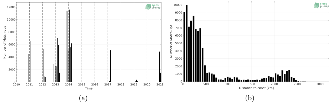
Figure 1: Number of match-ups between TSG (GOSUD-Sailing-ship) and SMOS SSS L3 v7 - 9 Days (CATDS-CECOS-LOCEAN) SSS as a function of time (a) and as function of the distance to coast (b) over the Southern Ocean Pi-MEP region and for the full satellite product period.
