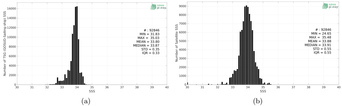
Figure 2: Histograms of SSS from TSG (GOSUD-Sailing-ship) (a) and SMOS SSS L3 v7 - 9 Days (CATDS-CECOS-LOCEAN) (b) considering all match-up pairs per bins of 0.1 over the Southern Ocean Pi-MEP region and for the full satellite product period.
