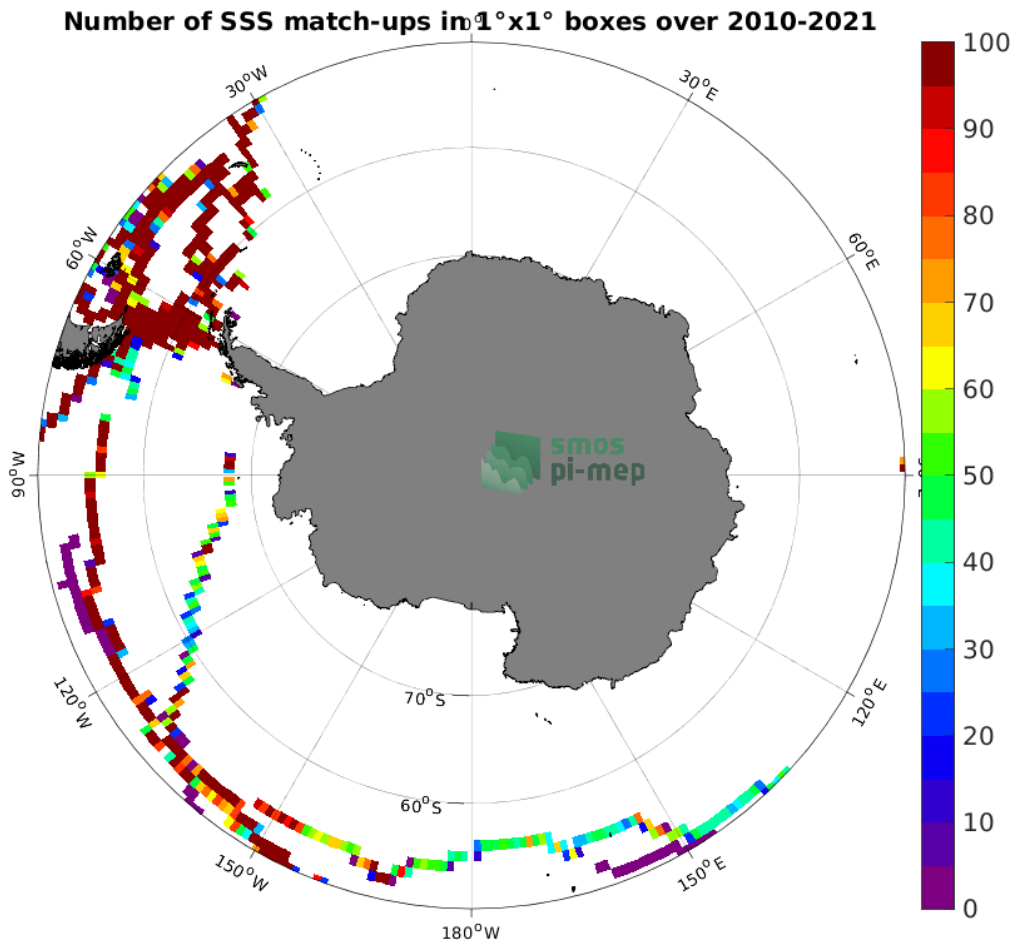
Figure 4: Number of SSS match-ups between TSG (GOSUD-Sailing-ship) SSS and the SMOS SSS L3 v7 - 9 Days (CATDS-CECOS-LOCEAN) SSS product for the Southern Ocean Pi-MEP region over 1^\circ \times 1^\circ boxes and for the full satellite product period.
