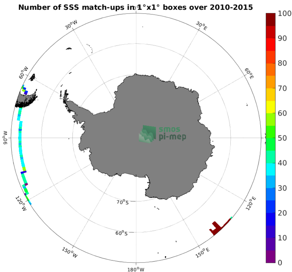
Figure 4: Number of SSS match-ups between TSG (GOSUD-Research-vessel) SSS and the SMOS SSS L3 v7 - 9 Days (CATDS-CECOS-LOCEAN) SSS product for the Southern Ocean Pi-MEP region over 1^{\circ} \times 1^{\circ} boxes and for the full satellite product period.
