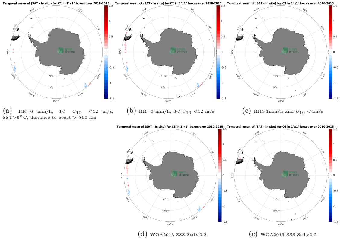
Figure 12: Temporal mean gridded over spatial boxes of size 1°x1° of \Delta SSS (SMOS SSS L3 v7 - 9 Days (CATDS-CECOS-LOCEAN) - TSG (GOSUD-Research-vessel)) for 5 different subdatasets corresponding to:RR=0 mm/h, 3 < U_{10} < 12 m/s, SST>5°C, distance to coast > 800 km (a), RR=0 mm/h, 3 < U_{10} < 12 m/s (b), RR>1mm/h and U_{10} < 4 m/s (c), WOA2013 SSS Std<0.2 (d), WOA2013 SSS Std>0.2 (e).
