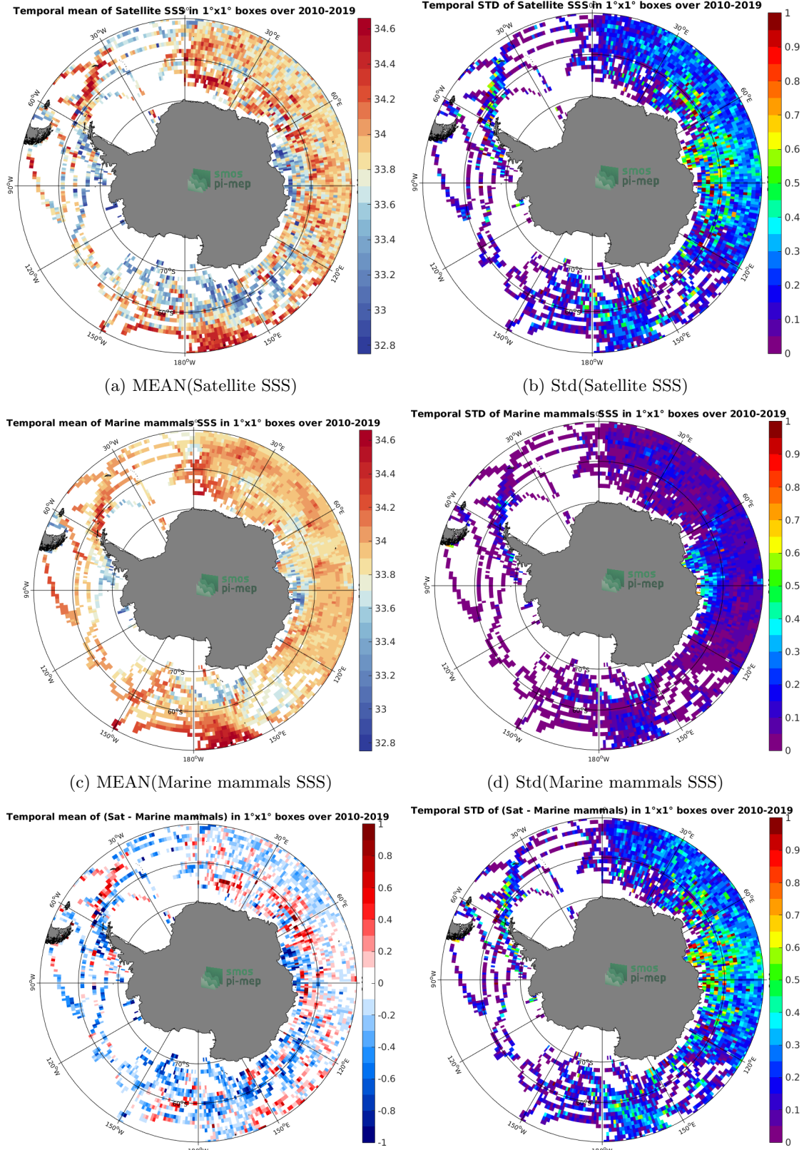
Figure 6: Temporal mean (left) and Std (right) of SSS from SMOS SSS L3 v7 - 9 Days (CATDS-CECOS-LOCEAN) (top), Marine mammals (middle), and of \Delta SSS (Satellite - Marine mammals). Only match-up pairs are used to generate these maps.
