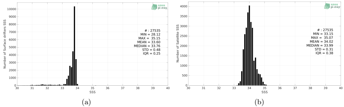
Figure 2: Histograms of SSS from Surface drifters (a) and SMOS SSS L3 v7 - 9 Days (CATDS-CECOS-LOCEAN) (b) considering all match-up pairs per bins of 0.1 over the Southern Ocean Pi-MEP region and for the full satellite product period.
