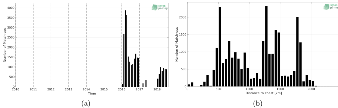
Figure 1: Number of match-ups between Surface drifters and SMOS SSS L3 v7 - 9 Days (CATDS-CECOS-LOCEAN) SSS as a function of time (a) and as function of the distance to coast (b) over the Southern Ocean Pi-MEP region and for the full satellite product period.
