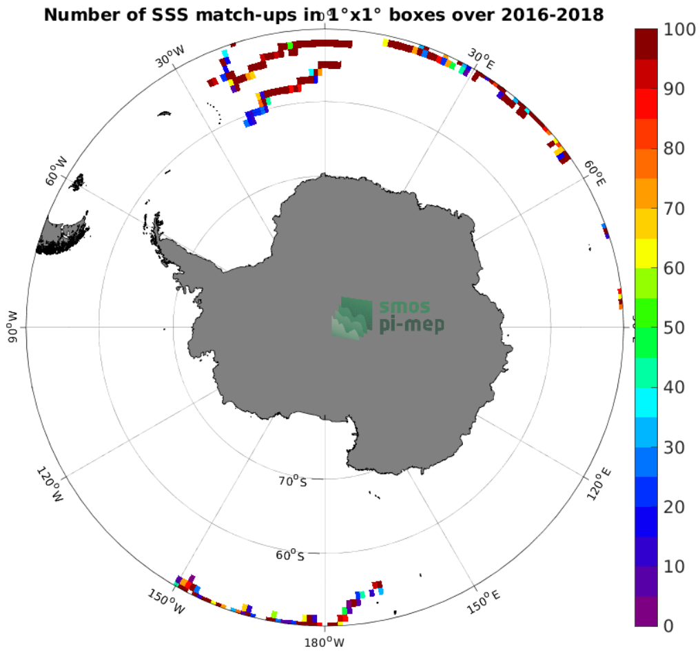
Figure 3: Number of SSS match-ups between Surface drifters SSS and the SMOS SSS L3 v7 - 9 Days (CATDS-CECOS-LOCEAN) SSS product for the Southern Ocean Pi-MEP region over 1^\circ \times 1^\circ boxes and for the full satellite product period.
